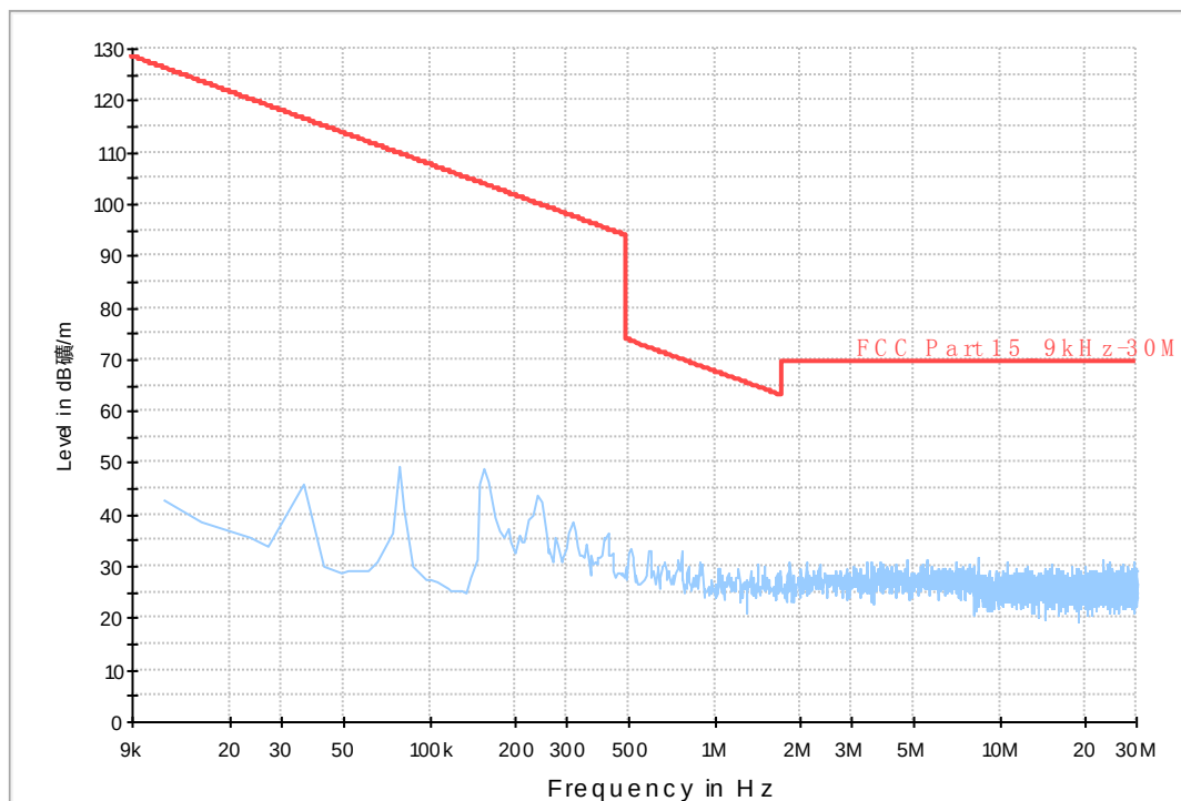
Fig. 127 Radiated Spurious Emission (802.11a, ch40, 9 kHz ~30 MHz)
