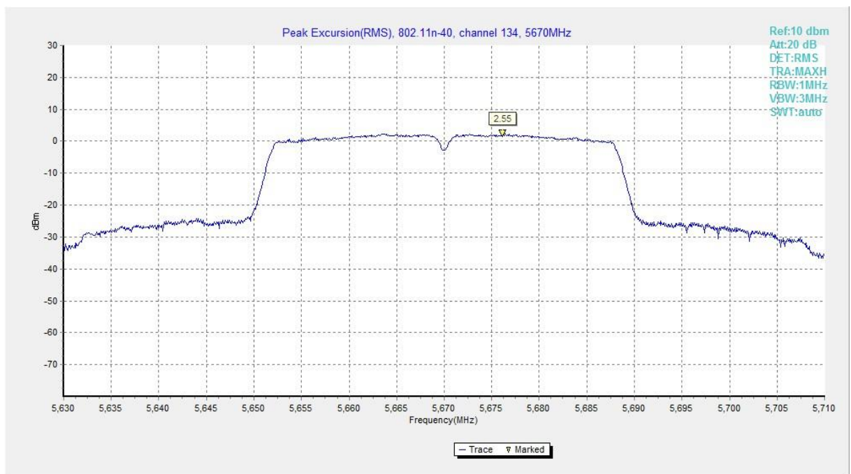
Fig. 179 Peak Excursions (802.11n-HT40, ch134, average)
