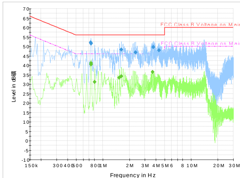
Fig. 129 Conducted Emission(802.11a, IDLE)
