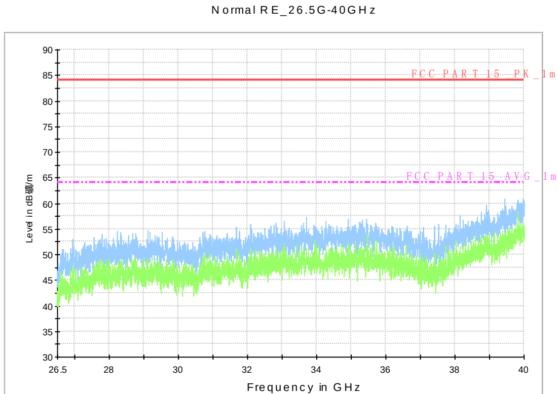
Fig. 124 Radiated Spurious Emission (802.11n-HT40, ch118, 26.5 GHz-40 GHz)
