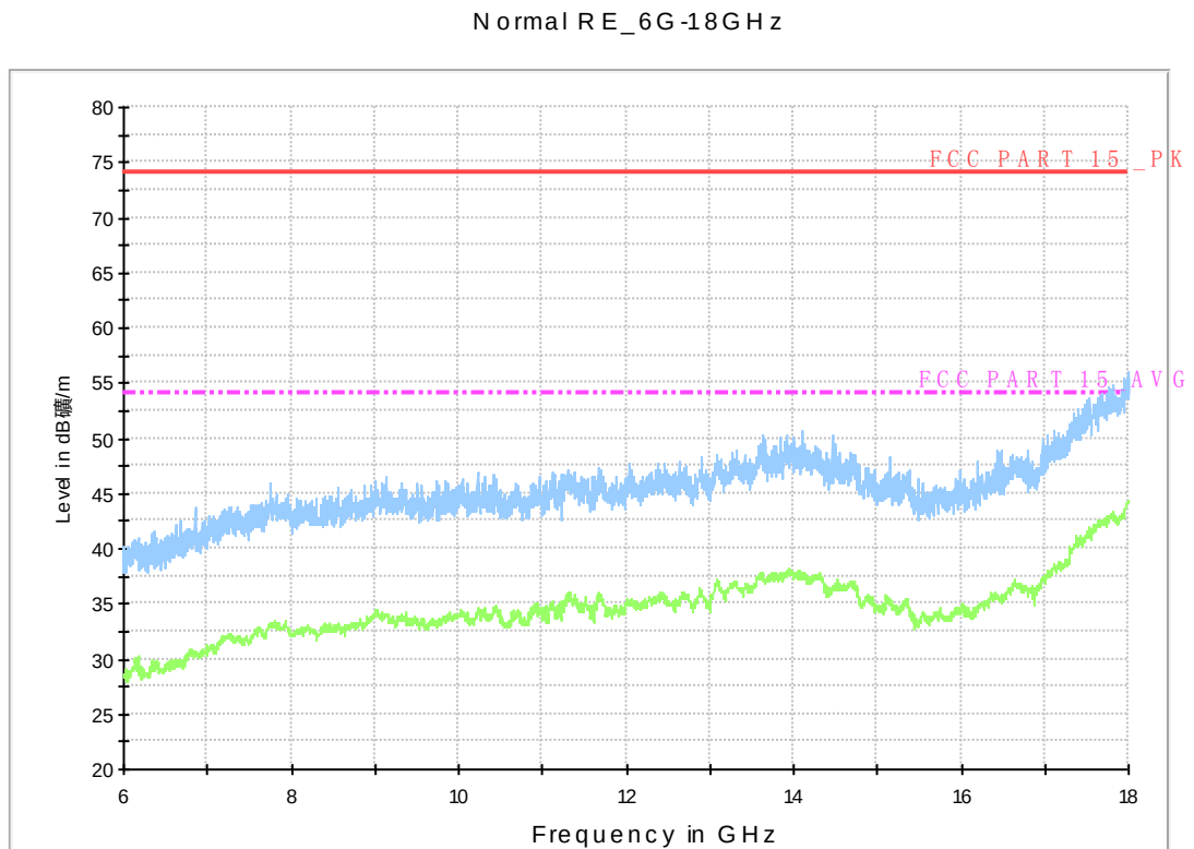
Fig. 119 Radiated Spurious Emission (802.11n-HT40, ch102, 6 GHz-18 GHz)
