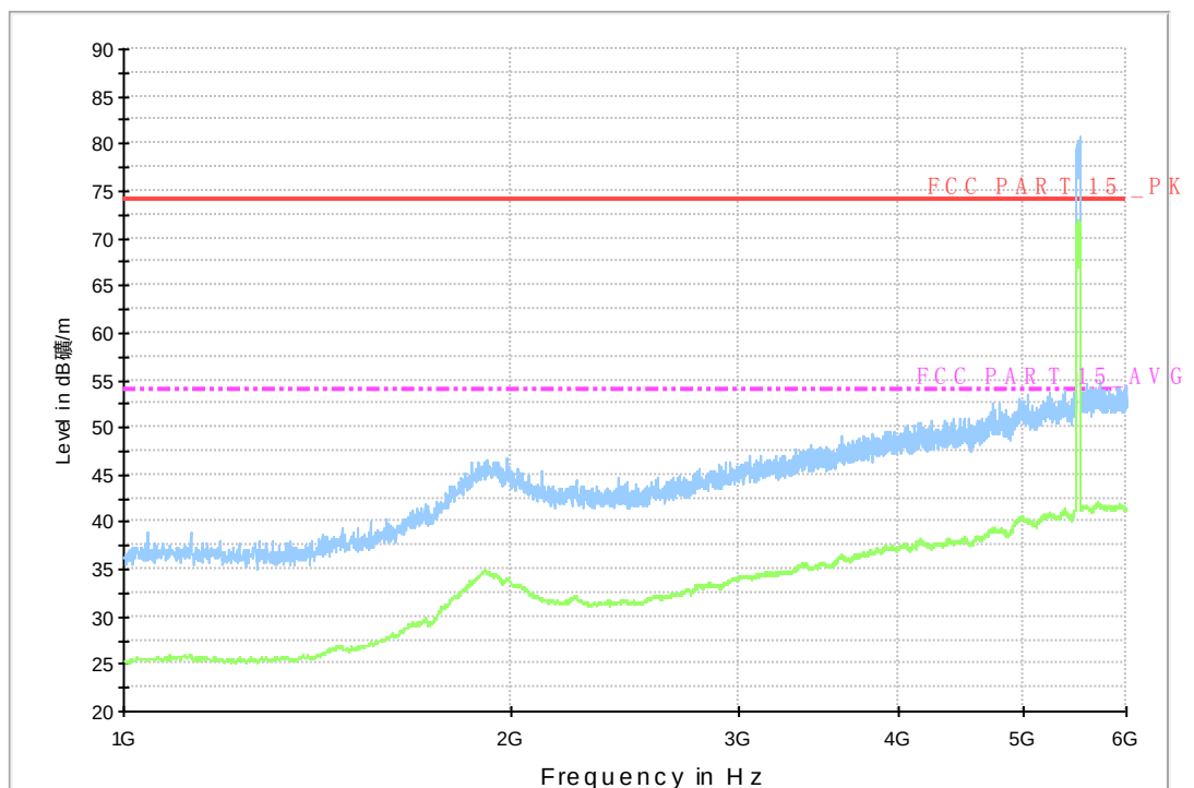
RE_WLAN_1G-6GHz
