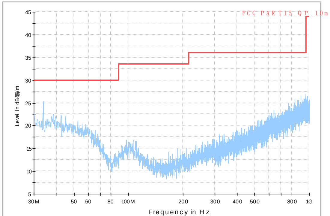
Normal RE_30M-1GHz_10m
