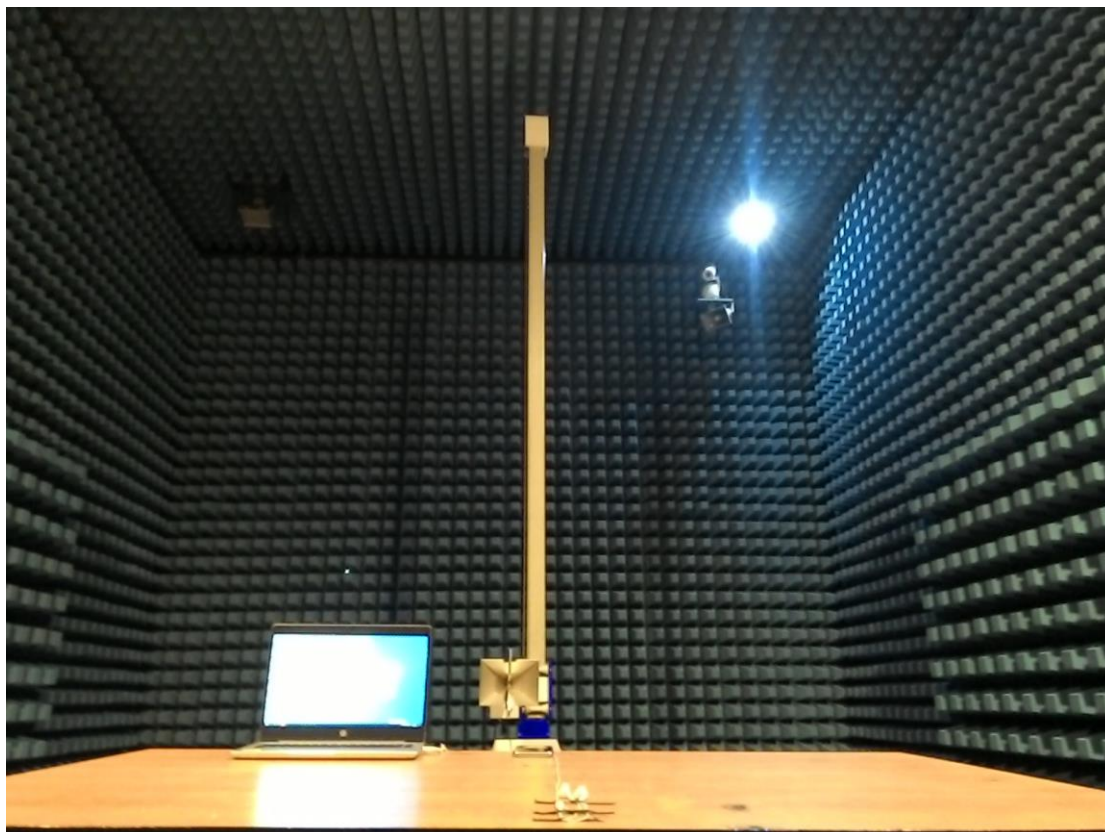
FCC Part15B Radiated Emission above 1GHz -Front
