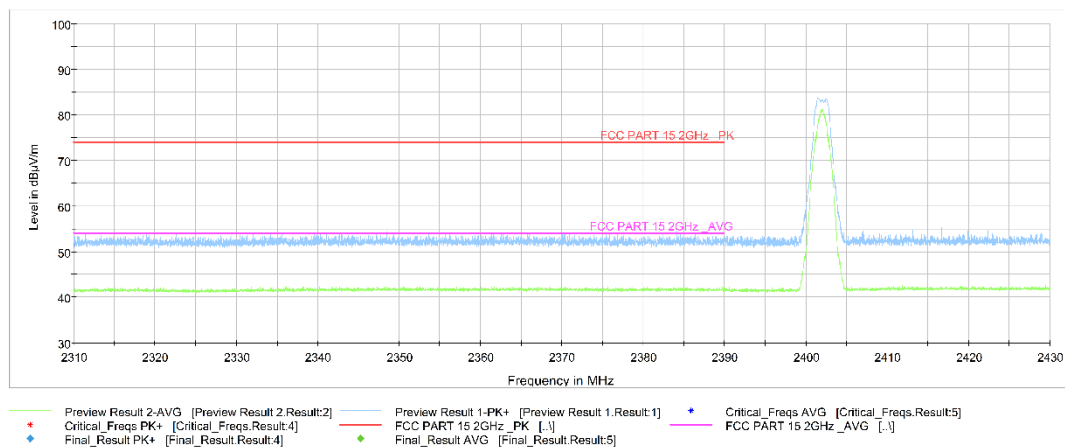
Fig.3. Frequency Band Edges: GFSK, 2402 MHz, Hopping Off, 2.31 GHz – 2.43GHz
