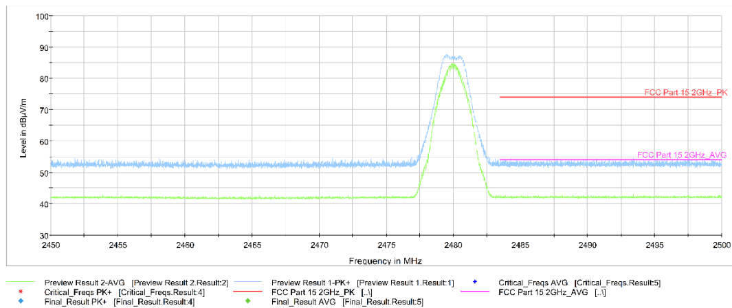
Fig.4. Frequency Band Edges: GFSK, 2480 MHz, Hopping Off, 2.45 GHz - 2.50GHz
