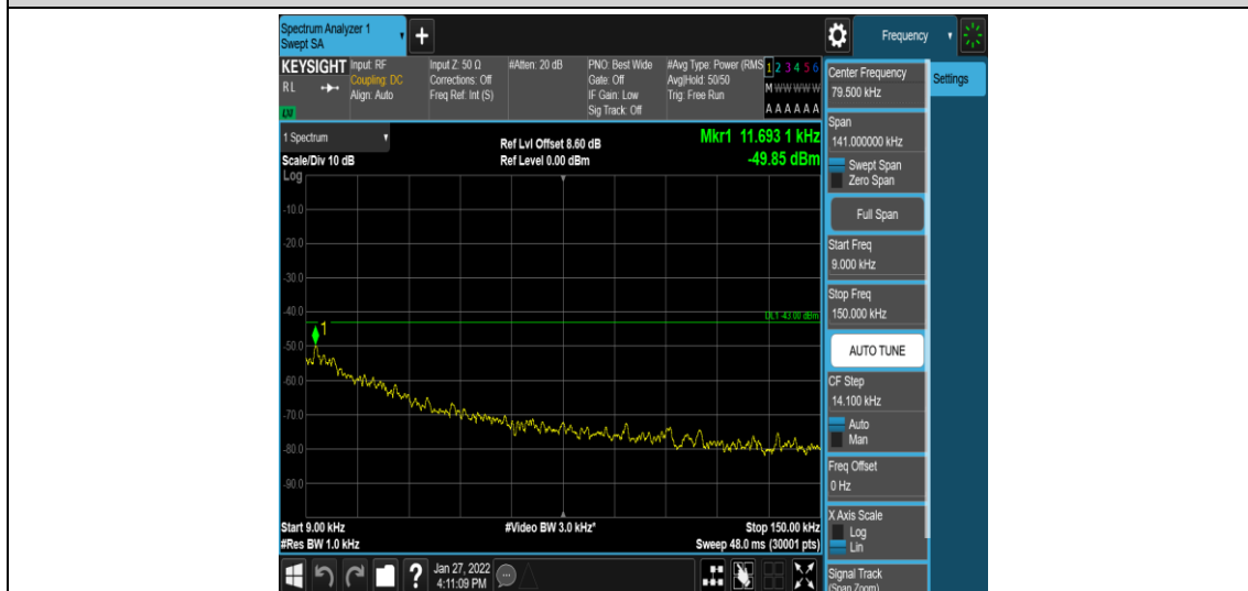
Band4-10MHz-QPSK-20175-1-0-Low-0.009-0.15--49.85-PASS
