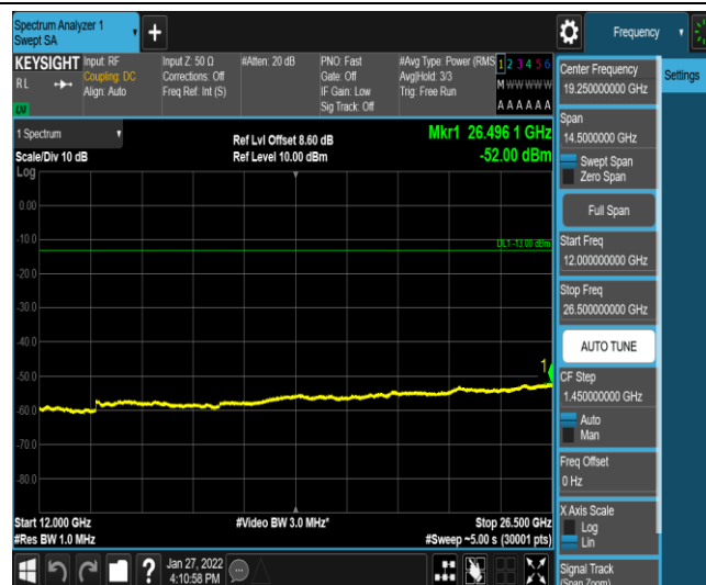
Band4-10MHz-16QAM-20000-1-0-Low-12000-26500--52-PASS
