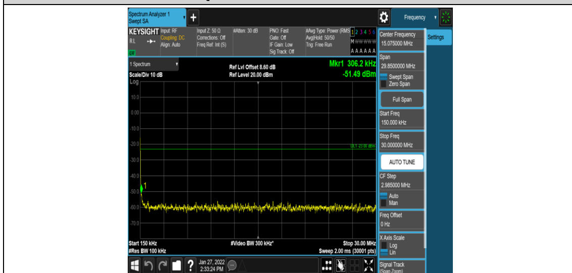
Band4-5MHz-16QAM-20175-1-0-Low-0.15-30--51.49-PASS
