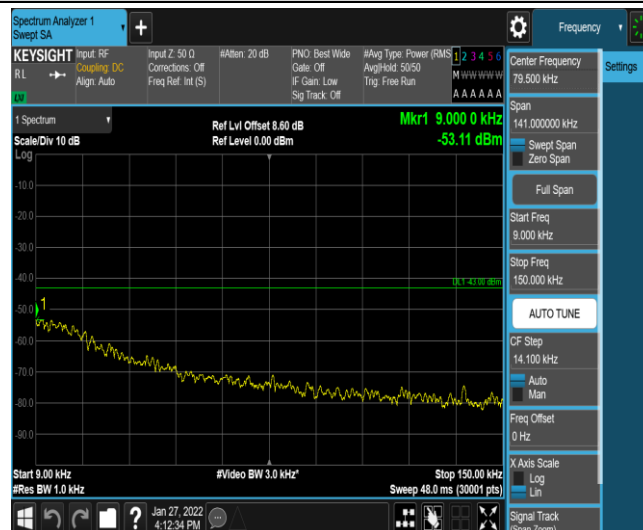
Band4-10MHz-16QAM-20175-1-0-Low-0.009-0.15--53.11-PASS
