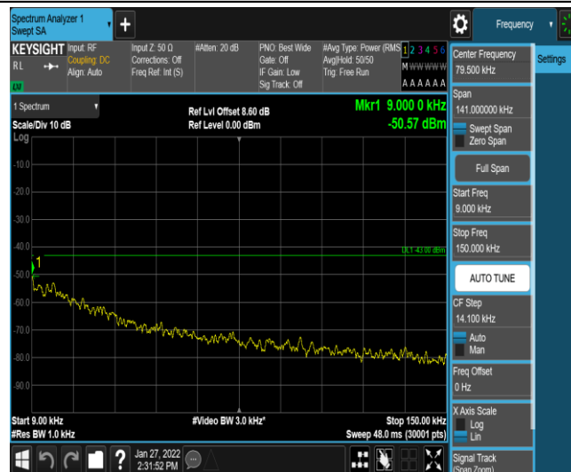
Band4-5MHz-QPSK-20175-1-0-Low-0.009-0.15--50.57-PASS
