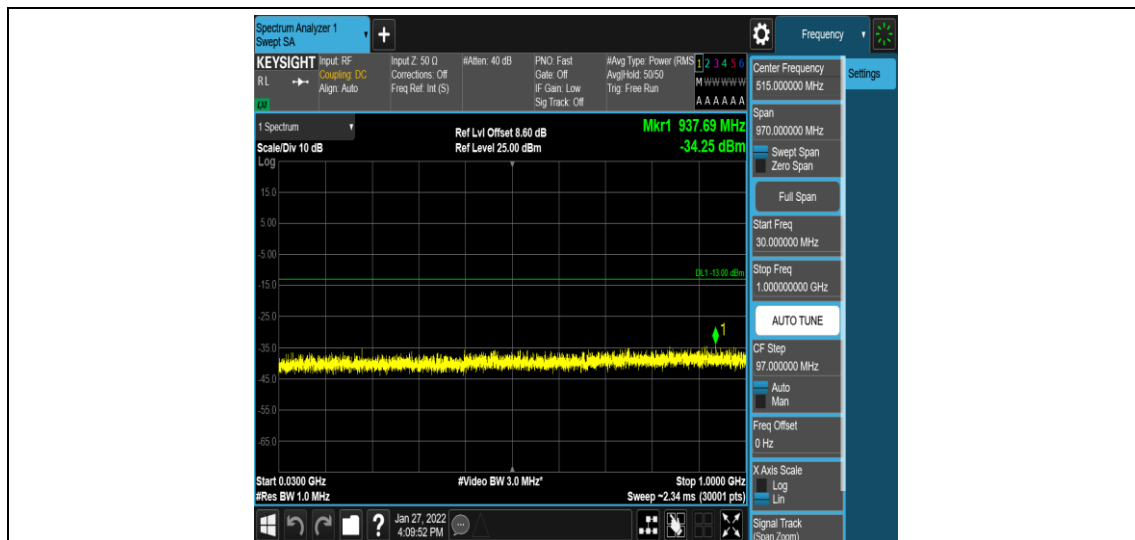
Band4-10MHz-16QAM-20000-1-0-Low-30-1000--34.26-PASS
