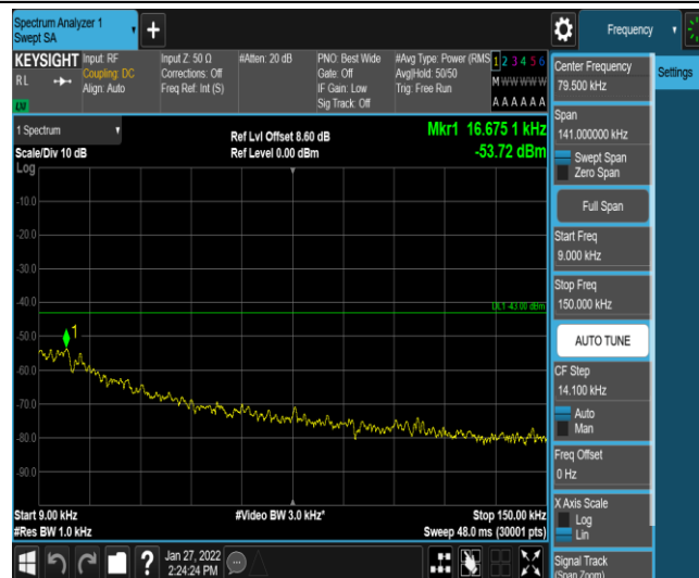
Band4-5MHz-16QAM-19975-1-0-Low-0.009-0.15--53.72-PASS
