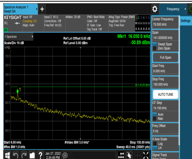
Band4-5MHz-QPSK-20375-1-0-High-0.009-0.15--50.9-PASS
