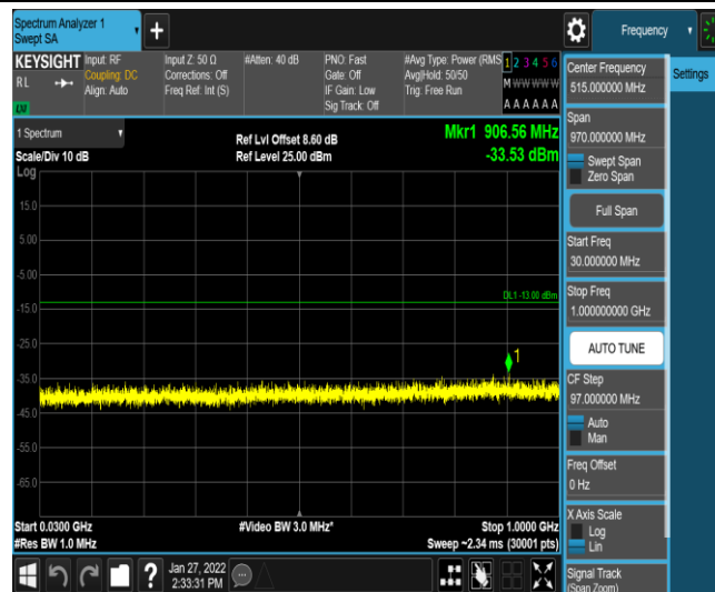
Band4-5MHz-16QAM-20175-1-0-Low-30-1000--33.53-PASS
