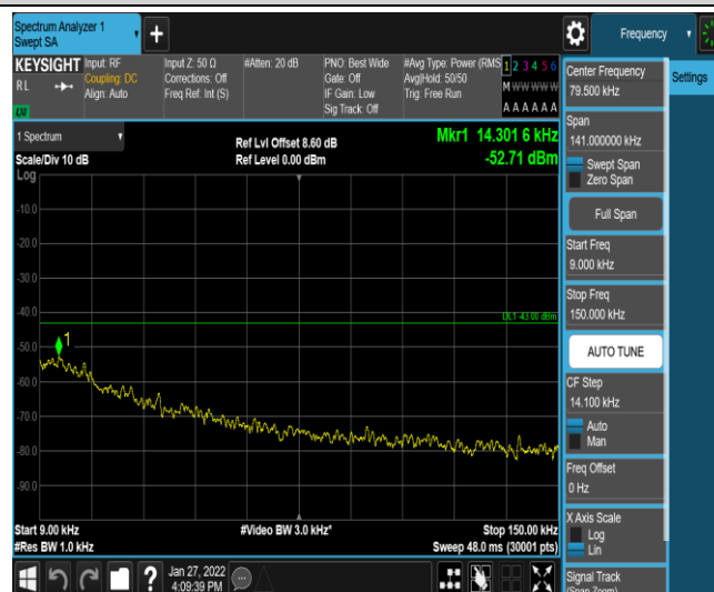
Band4-10MHz-16QAM-20000-1-0-Low-0.009-0.15--52.71-PASS
