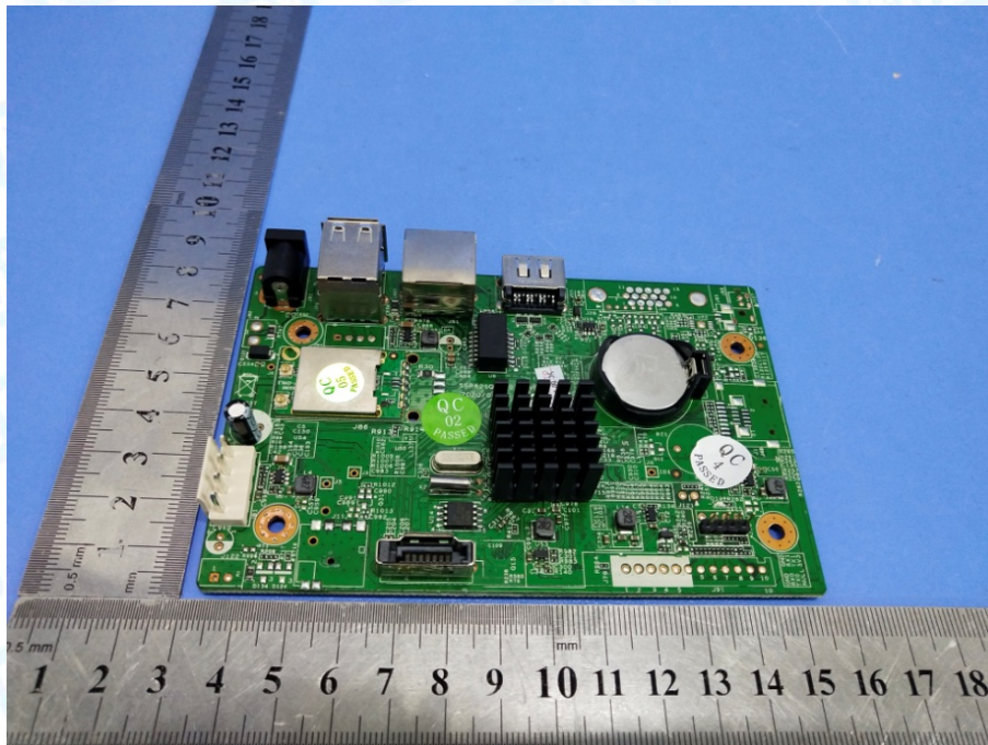
Photo 15 Appearance of PCB-Project 2
