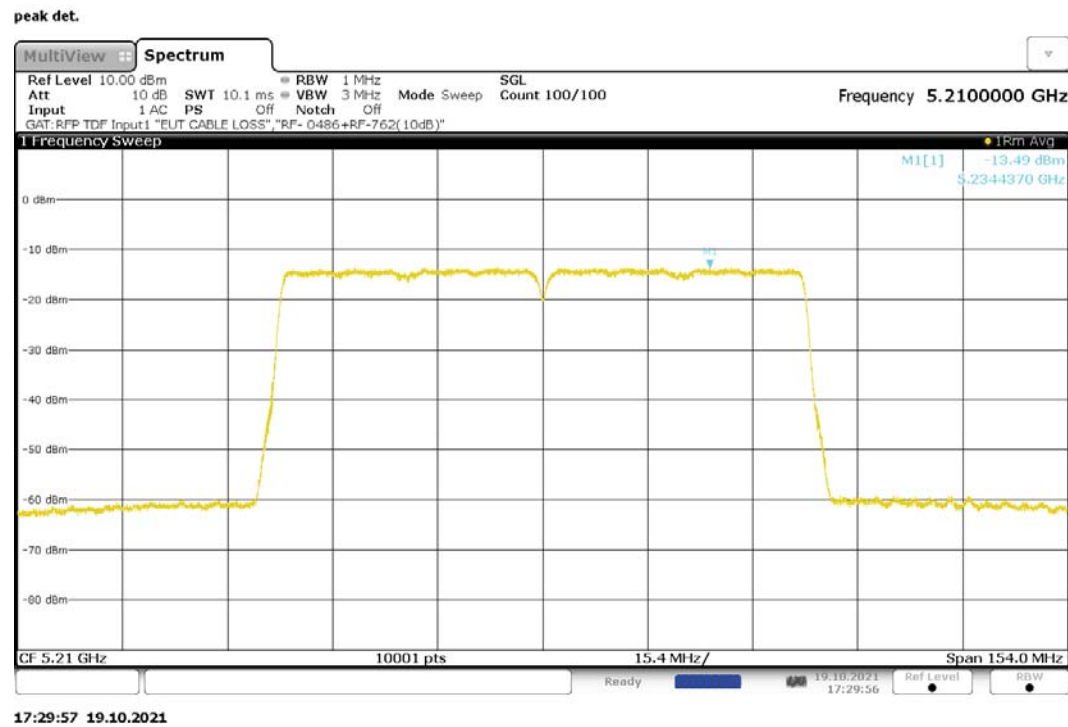
Figure 273: Maximum Power Spectral Density, 802.11ac-80, MIMO, RF1, 5210MHz
