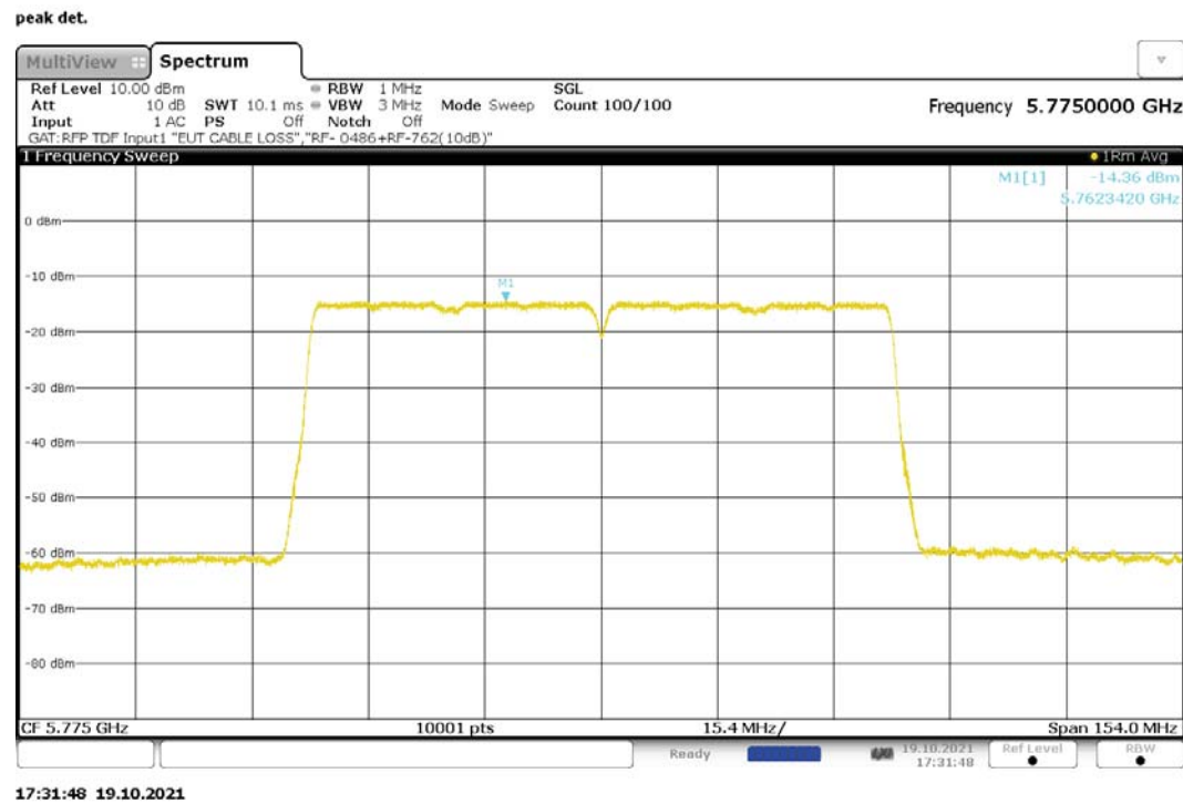
Figure 274: Maximum Power Spectral Density, 802.11ac-80, MIMO, RF1, 5775MHz
