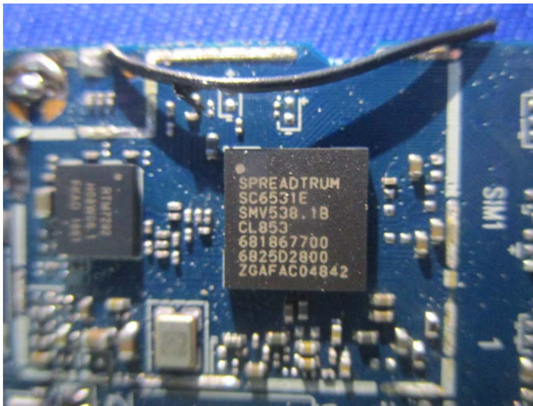
Main Chipset
