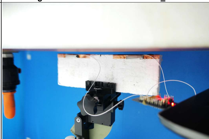
Bottom Side of EUT Tested at 5 mm_USB
