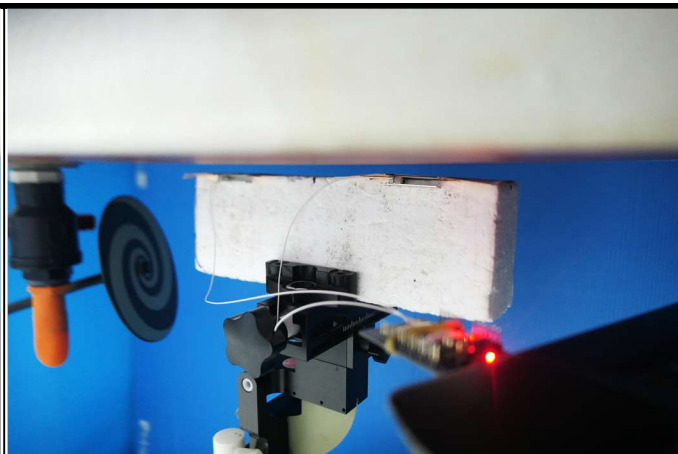
Rear Face of EUT Tested at 5 mm_USB
