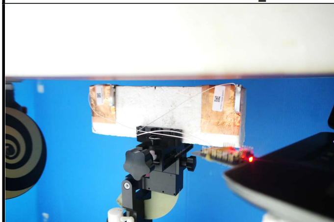
Left Side of EUT Tested at 5 mm_USB
