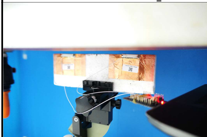
Top Side of EUT Tested at 5 mm_USB
