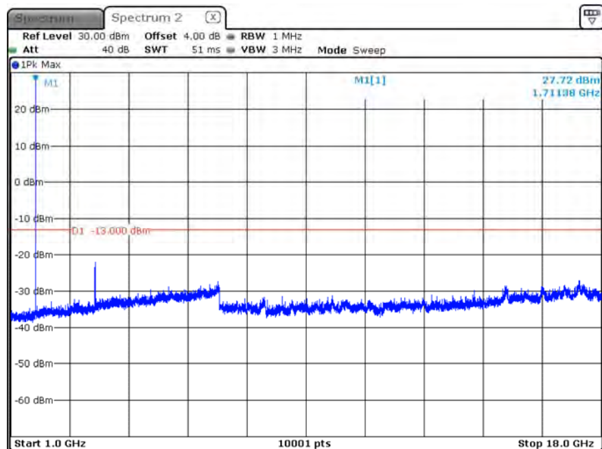
B66_CH132047_15M_1RB0_16-QAM_Above 1G
