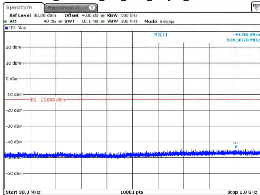
B66_CH132322_10M_1RB0_16-QAM_Below 1G
