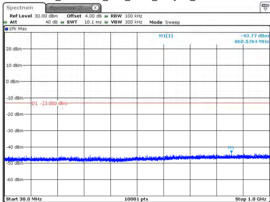
B66_CH132047_15M_1RB0_16-QAM_Below 1G
