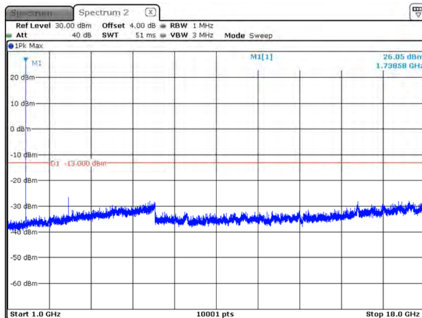
B66_CH132322_15M_1RB0_16-QAM_Above 1G
