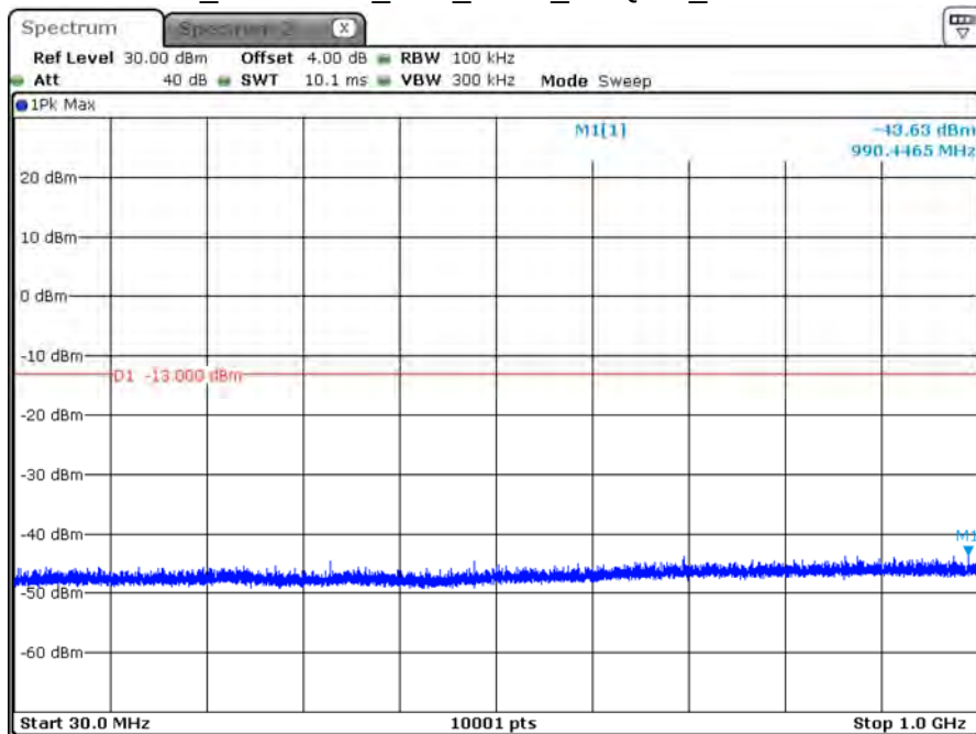
B66_CH132622_10M_1RB5_16-QAM_Below 1G
