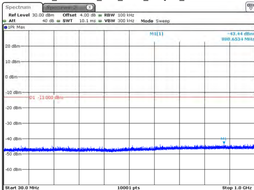
B66_CH132322_20M_1RB0_16-QAM_Below 1G
