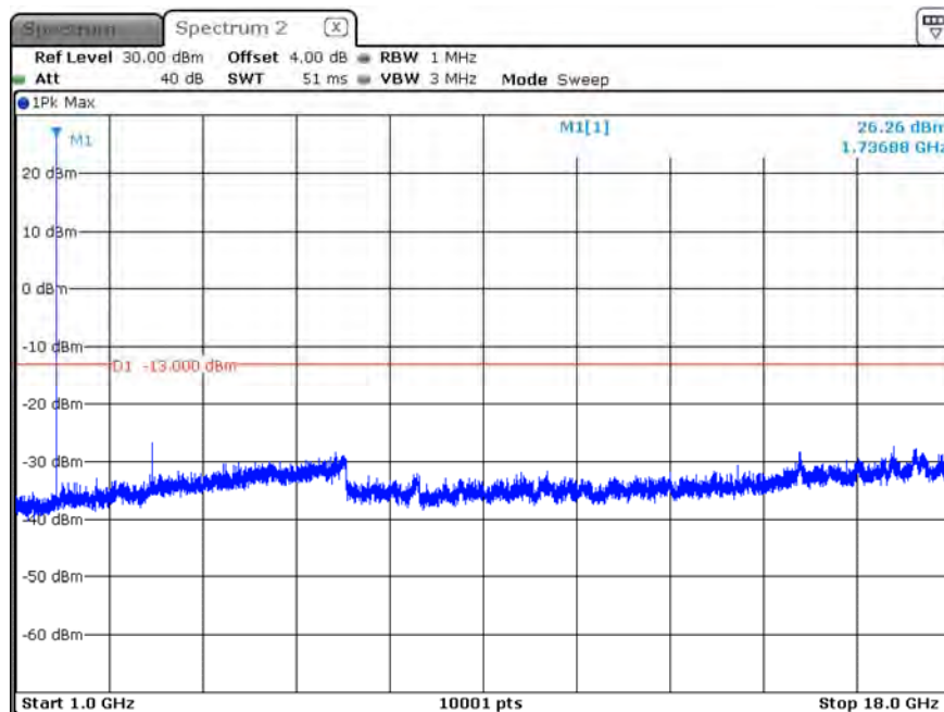
B66_CH132322_20M_1RB0_16-QAM_Above 1G
