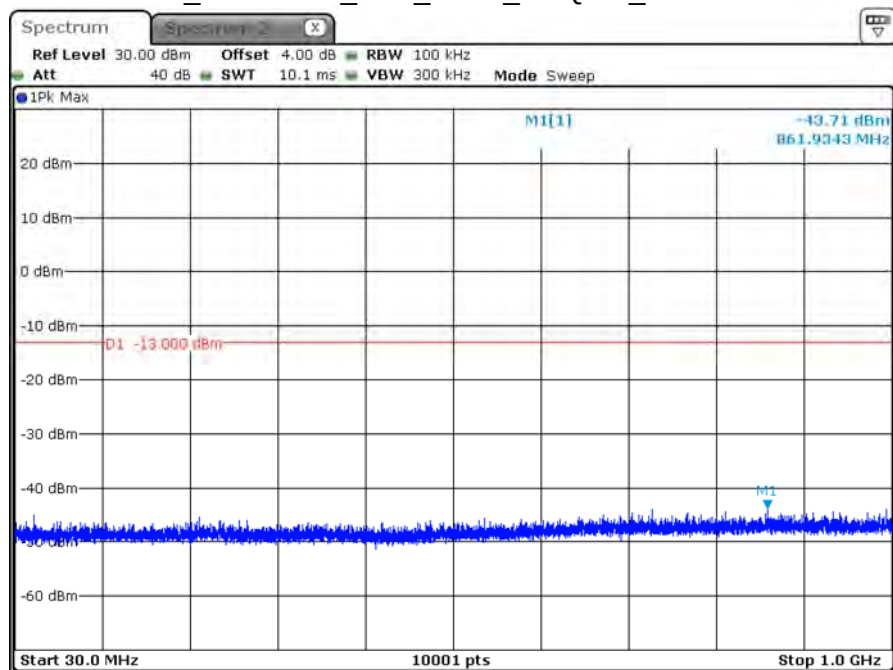
B66_CH132597_15M_1RB5_16-QAM_Below 1G
