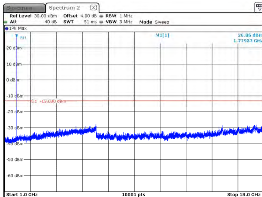
B66_CH132622_10M_1RB5_16-QAM_Above 1G
