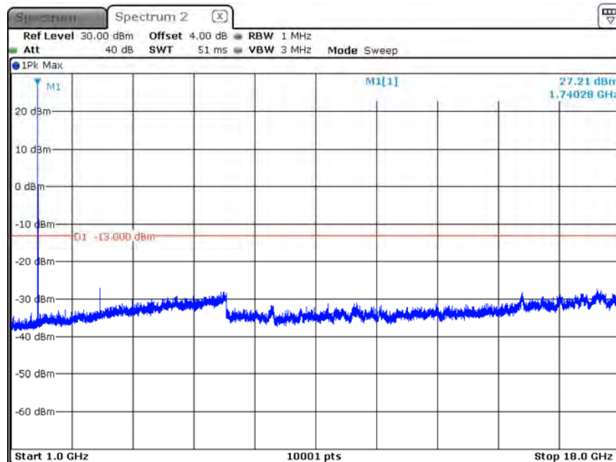
B66_CH132322_10M_1RB0_16-QAM_Above 1G
