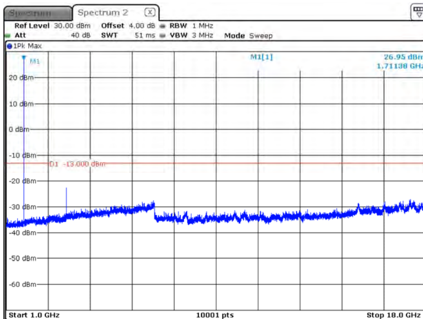
B66_CH132072_20M_1RB0_16-QAM_Above 1G
