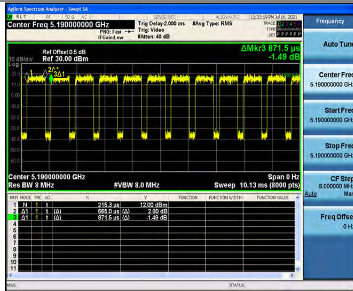
802.11n(HT40)_Ant2_5190
