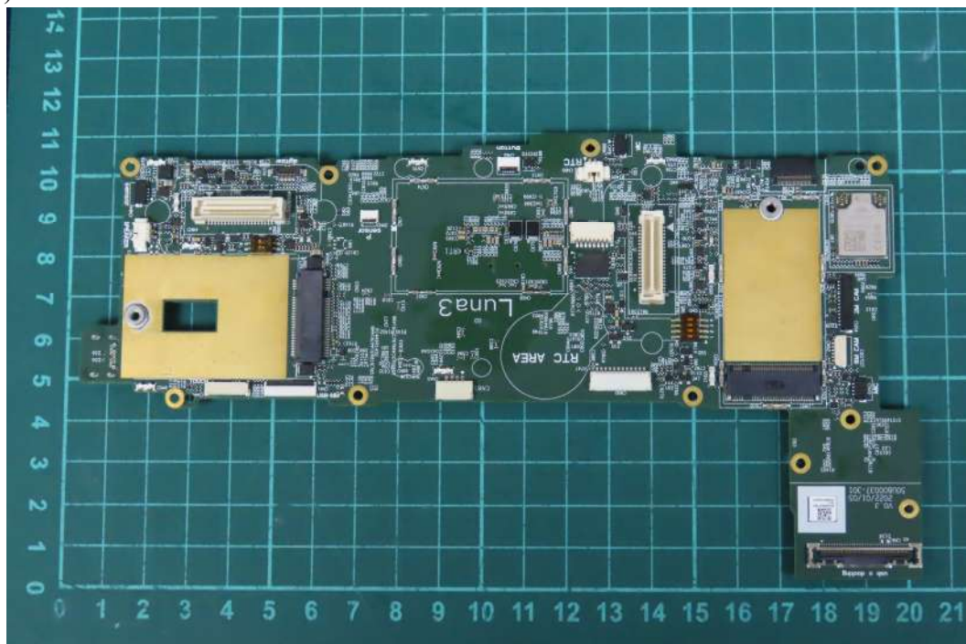
(38) EUT Photo
