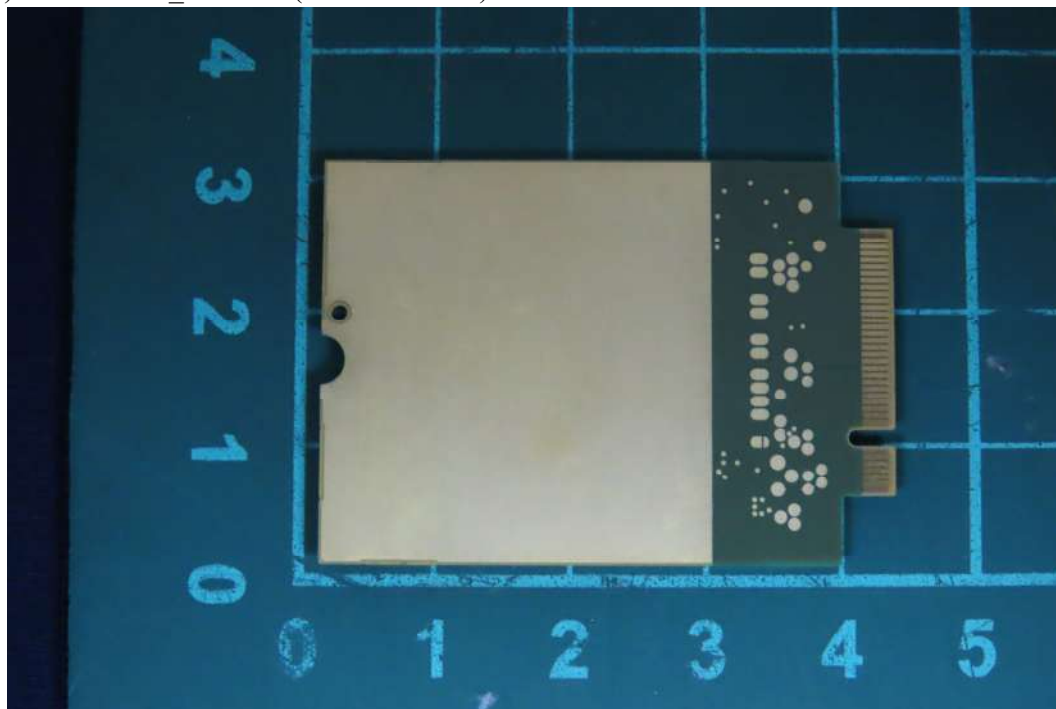
(35) EUT Photo _EM7411 (For FCC/ISED)
