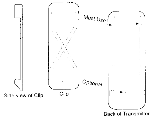
Figure 2. Belt Clip Attachment
