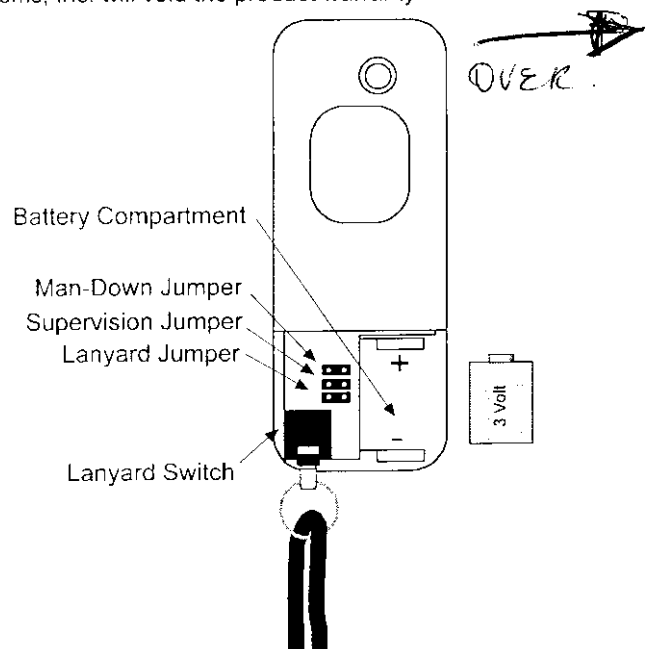
Figure 5. Internal Components
