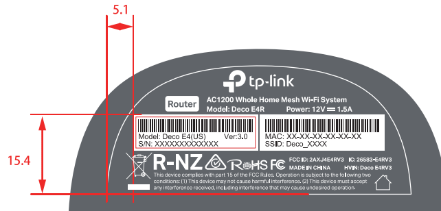
58.66*24.78mm ±0.2
