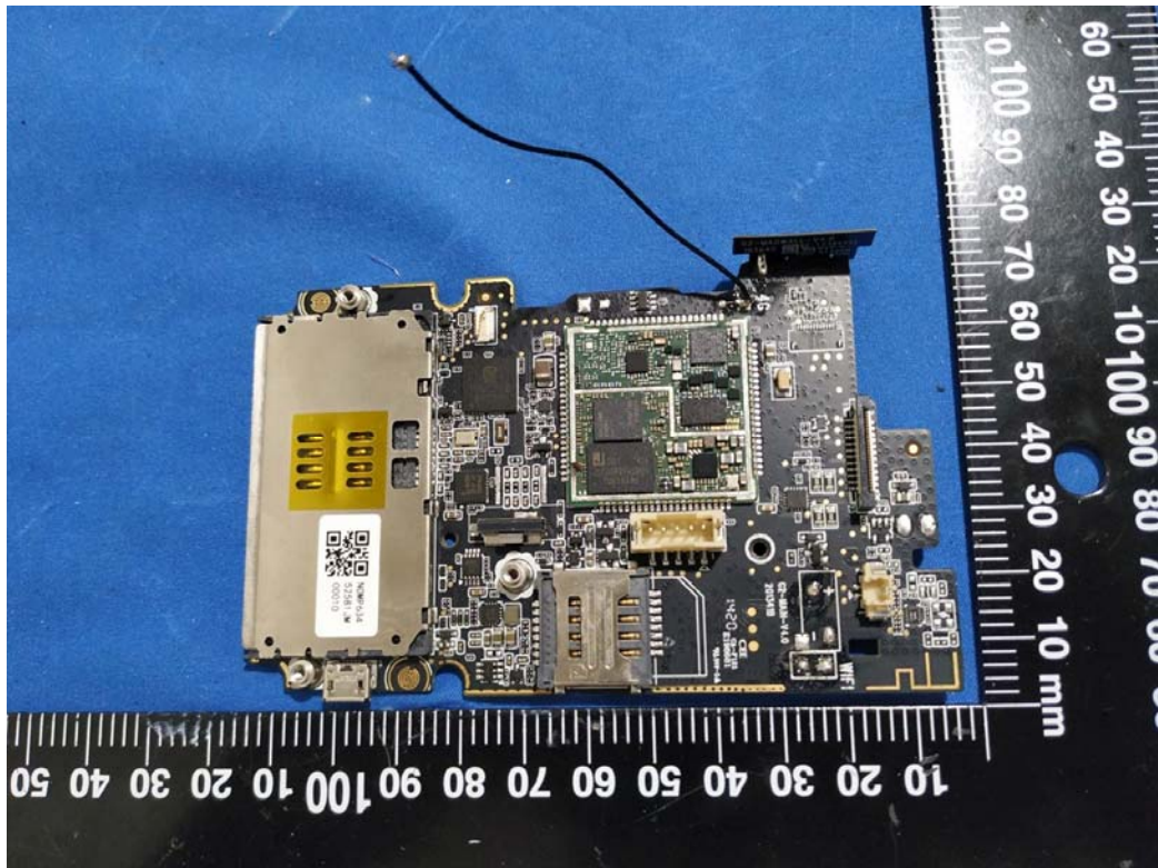
BT Antenna
