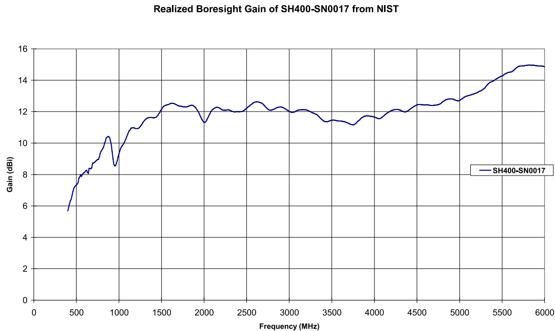
Figure 3 – NIST calibrated boresight gain vs. frequency plot of the MVG SH400-SN0017
