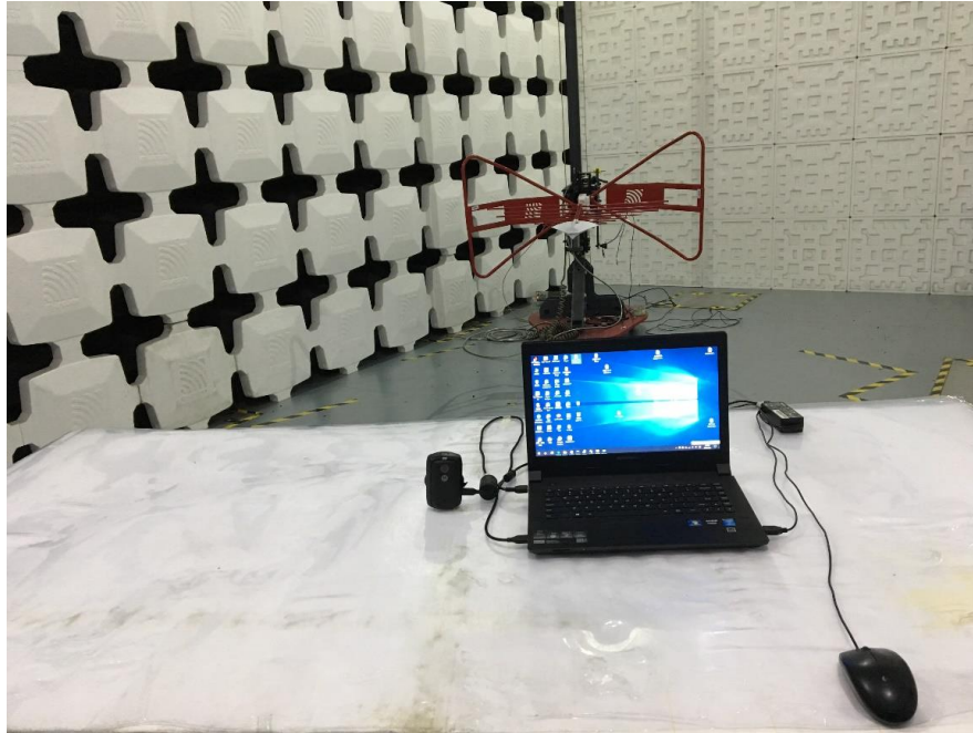
Figure 1: Radiated Emission Test Setup (30MHz~1GHz)
