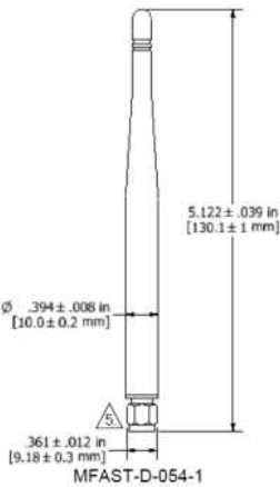
Figure 6: Antenna Configuration
