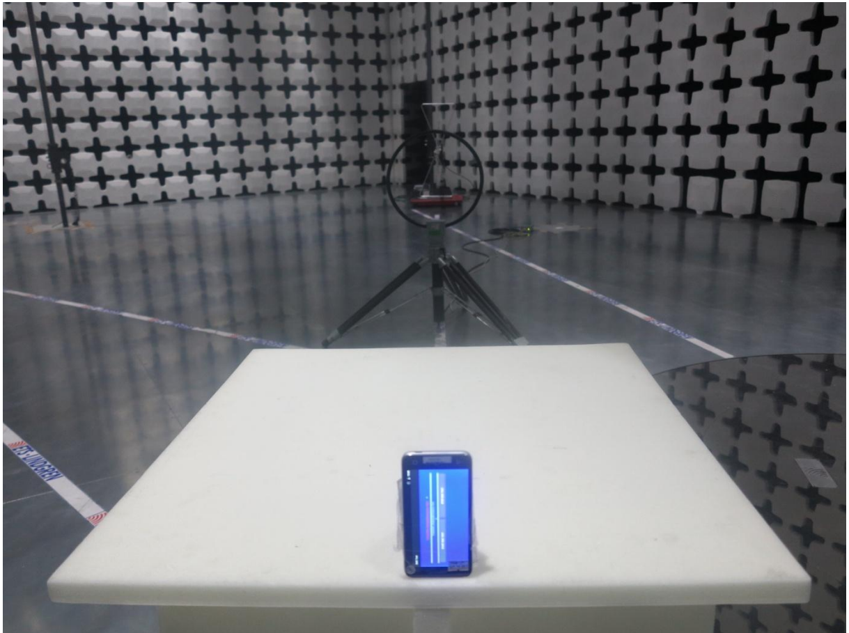
Picture B-1: Field Strength Measurements (Below 30MHz)
