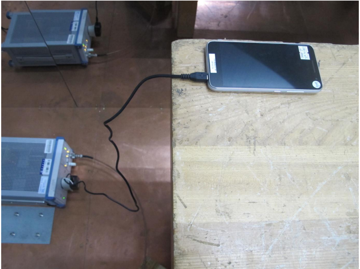
Picture B-3: Conducted Emissions Measurements
