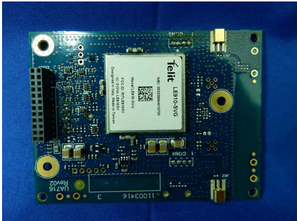
(1) EUT Photo
