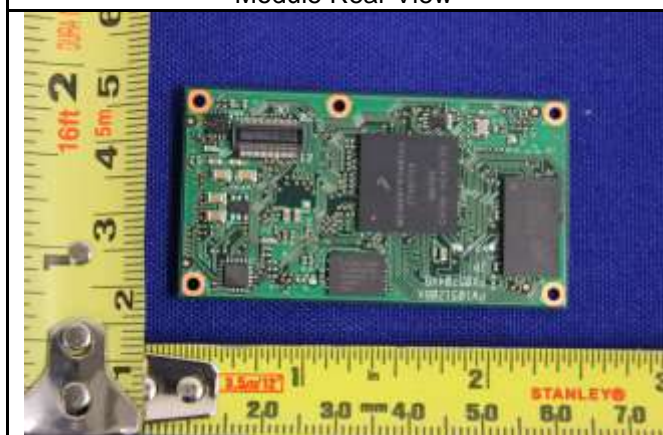
PCB3 Rear View
