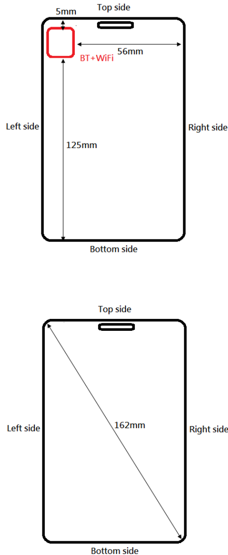
Fig.15 Antenna location and dimensional size
