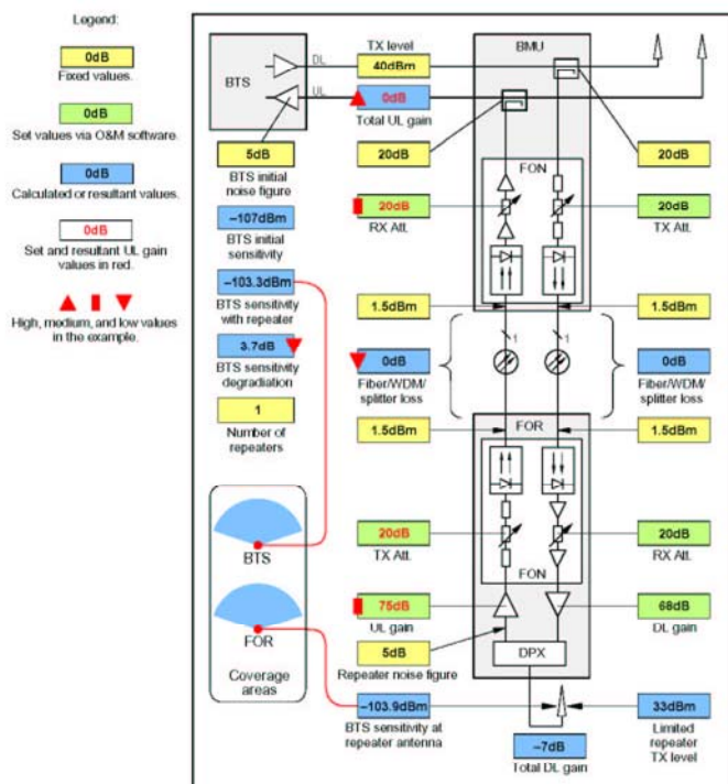
Figure 6-5. One FOR, low optical loss, medium uplink gain and attenuation
