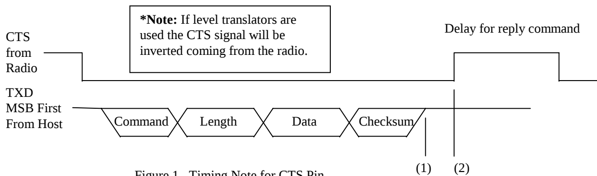
Figure 1. Timing Note for CTS Pin
