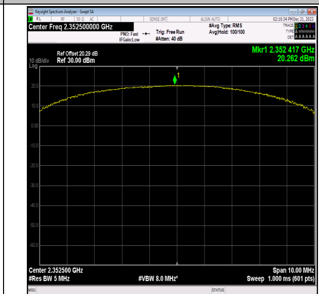
40(2350-2360)-5MHz-QPSK-39175-25RB#0-PASS
