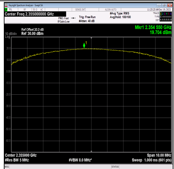
40(2350-2360)-5MHz-QPSK-39200-25RB#12-PASS
