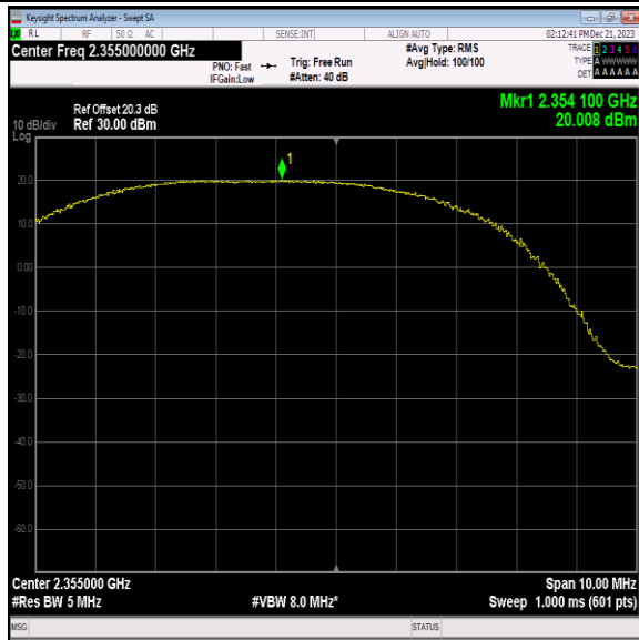
40(2350-2360)-5MHz-QPSK-39200-12RB#6-PASS
