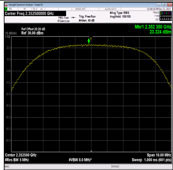
40(2350-2360)-5MHz-QPSK-39175-1RB#12-PASS
