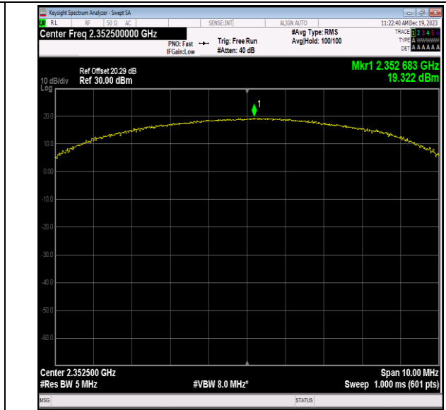
40(2350-2360)-5MHz-16QAM-39175-25RB#12-PASS
