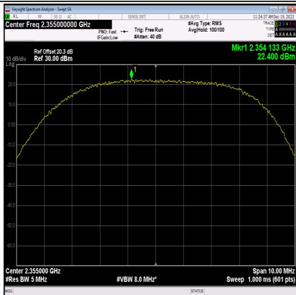
40(2350-2360)-5MHz-QPSK-39200-1RB#49-PASS
