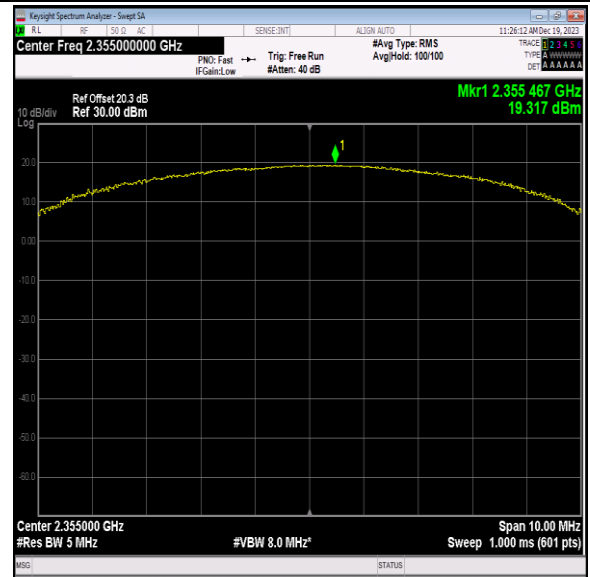
40(2350-2360)-5MHz-QPSK-39200-50RB#0-PASS
