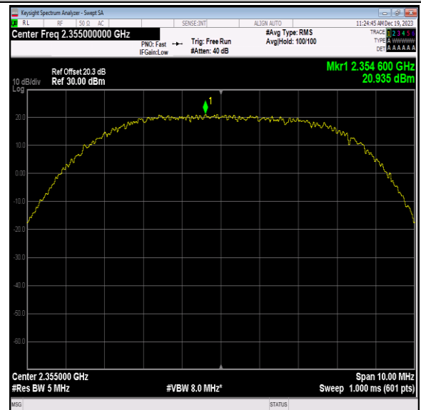
40(2350-2360)-5MHz-16QAM-39200-1RB#49-PASS
