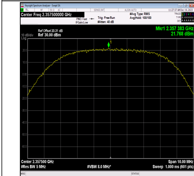
40(2350-2360)-5MHz-16QAM-39225-1RB#49-PASS
