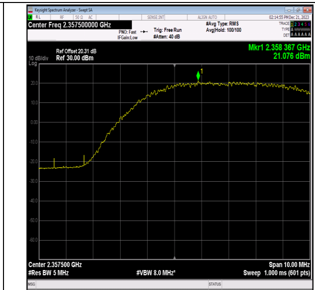
40(2350-2360)-5MHz-16QAM-39225-1RB#24-PASS
