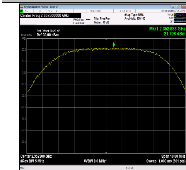
40(2350-2360)-5MHz-16QAM-39175-1RB#12-PASS
