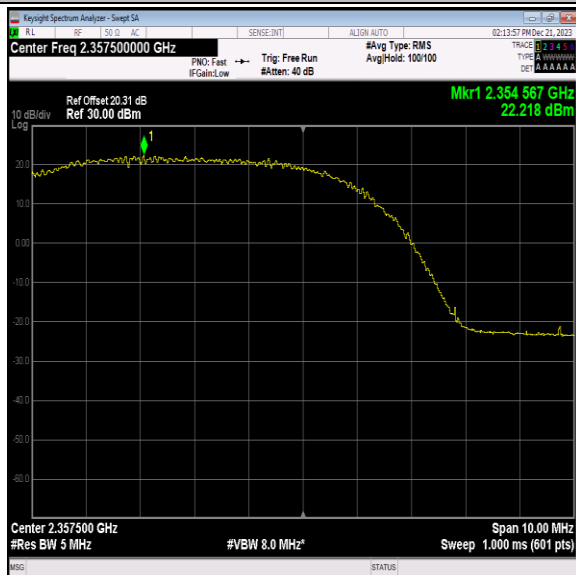
40(2350-2360)-5MHz-QPSK-39225-1RB#0-PASS
