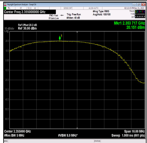
40(2350-2360)-5MHz-QPSK-39200-12RB#0-PASS
