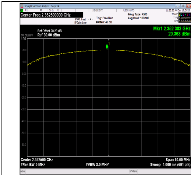
40(2350-2360)-5MHz-QPSK-39175-25RB#12-PASS
