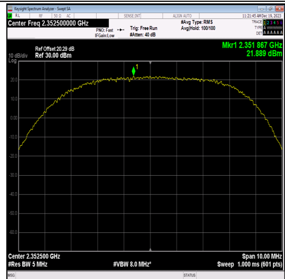
40(2350-2360)-5MHz-QPSK-39175-1RB#49-PASS
