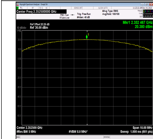
40(2350-2360)-5MHz-QPSK-39175-50RB#0-PASS
