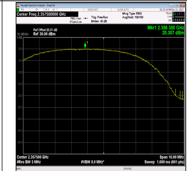
40(2350-2360)-5MHz-16QAM-39225-12RB#0-PASS
