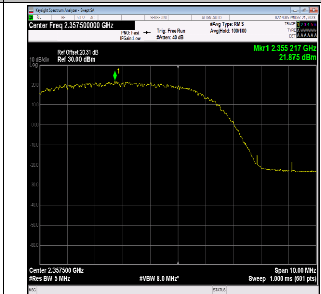
40(2350-2360)-5MHz-16QAM-39225-1RB#0-PASS
