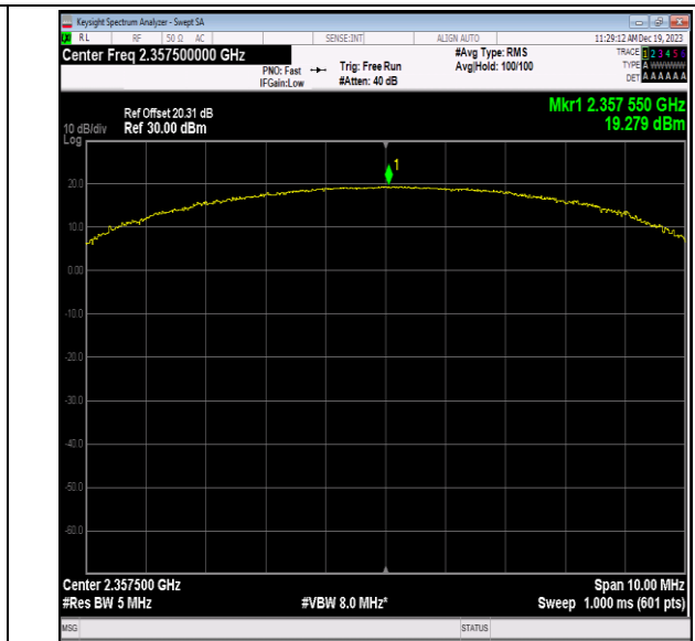
40(2350-2360)-5MHz-16QAM-39225-50RB#0-PASS
