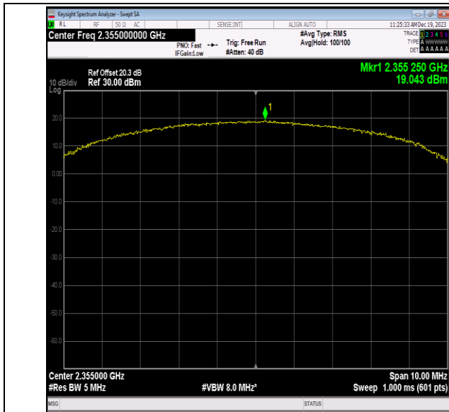
40(2350-2360)-5MHz-16QAM-39200-25RB#12-PASS
