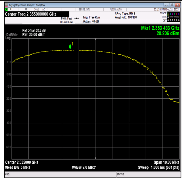
40(2350-2360)-5MHz-QPSK-39200-12RB#11-PASS
