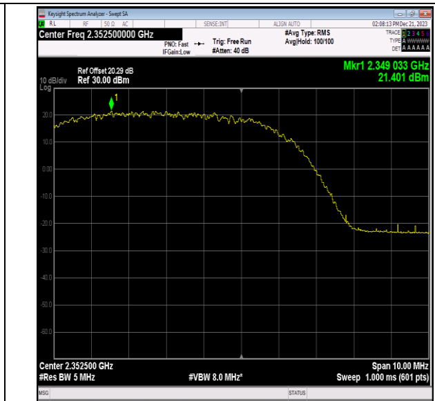
40(2350-2360)-5MHz-16QAM-39175-1RB#0-PASS
