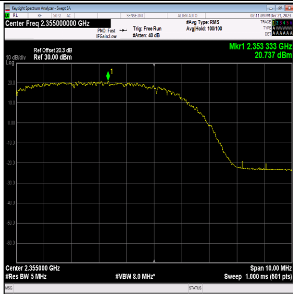
40(2350-2360)-5MHz-16QAM-39200-1RB#0-PASS
