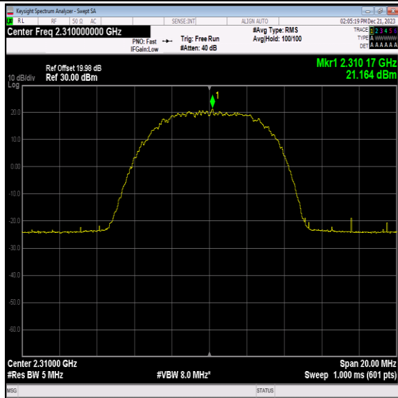
40(2305-2315)-10MHz-64QAM-38750-1RB#24-PASS
