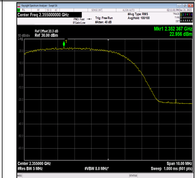
40(2350-2360)-5MHz-QPSK-39200-1RB#0-PASS
