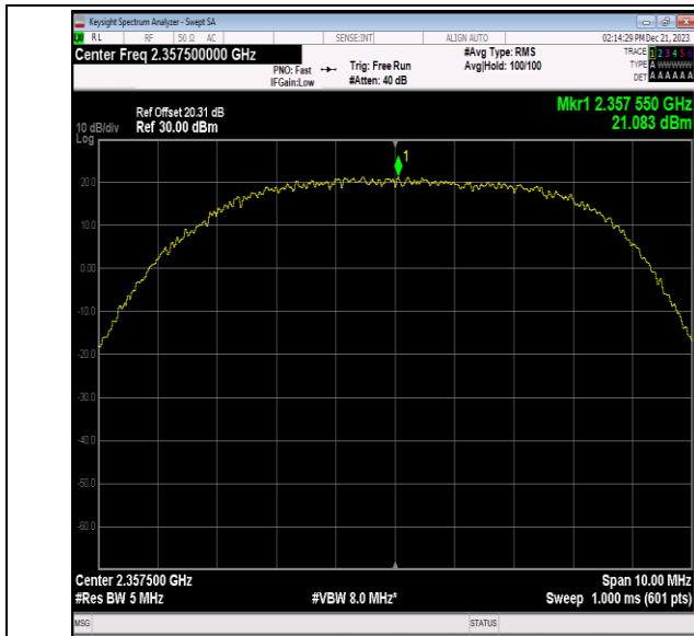
40(2350-2360)-5MHz-16QAM-39225-1RB#12-PASS
