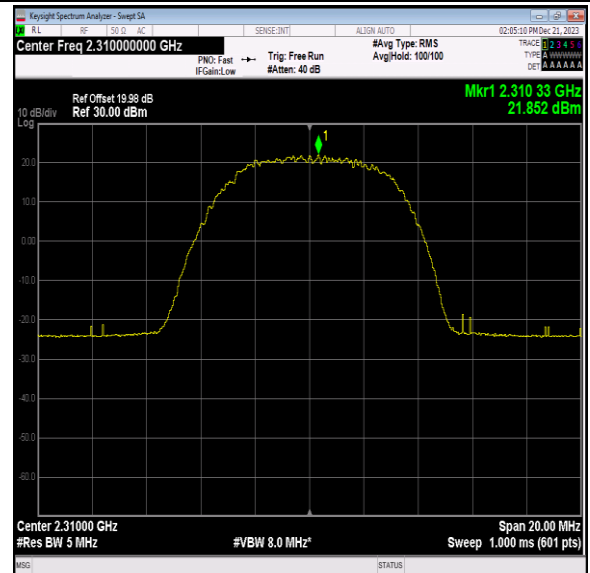
40(2305-2315)-10MHz-16QAM-38750-1RB#24-PASS
