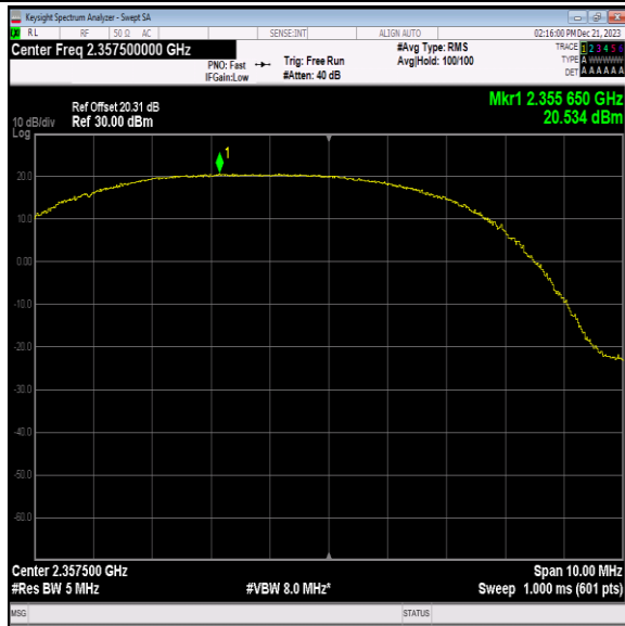
40(2350-2360)-5MHz-QPSK-39225-12RB#11-PASS
