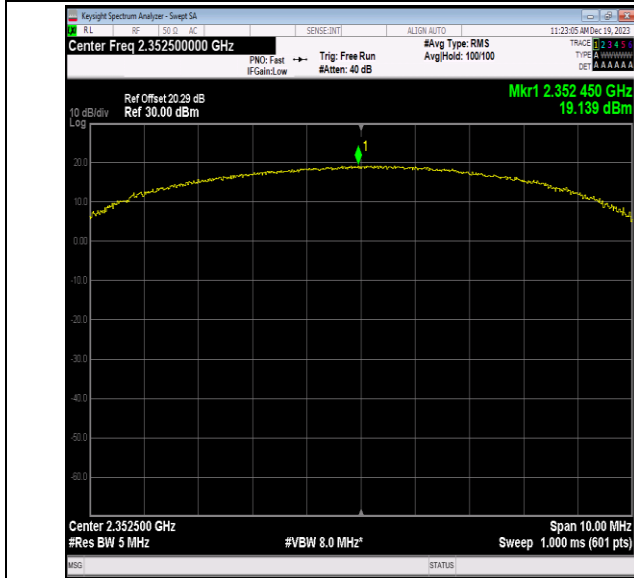
40(2350-2360)-5MHz-16QAM-39175-25RB#25-PASS
