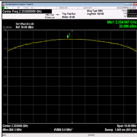
40(2350-2360)-5MHz-QPSK-39200-25RB#0-PASS
