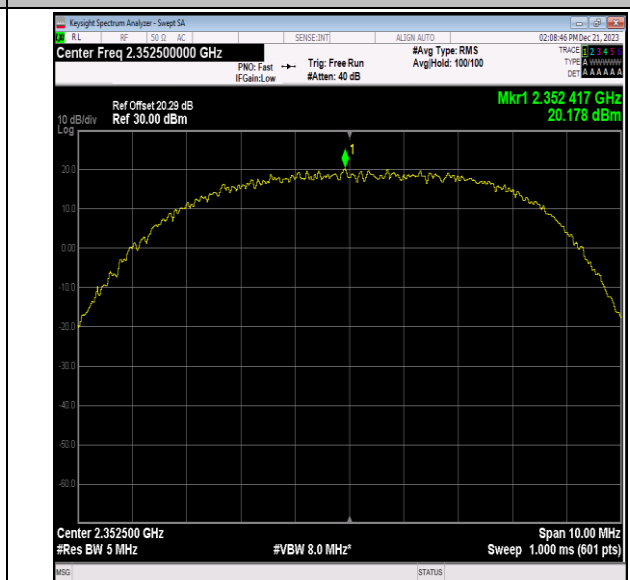
40(2350-2360)-5MHz-64QAM-39175-1RB#12-PASS
