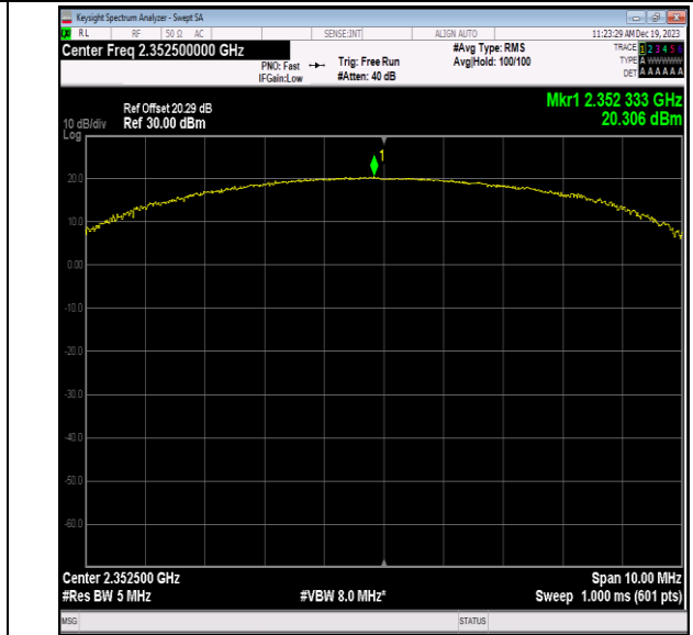
40(2350-2360)-5MHz-16QAM-39175-50RB#0-PASS
