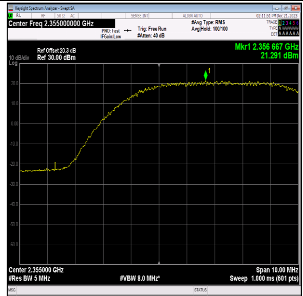
40(2350-2360)-5MHz-QPSK-39200-1RB#24-PASS
