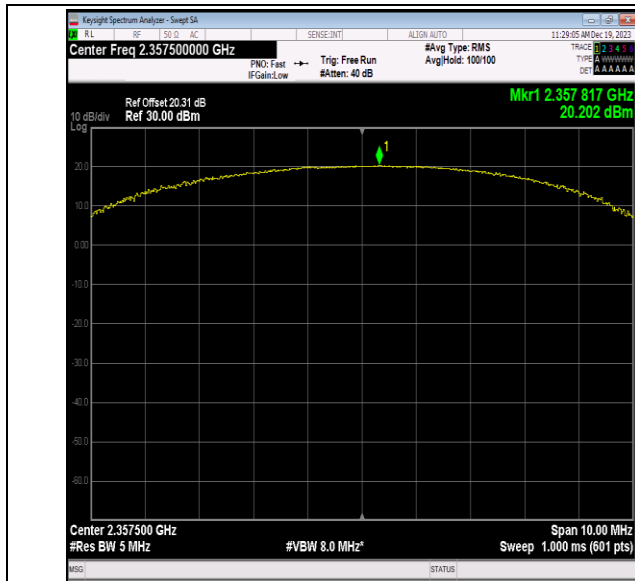
40(2350-2360)-5MHz-QPSK-39225-50RB#0-PASS
