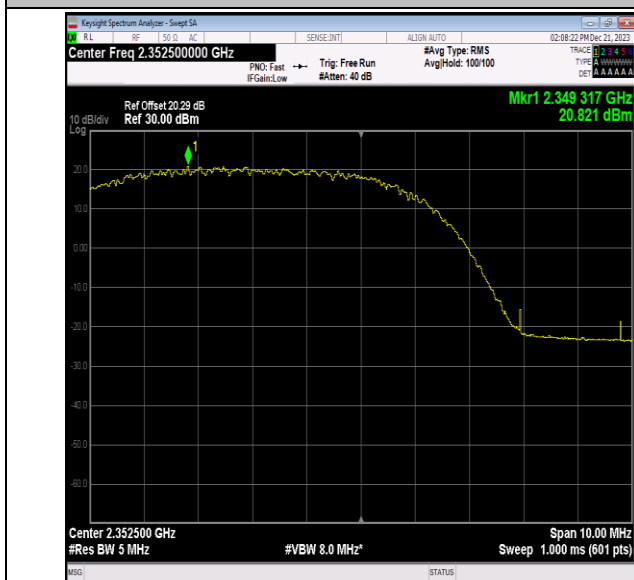
40(2350-2360)-5MHz-64QAM-39175-1RB#0-PASS
