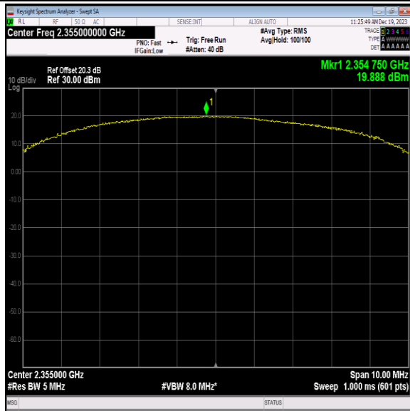
40(2350-2360)-5MHz-QPSK-39200-25RB#25-PASS
