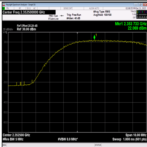
40(2350-2360)-5MHz-QPSK-39175-1RB#24-PASS
