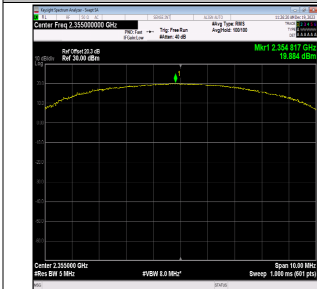
40(2350-2360)-5MHz-16QAM-39200-50RB#0-PASS
