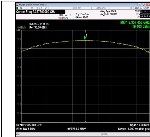
40(2350-2360)-5MHz-16QAM-39225-25RB#25-PASS
