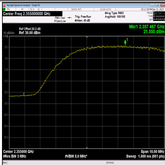
40(2350-2360)-5MHz-16QAM-39200-1RB#24-PASS
