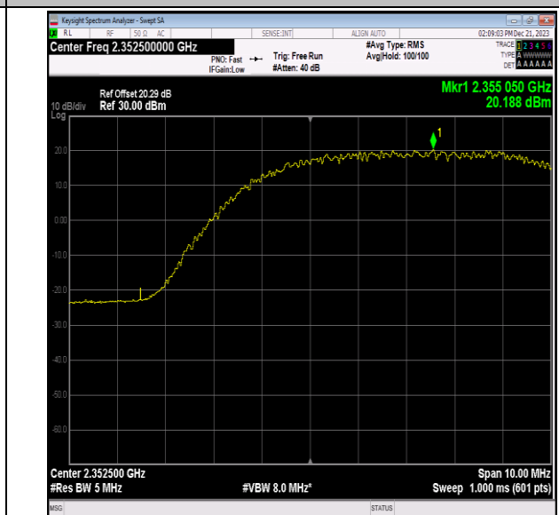
40(2350-2360)-5MHz-16QAM-39175-1RB#24-PASS
