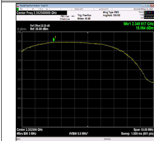
40(2350-2360)-5MHz-QPSK-39175-12RB#11-PASS
