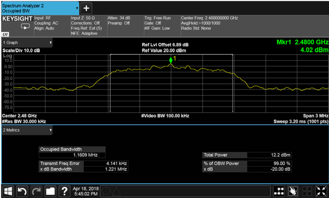
Figure 22 – 2480 MHz - 8-DPSK
