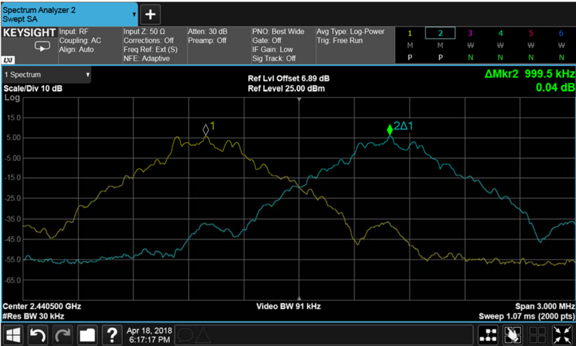
Figure 9 - GFSK
