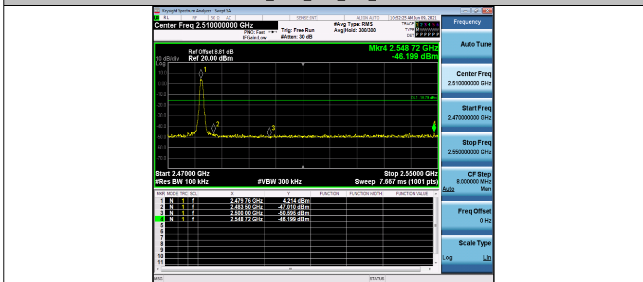
BLE_500K_Ant1_High_2480
