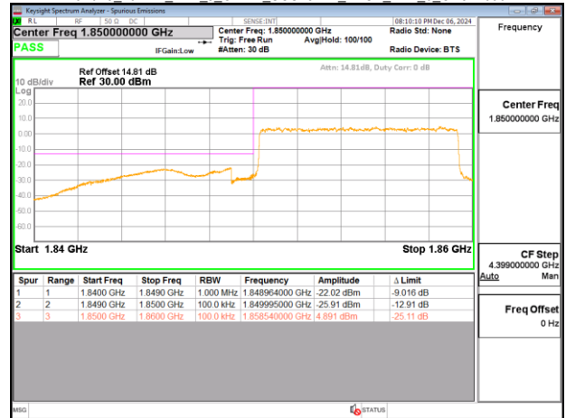
Band25_10MHz_DFT_s_OFDM_SCS15kHz_BPSK_RB50_0_CH371000
