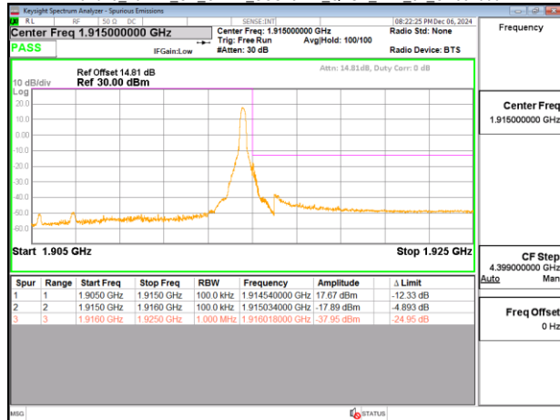
Band25_10MHz_CP_OFDM_SCS15kHz_QPSK_RB52_0_CH382000
