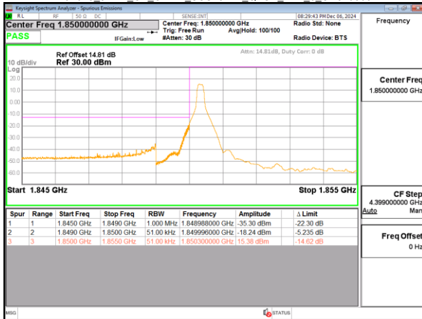
Band25_5MHz_CP_OFDM_SCS15kHz_QPSK_RB25_0_CH370500
