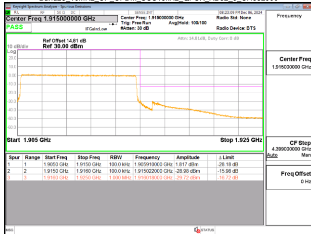
Band25_10MHz_CP_OFDM_SCS15kHz_QPSK_RB52_0_CH382000
