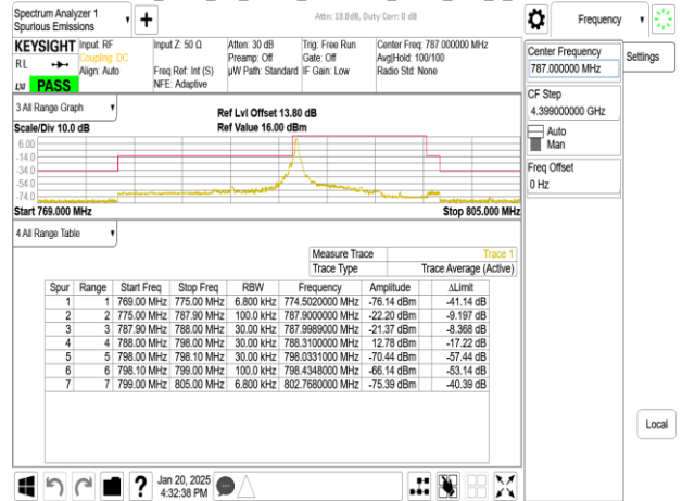
Band14_5MHz_CP_OFDM_SCS15kHz_QPSK_RB25_0_CH158100
