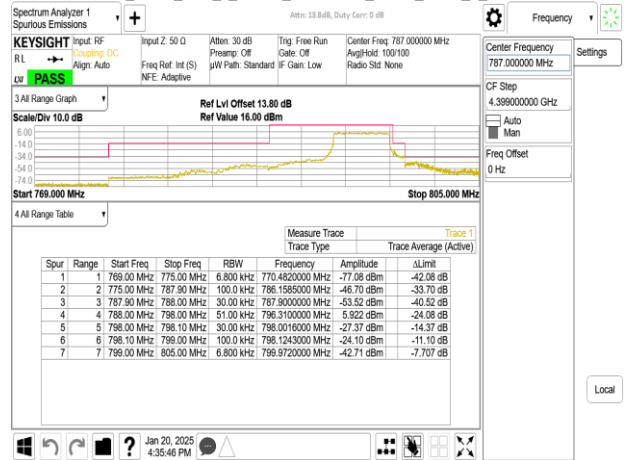
Band14_5MHz_CP_OFDM_SCS15kHz_QPSK_RB1_0_CH158100
