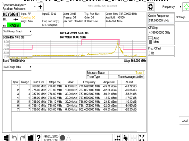
Band14_10MHz_CP_OFDM_SCS15kHz_QPSK_RB2_0_CH158600
