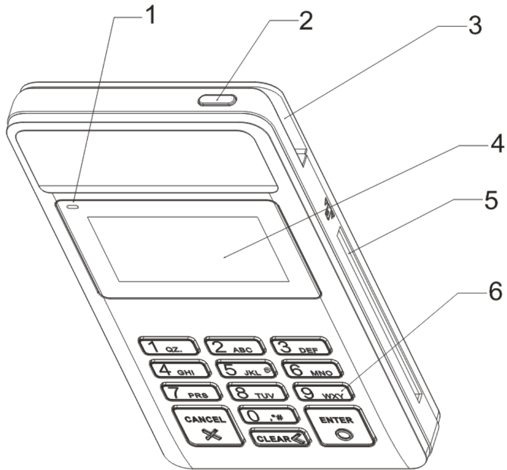
Figure 1. Front view
