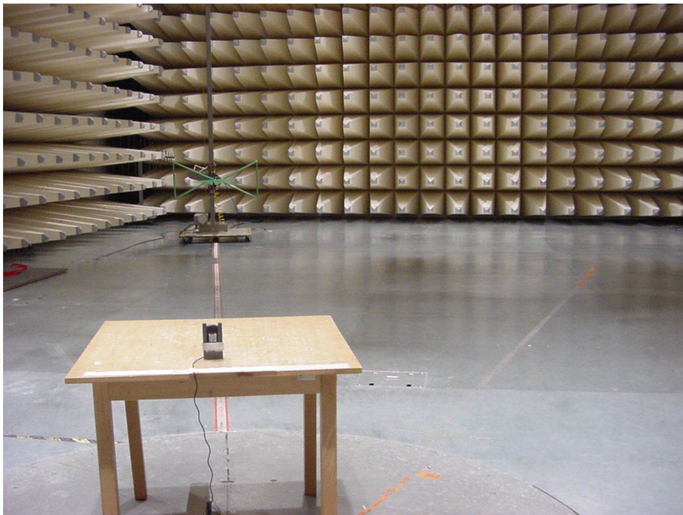
Photo 2 (Radiated Emissions):
