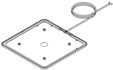
Deactivator Antenna 265 x 265 (cable length 1600 mm)
