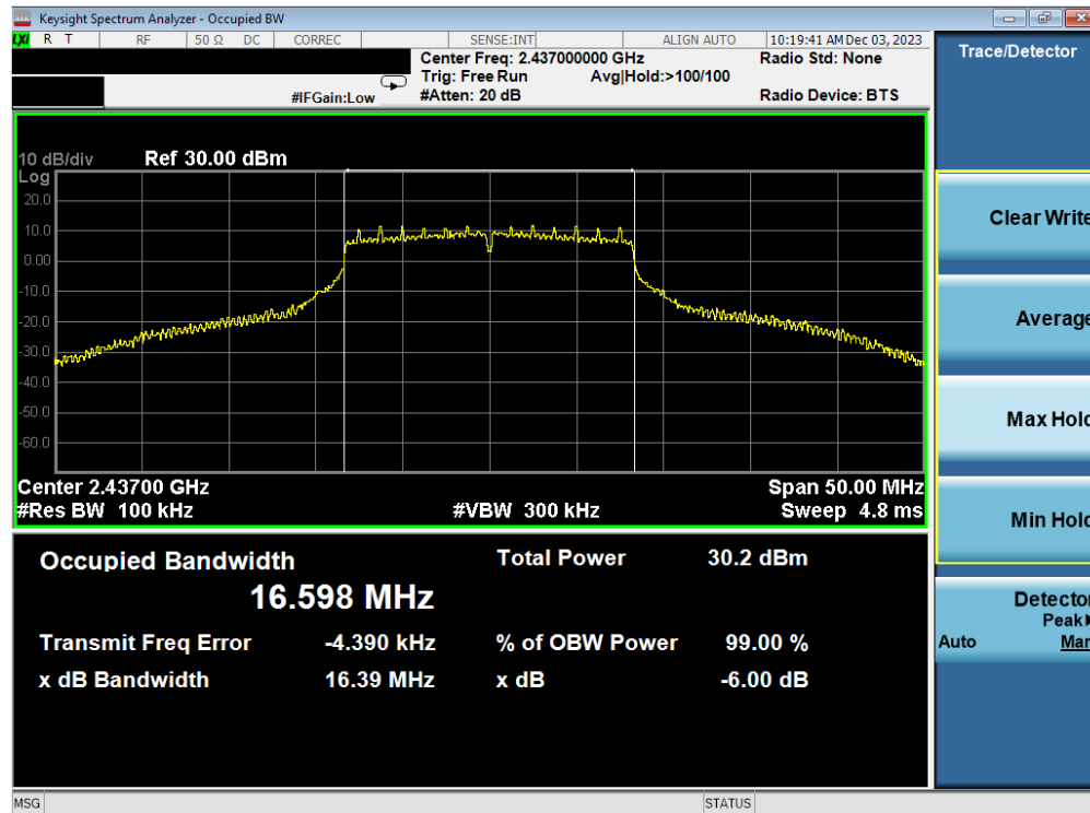
Plot 7-2. 6 dB BW and 99% OBW Plot Antenna WF7b (802.11g – Ch. 6) – 12Mbps
