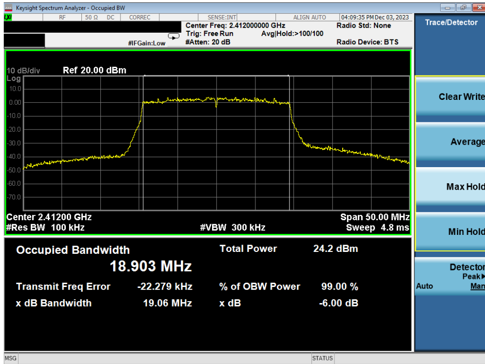
Plot 7-46. 6 dB BW and 99% OBW Plot Antenna WF2b (802.11ax(SU) - (2.4GHz) – Ch. 1) – MCS4
