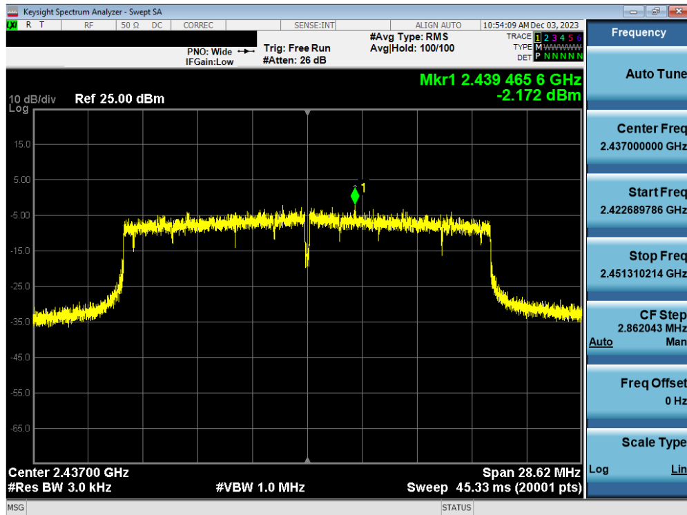
Plot 7-77. Power Spectral Density Plot Antenna WF7b (802.11ax(SU) - (2.4GHz) – Ch. 6) – MCS4
