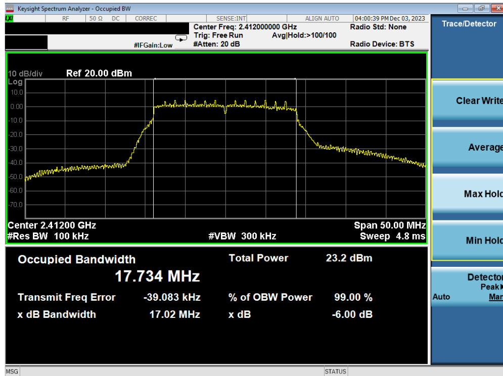
Plot 7-34. 6 dB BW and 99% OBW Plot Antenna WF2b (802.11n (2.4GHz) – Ch. 1) – MCS2
