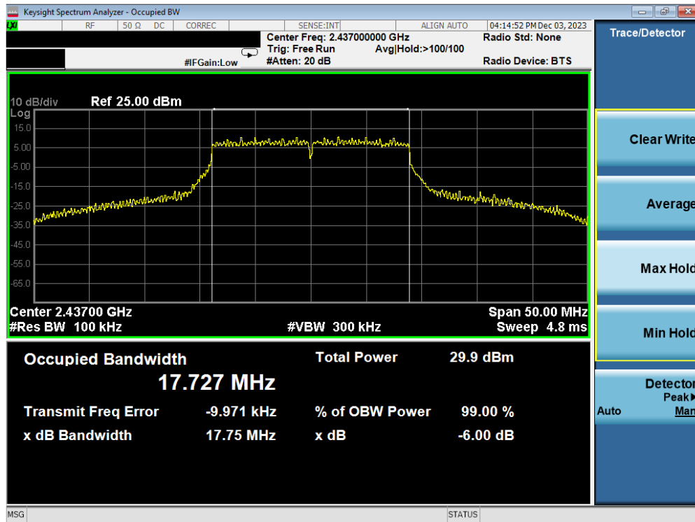
Plot 7-56. 6 dB BW and 99% OBW Plot Antenna WF2b (802.11n (2.4GHz) – Ch. 6) – MCS7
