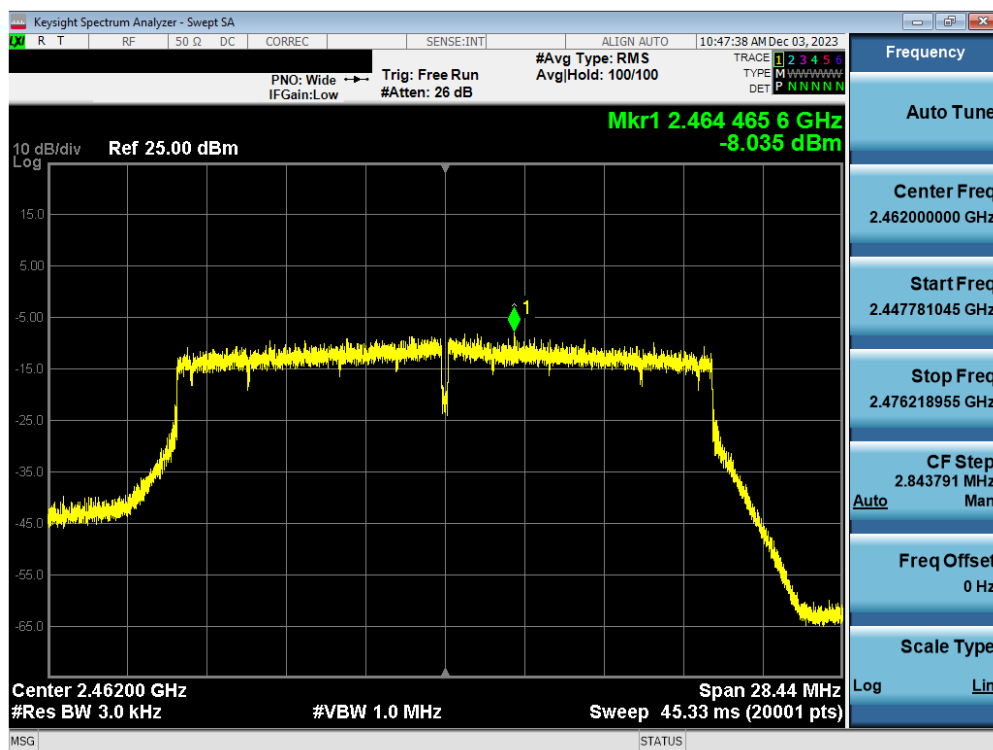
Plot 7-69. Power Spectral Density Plot Antenna WF7b (802.11ax(SU) - (2.4GHz) – Ch. 11) – MCS2
