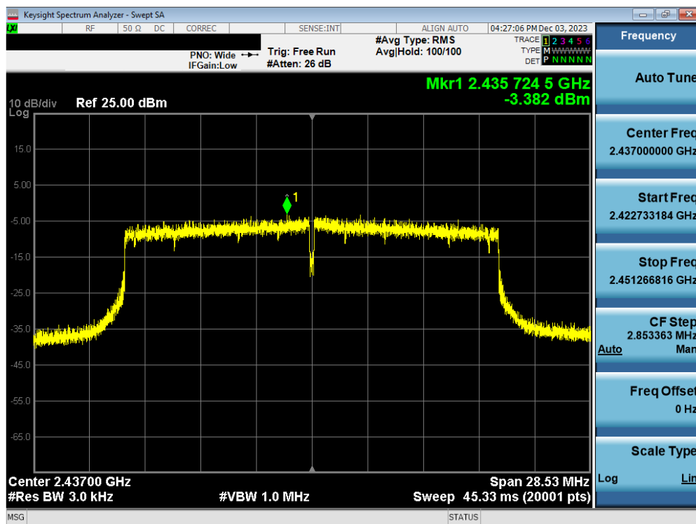
Plot 7-98. Power Spectral Density Plot Antenna WF2b (802.11ax(SU) - (2.4GHz) – Ch. 6) – MCS2
