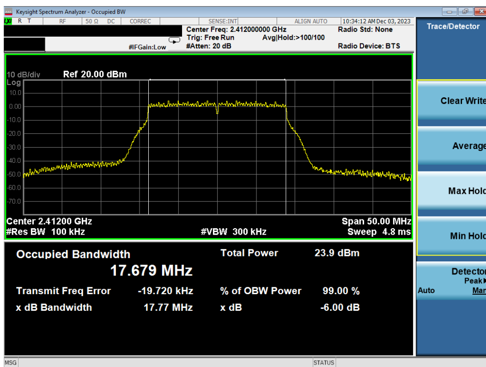
Plot 7-25. 6 dB BW and 99% OBW Plot Antenna WF7b (802.11n (2.4GHz) – Ch. 1) – MCS7
