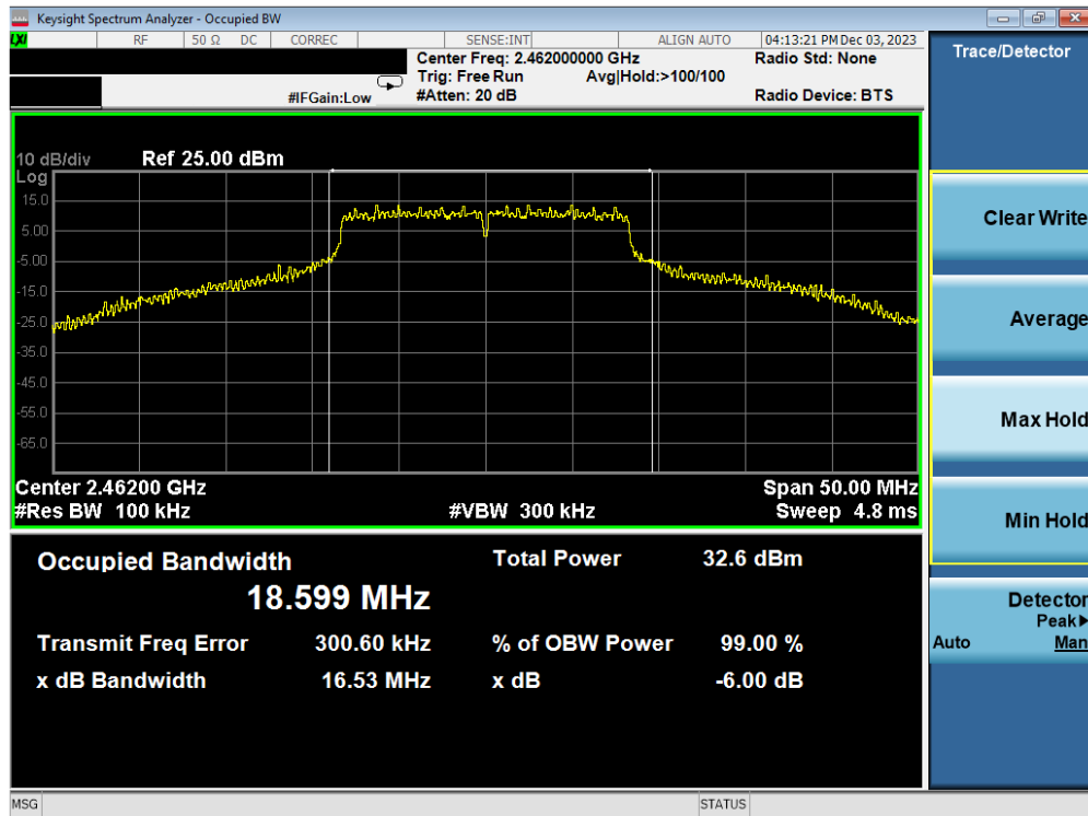
Plot 7-54. 6 dB BW and 99% OBW Plot Antenna WF2b (802.11g – Ch. 11) – 54Mbps
