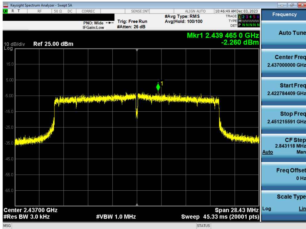
Plot 7-68. Power Spectral Density Plot Antenna WF7b (802.11ax(SU) - (2.4GHz) – Ch. 6) – MCS2
