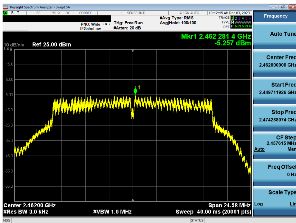
Plot 7-63. Power Spectral Density Plot Antenna WF7b (802.11g – Ch. 11) – 12Mbps
