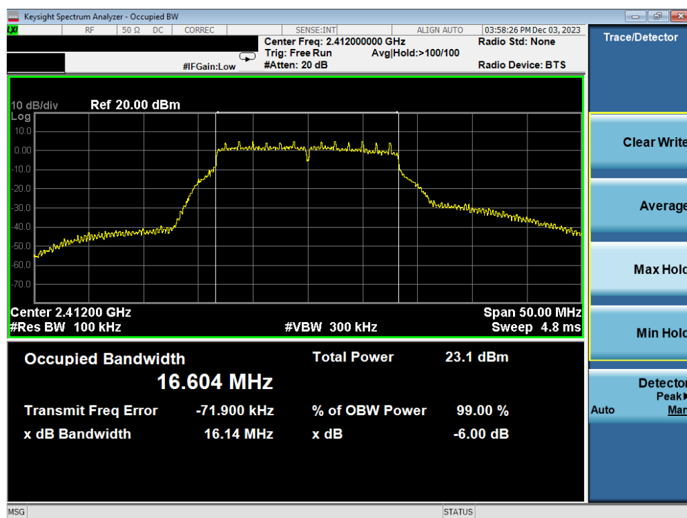
Plot 7-31. 6 dB BW and 99% OBW Plot Antenna WF2b (802.11g – Ch. 1) – 12Mbps
