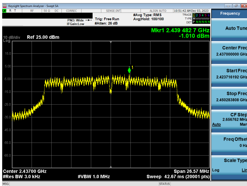
Plot 7-74. Power Spectral Density Plot Antenna WF7b (802.11n (2.4GHz) – Ch. 6) – MCS4
