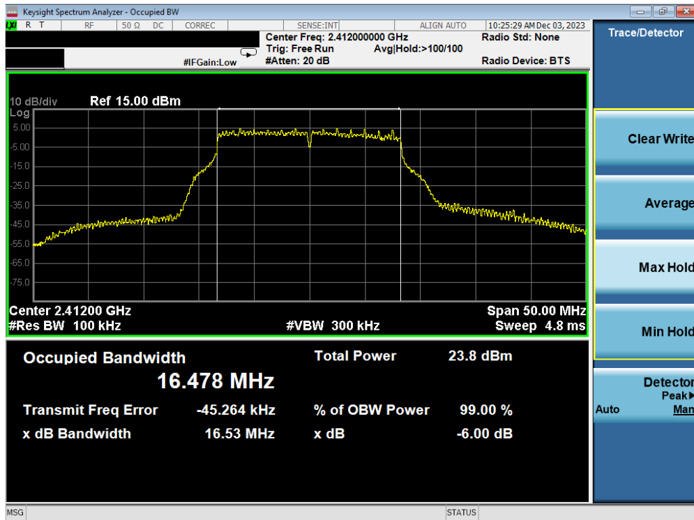
Plot 7-10. 6 dB BW and 99% OBW Plot Antenna WF7b (802.11g – Ch. 1) – 24Mbps
