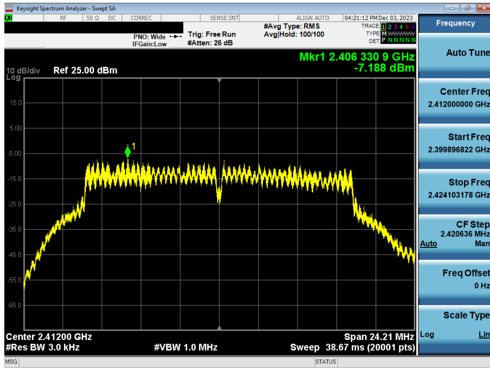
Plot 7-91. Power Spectral Density Plot Antenna WF2b (802.11g – Ch. 1) – 12Mbps
