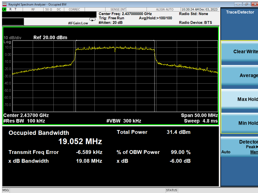
Plot 7-17. 6 dB BW and 99% OBW Plot Antenna WF7b (802.11ax(SU) - (2.4GHz) – Ch. 6) – MCS4
