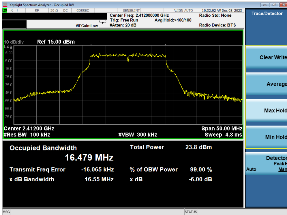
Plot 7-22. 6 dB BW and 99% OBW Plot Antenna WF7b (802.11g – Ch. 1) – 54Mbps
