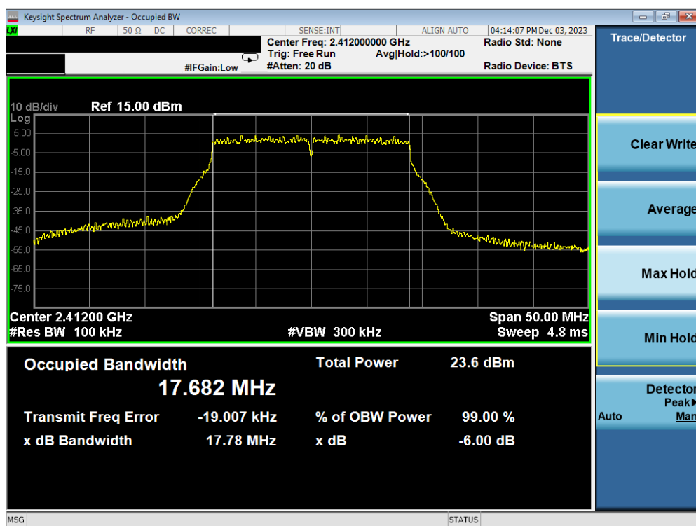
Plot 7-55. 6 dB BW and 99% OBW Plot Antenna WF2b (802.11n (2.4GHz) – Ch. 1) – MCS7
