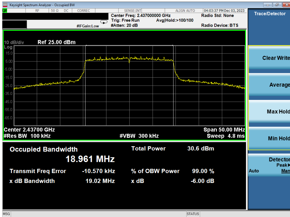
Plot 7-38. 6 dB BW and 99% OBW Plot Antenna WF2b (802.11ax(SU) - (2.4GHz) – Ch. 6) – MCS2
