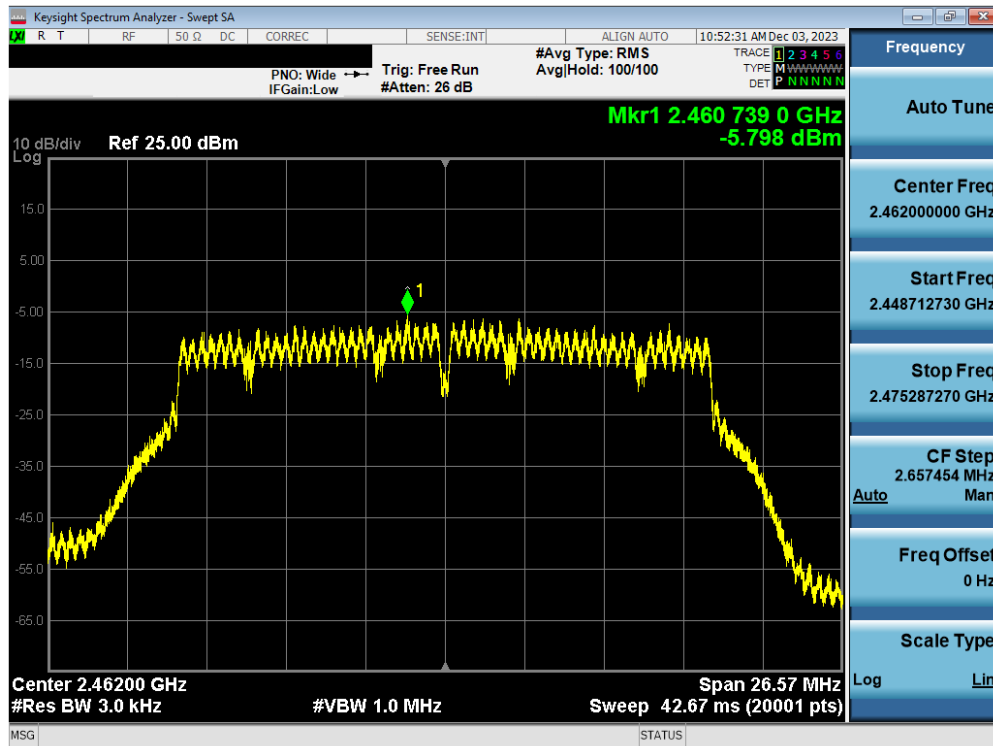
Plot 7-75. Power Spectral Density Plot Antenna WF7b (802.11n (2.4GHz) – Ch. 11) – MCS4
