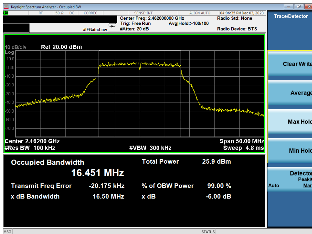
Plot 7-42. 6 dB BW and 99% OBW Plot Antenna WF2b (802.11g – Ch. 11) – 24Mbps
