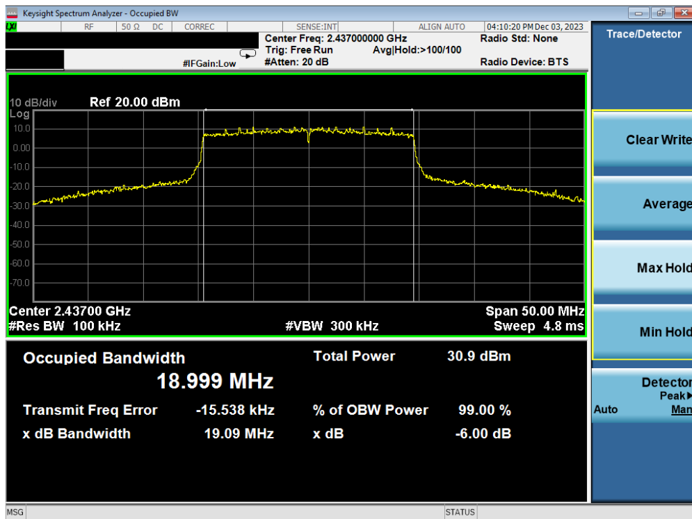
Plot 7-47. 6 dB BW and 99% OBW Plot Antenna WF2b (802.11ax(SU) - (2.4GHz) – Ch. 6) – MCS4
