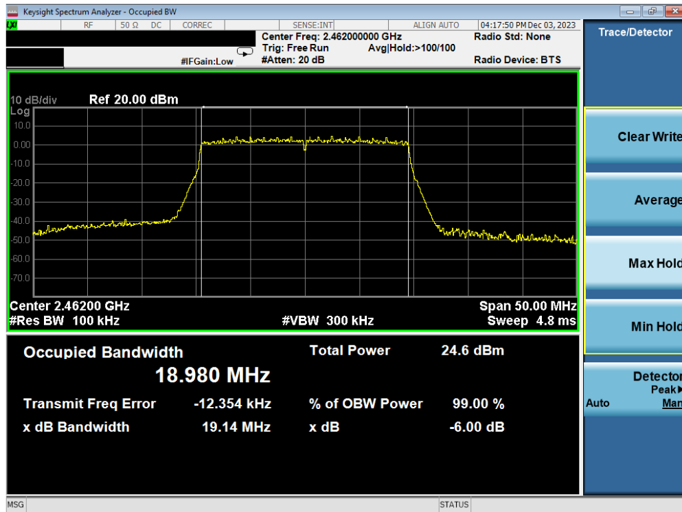
Plot 7-60. 6 dB BW and 99% OBW Plot Antenna WF2b (802.11ax(SU) - (2.4GHz) – Ch. 11) – MCS9
