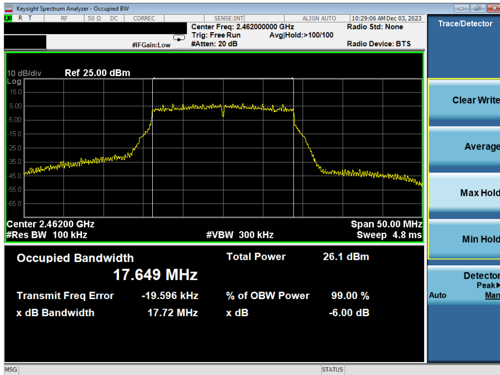
Plot 7-15. 6 dB BW and 99% OBW Plot Antenna WF7b (802.11n (2.4GHz) – Ch. 11) – MCS4
