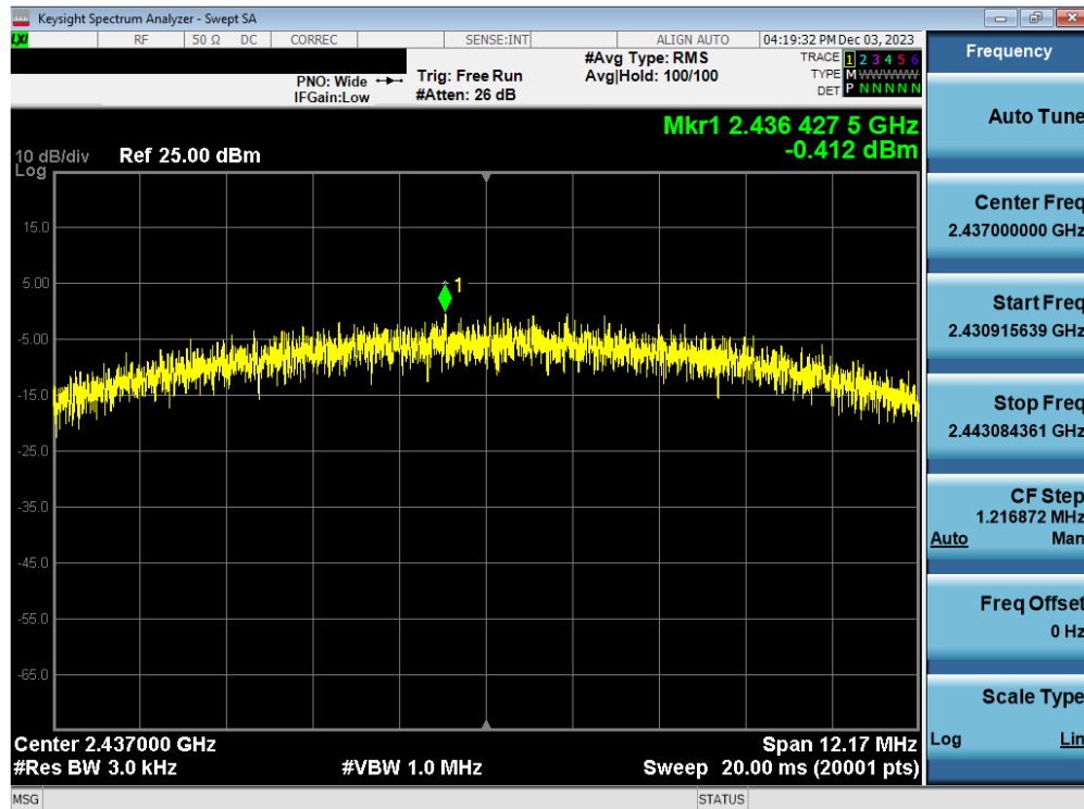
Plot 7-110. Power Spectral Density Plot Antenna WF2b (802.11b – Ch. 6) – 11Mbps
