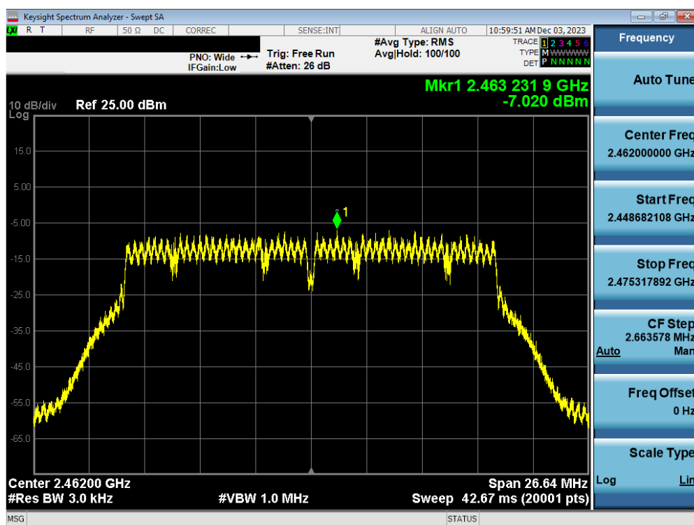
Plot 7-87. Power Spectral Density Plot Antenna WF7b (802.11n (2.4GHz) – Ch. 11) – MCS7
