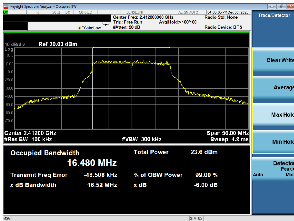
Plot 7-40. 6 dB BW and 99% OBW Plot Antenna WF2b (802.11g – Ch. 1) – 24Mbps
