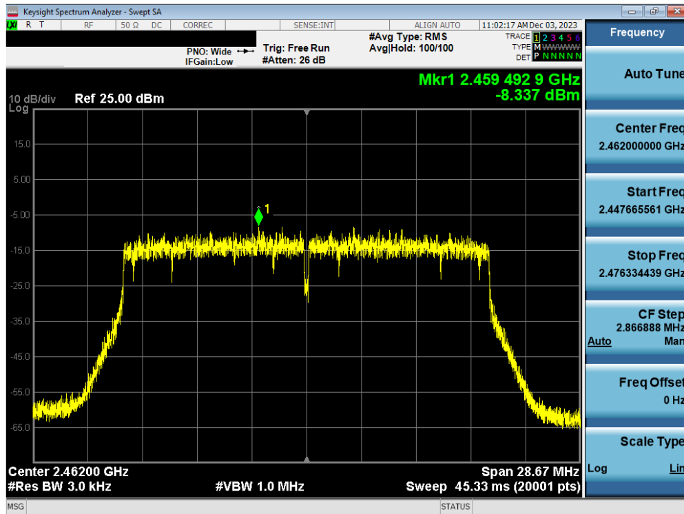
Plot 7-90. Power Spectral Density Plot Antenna WF7b (802.11ax(SU) - (2.4GHz) – Ch. 11) – MCS9
