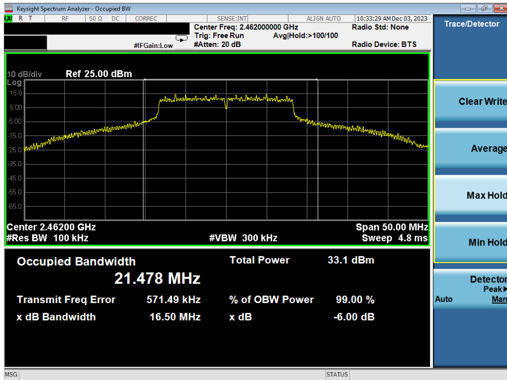
Plot 7-24. 6 dB BW and 99% OBW Plot Antenna WF7b (802.11g – Ch. 11) – 54Mbps
