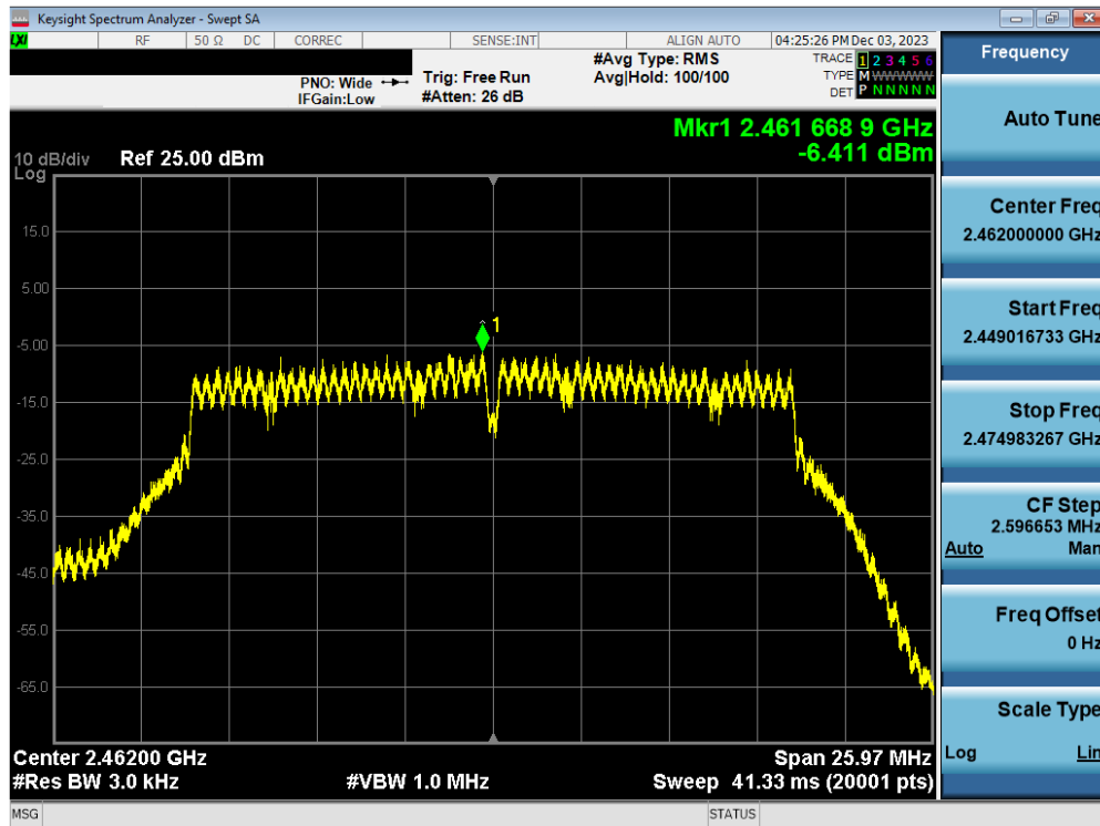
Plot 7-96. Power Spectral Density Plot Antenna WF2b (802.11n (2.4GHz) – Ch. 11) – MCS2
