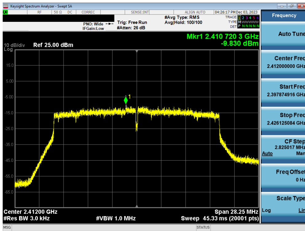
Plot 7-97. Power Spectral Density Plot Antenna WF2b (802.11ax(SU) - (2.4GHz) – Ch. 1) – MCS2
