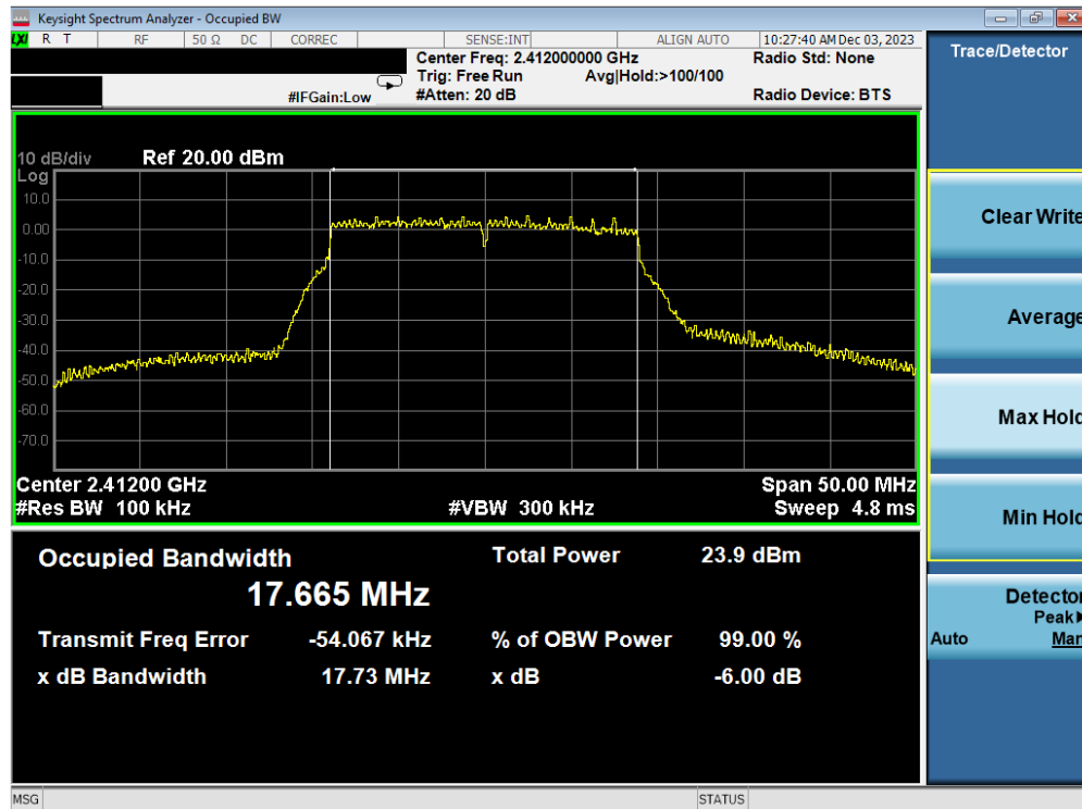
Plot 7-13. 6 dB BW and 99% OBW Plot Antenna WF7b (802.11n (2.4GHz) – Ch. 1) – MCS4
