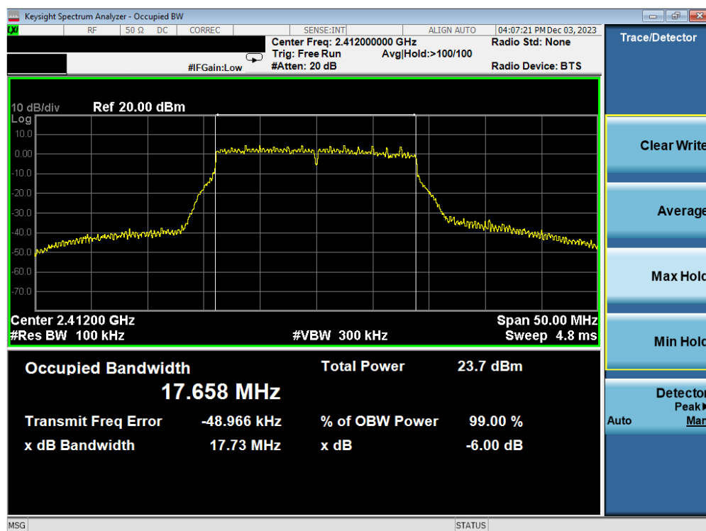
Plot 7-43. 6 dB BW and 99% OBW Plot Antenna WF2b (802.11n (2.4GHz) – Ch. 1) – MCS4
