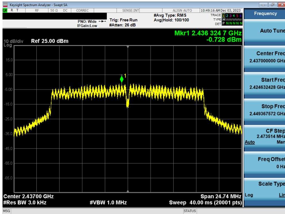
Plot 7-71. Power Spectral Density Plot Antenna WF7b (802.11g – Ch. 6) – 24Mbps
