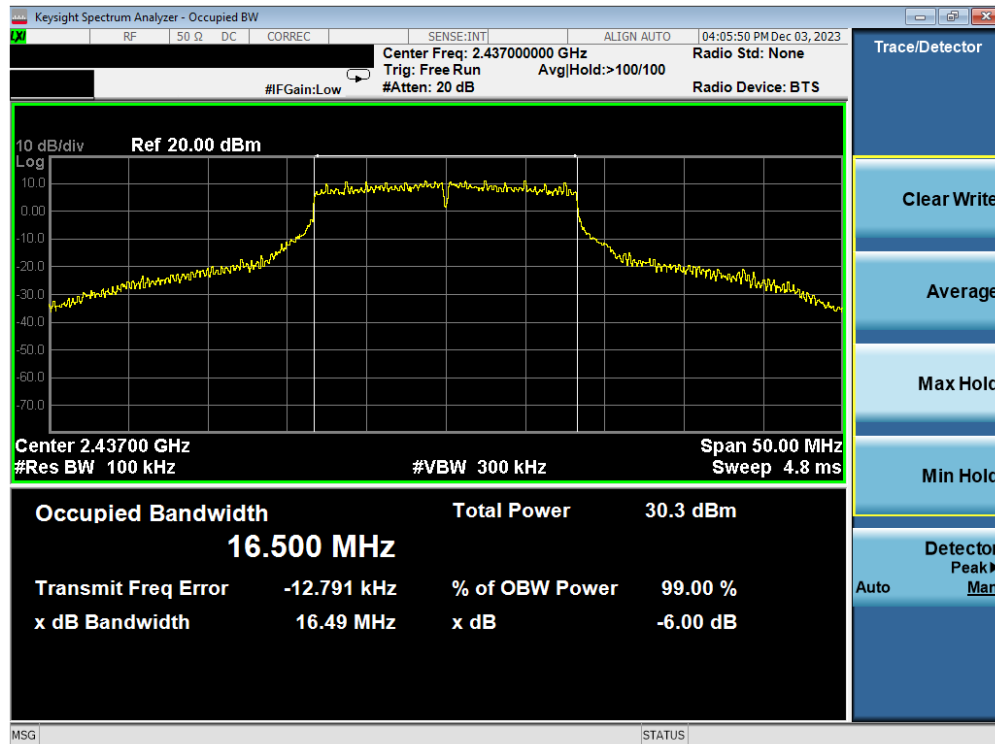
Plot 7-41. 6 dB BW and 99% OBW Plot Antenna WF2b (802.11g – Ch. 6) – 24Mbps
