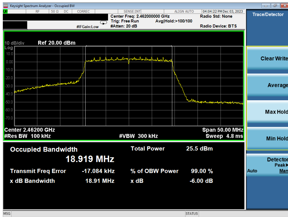
Plot 7-39. 6 dB BW and 99% OBW Plot Antenna WF2b (802.11ax(SU) - (2.4GHz) – Ch. 11) – MCS2
