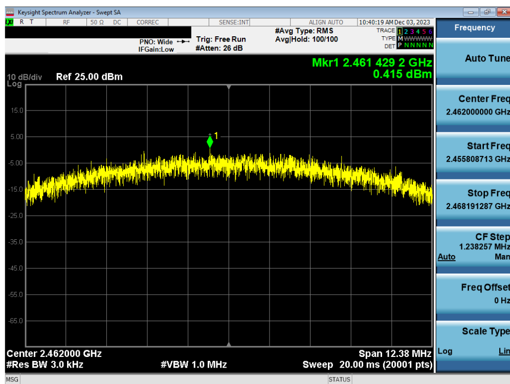
Plot 7-81. Power Spectral Density Plot Antenna WF7b (802.11b – Ch. 11) – 11Mbps
