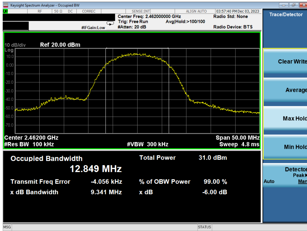
Plot 7-51. 6 dB BW and 99% OBW Plot Antenna WF2b (802.11b – Ch. 11) – 11Mbps
