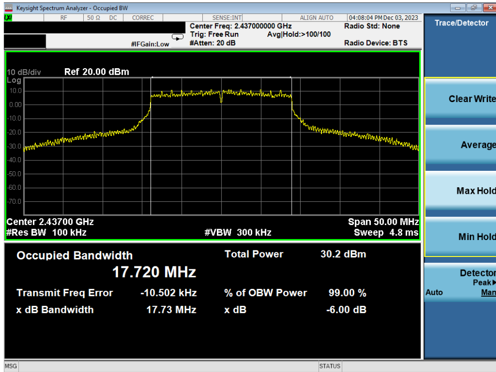
Plot 7-44. 6 dB BW and 99% OBW Plot Antenna WF2b (802.11n (2.4GHz) – Ch. 6) – MCS4
