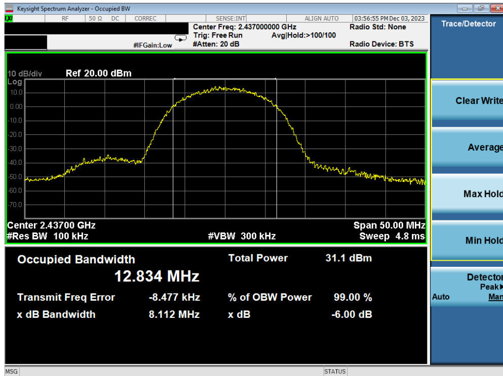
Plot 7-50. 6 dB BW and 99% OBW Plot Antenna WF2b (802.11b – Ch. 6) – 11Mbps
