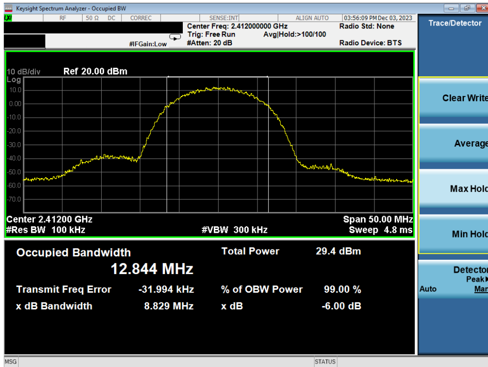
Plot 7-49. 6 dB BW and 99% OBW Plot Antenna WF2b (802.11b – Ch. 1) – 11Mbps
