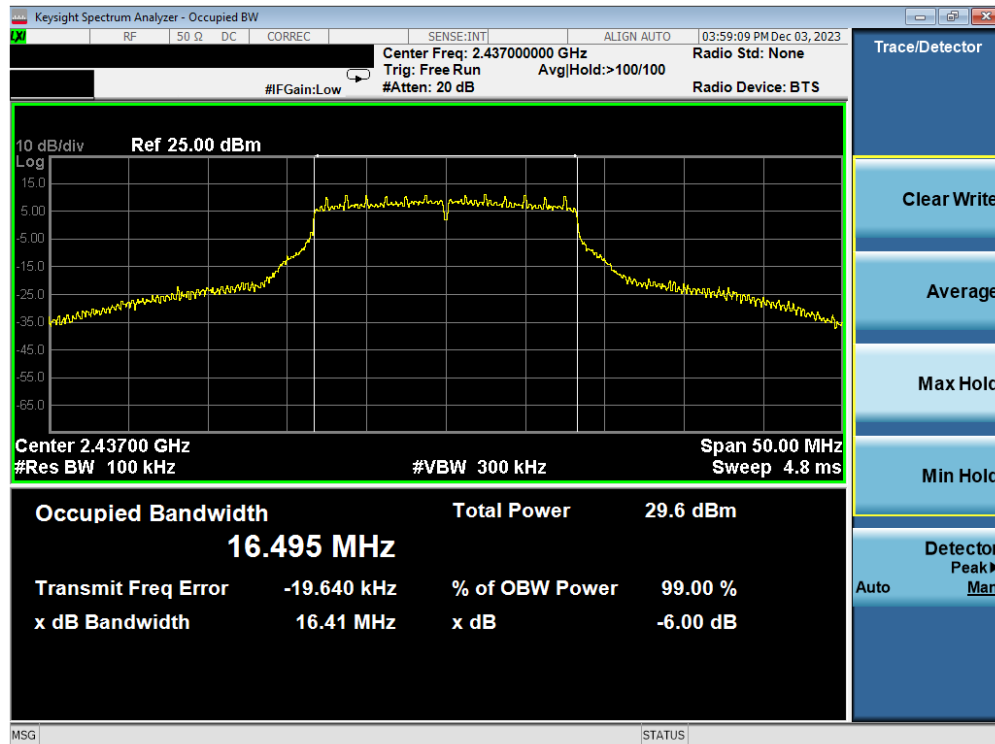
Plot 7-32. 6 dB BW and 99% OBW Plot Antenna WF2b (802.11g – Ch. 6) – 12Mbps
