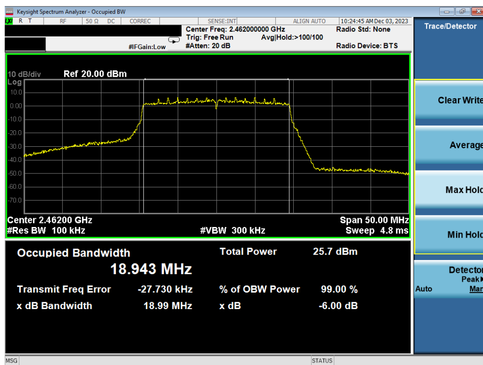
Plot 7-9. 6 dB BW and 99% OBW Plot Antenna WF7b (802.11ax(SU) - (2.4GHz) – Ch. 11) – MCS2
