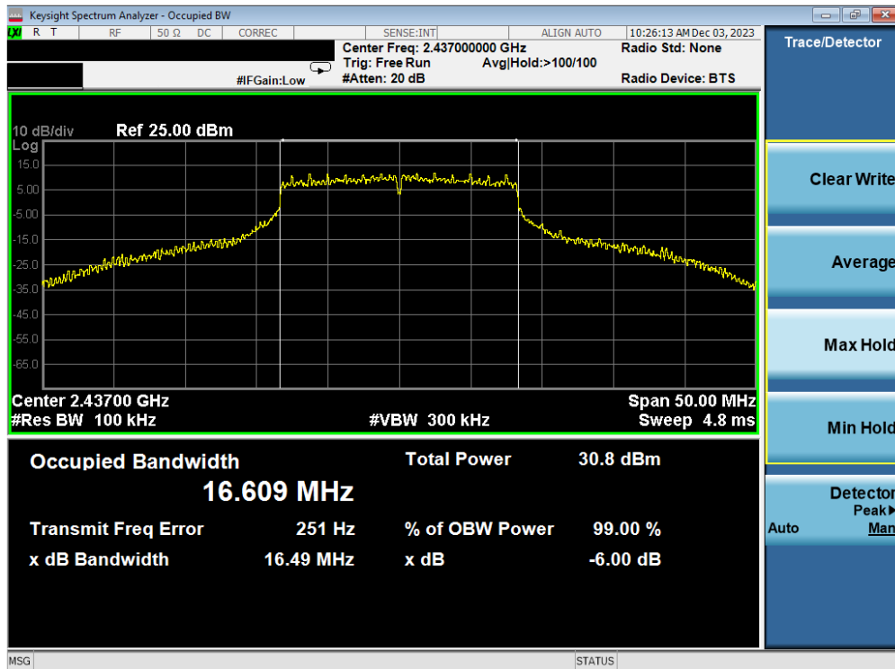
Plot 7-11. 6 dB BW and 99% OBW Plot Antenna WF7b (802.11g – Ch. 6) – 24Mbps
