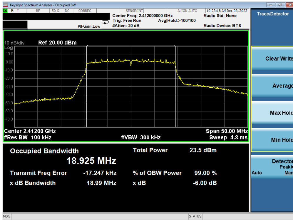
Plot 7-7. 6 dB BW and 99% OBW Plot Antenna WF7b (802.11ax(SU) - (2.4GHz) – Ch. 1) – MCS2
