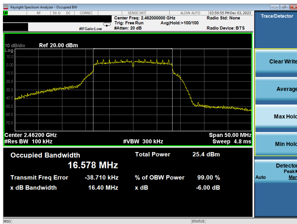
Plot 7-33. 6 dB BW and 99% OBW Plot Antenna WF2b (802.11g – Ch. 11) – 12Mbps
