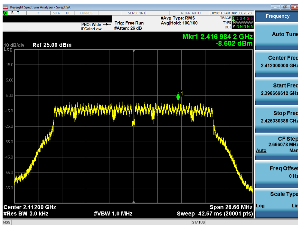
Plot 7-85. Power Spectral Density Plot Antenna WF7b (802.11n (2.4GHz) – Ch. 1) – MCS7
