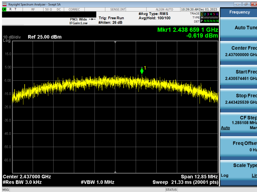
Plot 7-80. Power Spectral Density Plot Antenna WF7b (802.11b – Ch. 6) – 11Mbps
