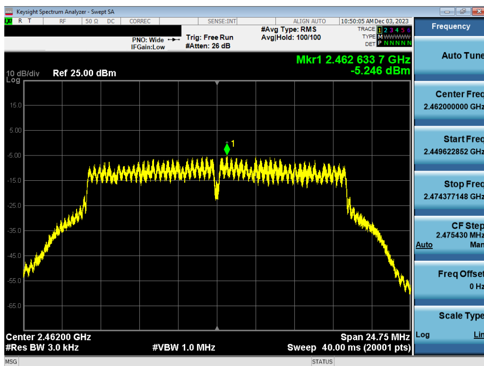
Plot 7-72. Power Spectral Density Plot Antenna WF7b (802.11g – Ch. 11) – 24Mbps
