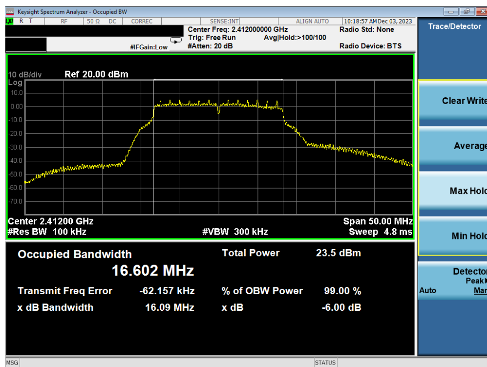
Plot 7-1. 6 dB BW and 99% OBW Plot Antenna WF7b (802.11g – Ch. 1) – 12Mbps
