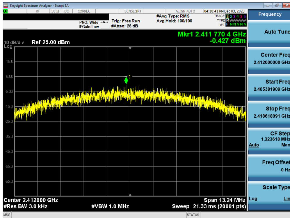
Plot 7-109. Power Spectral Density Plot Antenna WF2b (802.11b – Ch. 1) – 11Mbps
