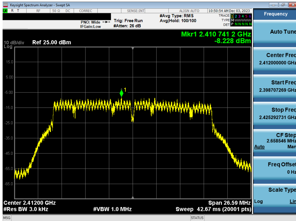
Plot 7-73. Power Spectral Density Plot Antenna WF7b (802.11n (2.4GHz) – Ch. 1) – MCS4
