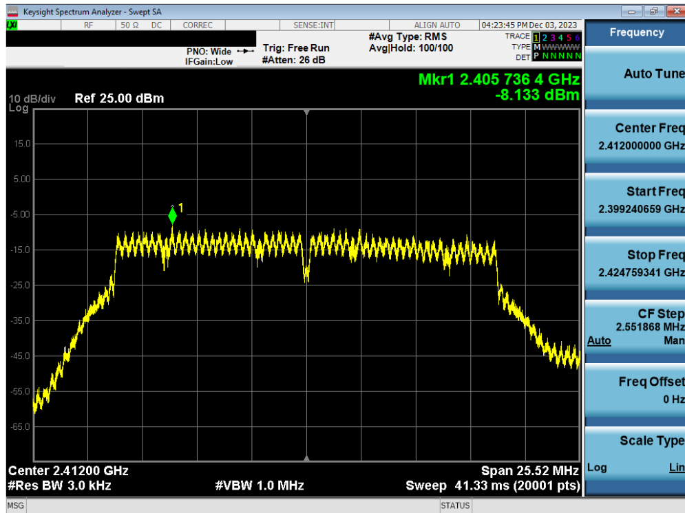
Plot 7-94. Power Spectral Density Plot Antenna WF2b (802.11n (2.4GHz) – Ch. 1) – MCS2
