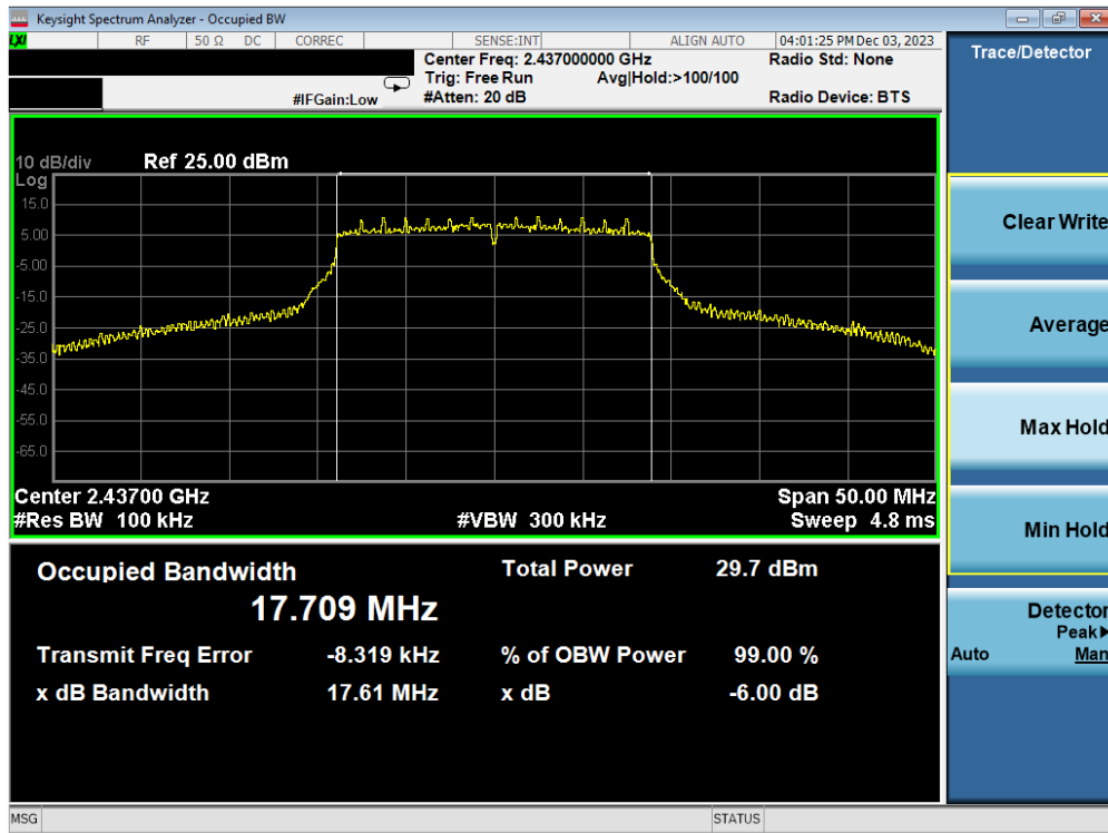
Plot 7-35. 6 dB BW and 99% OBW Plot Antenna WF2b (802.11n (2.4GHz) – Ch. 6) – MCS2
