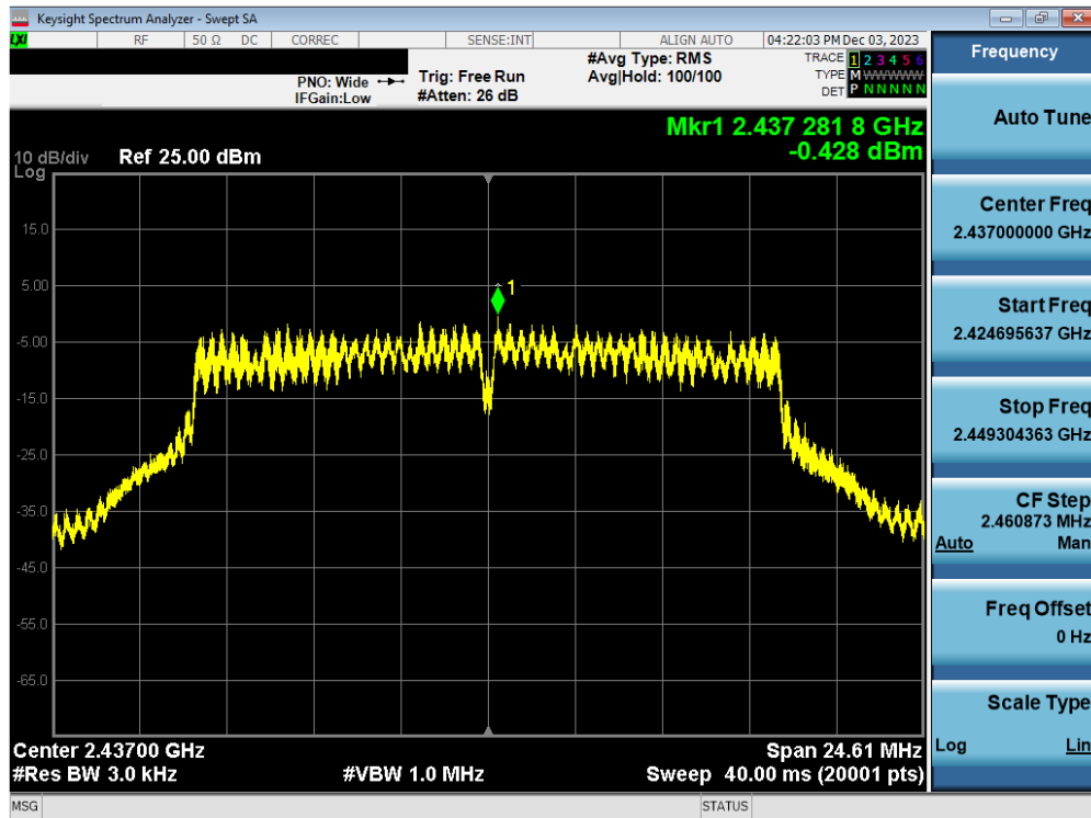
Plot 7-92. Power Spectral Density Plot Antenna WF2b (802.11g – Ch. 6) – 12Mbps
