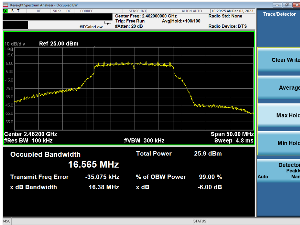
Plot 7-3. 6 dB BW and 99% OBW Plot Antenna WF7b (802.11g – Ch. 11) – 12Mbps
