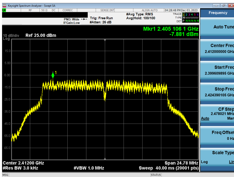
Plot 7-100. Power Spectral Density Plot Antenna WF2b (802.11g – Ch. 1) – 24Mbps
