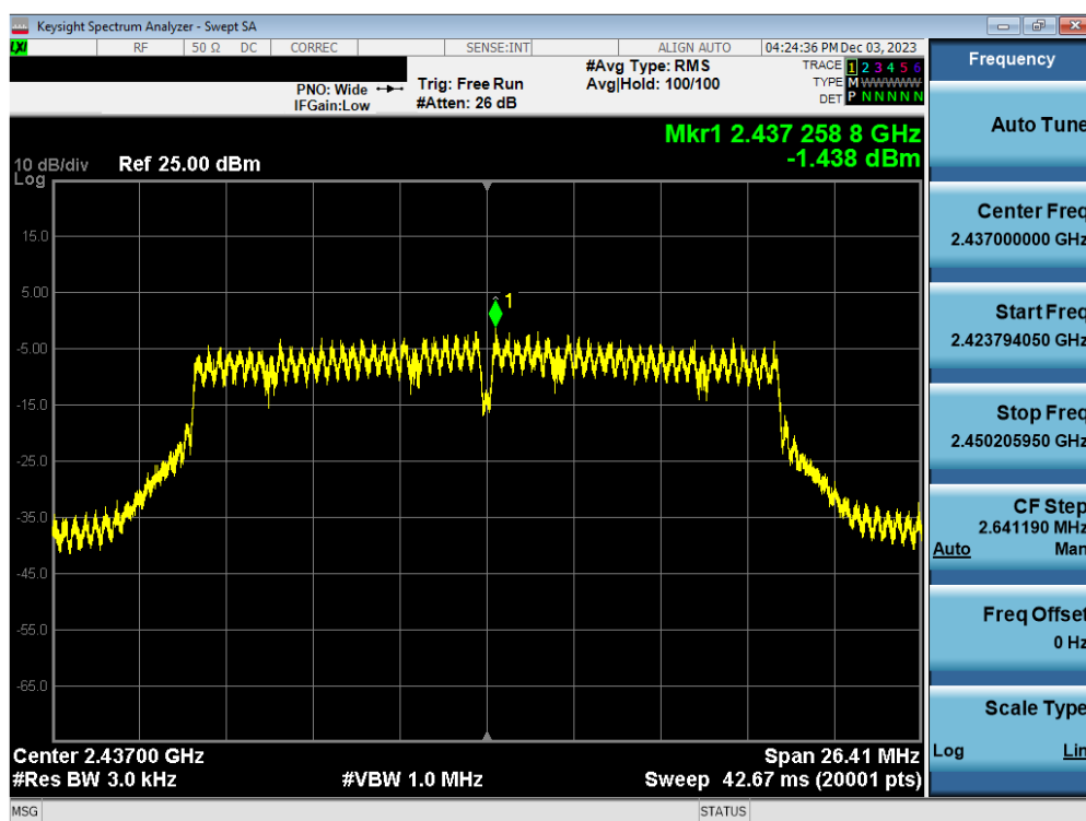
Plot 7-95. Power Spectral Density Plot Antenna WF2b (802.11n (2.4GHz) – Ch. 6) – MCS2
