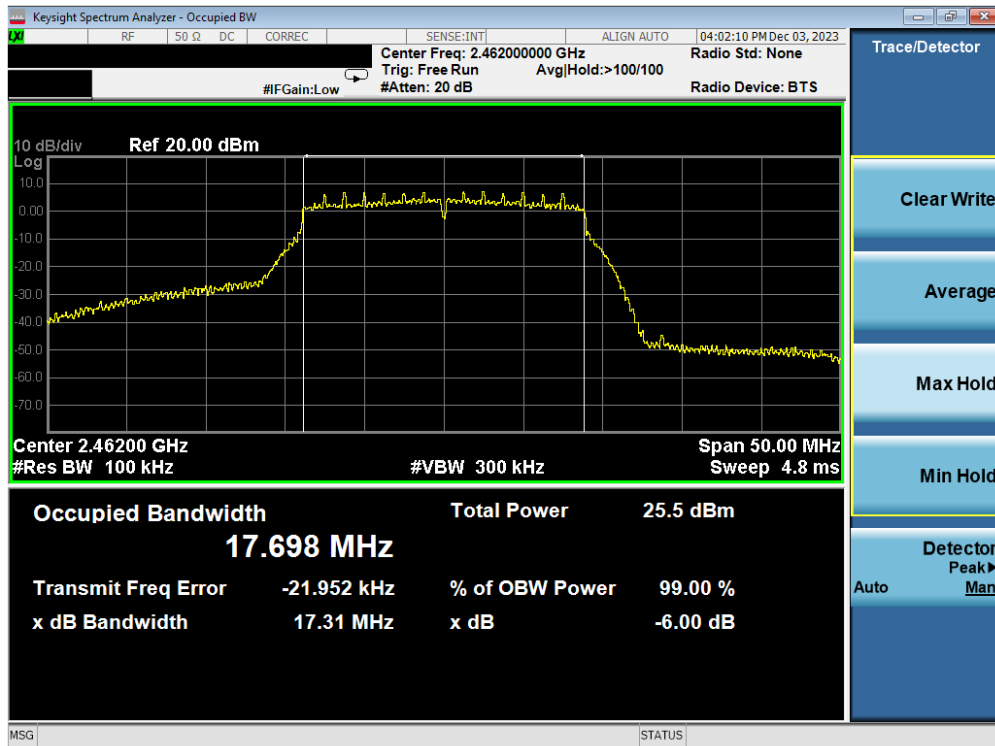
Plot 7-36. 6 dB BW and 99% OBW Plot Antenna WF2b (802.11n (2.4GHz) – Ch. 11) – MCS2
