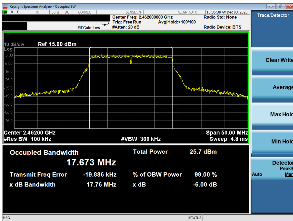
Plot 7-27. 6 dB BW and 99% OBW Plot Antenna WF7b (802.11n (2.4GHz) – Ch. 11) – MCS7
