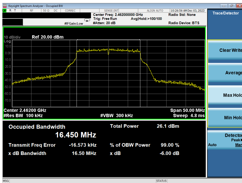
Plot 7-12. 6 dB BW and 99% OBW Plot Antenna WF7b (802.11g – Ch. 11) – 24Mbps
