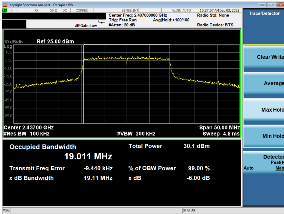
Plot 7-29. 6 dB BW and 99% OBW Plot Antenna WF7b (802.11ax(SU) - (2.4GHz) – Ch. 6) – MCS9
