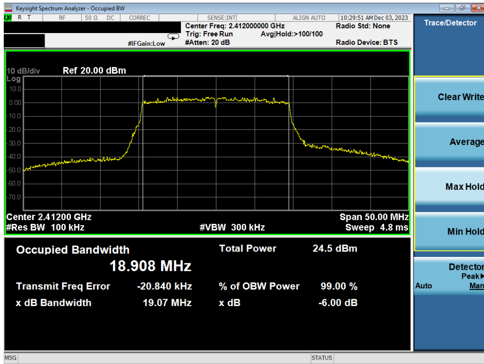
Plot 7-16. 6 dB BW and 99% OBW Plot Antenna WF7b (802.11ax(SU) - (2.4GHz) – Ch. 1) – MCS4
