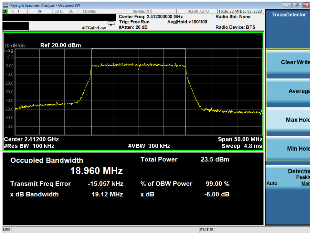
Plot 7-28. 6 dB BW and 99% OBW Plot Antenna WF7b (802.11ax(SU) - (2.4GHz) – Ch. 1) – MCS9
