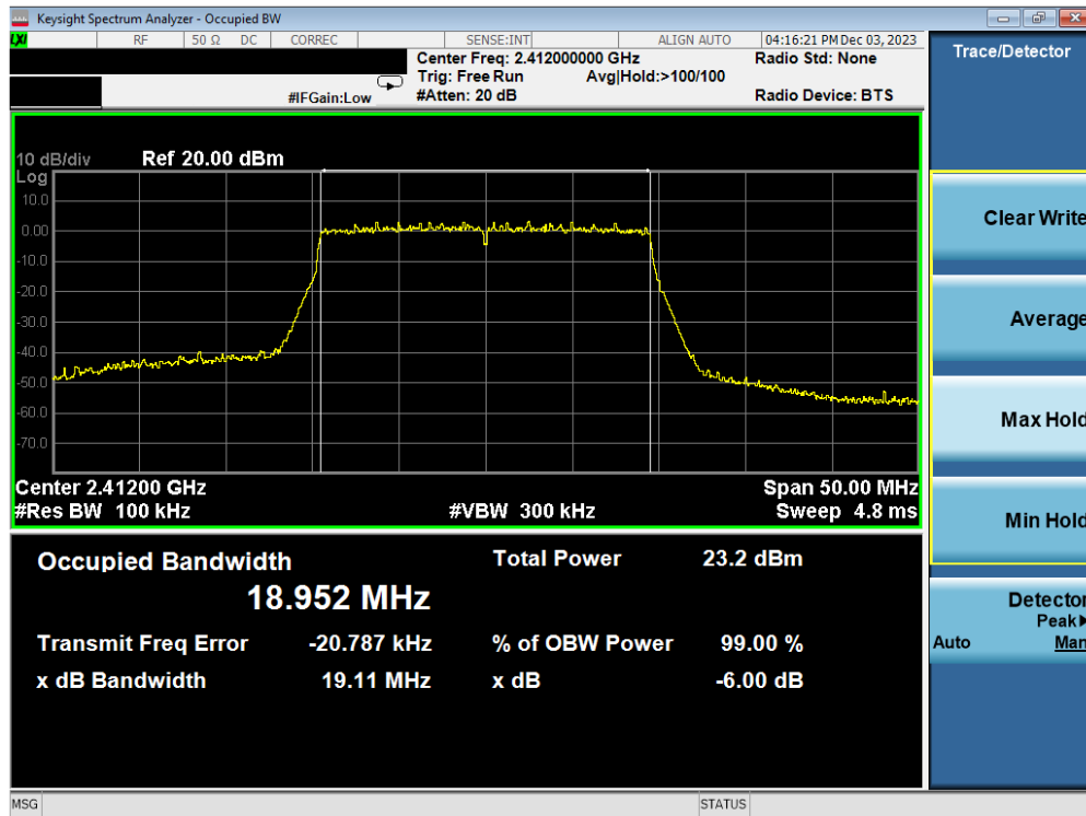
Plot 7-58. 6 dB BW and 99% OBW Plot Antenna WF2b (802.11ax(SU) - (2.4GHz) – Ch. 1) – MCS9
