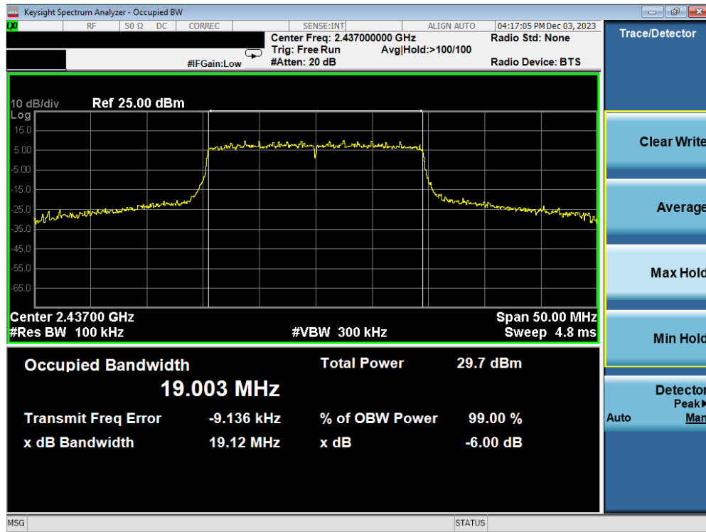
Plot 7-59. 6 dB BW and 99% OBW Plot Antenna WF2b (802.11ax(SU) - (2.4GHz) – Ch. 6) – MCS9
