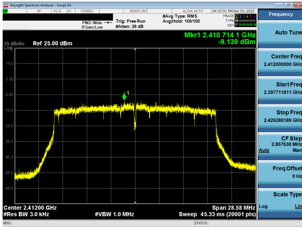
Plot 7-106. Power Spectral Density Plot Antenna WF2b (802.11ax(SU)) - (2.4GHz) – Ch. 1) – MCS4
