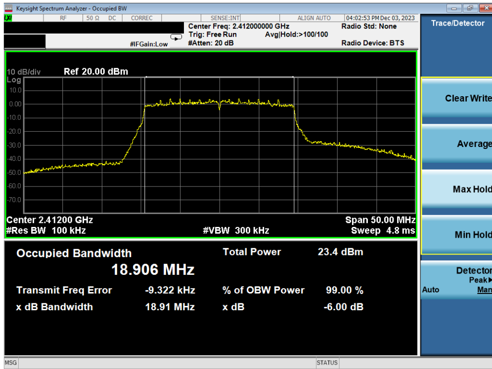
Plot 7-37. 6 dB BW and 99% OBW Plot Antenna WF2b (802.11ax(SU) - (2.4GHz) – Ch. 1) – MCS2
