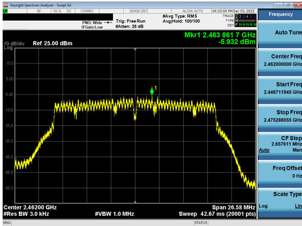
Plot 7-105. Power Spectral Density Plot Antenna WF2b (802.11n (2.4GHz) – Ch. 11) – MCS4
