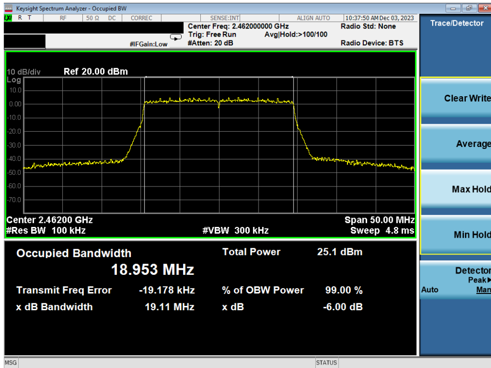
Plot 7-30. 6 dB BW and 99% OBW Plot Antenna WF7b (802.11ax(SU) - (2.4GHz) – Ch. 11) – MCS9
