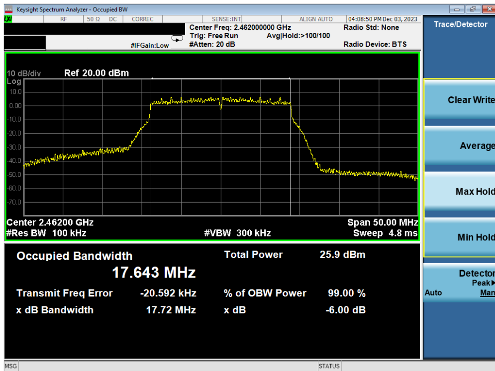
Plot 7-45. 6 dB BW and 99% OBW Plot Antenna WF2b (802.11n (2.4GHz) – Ch. 11) – MCS4
