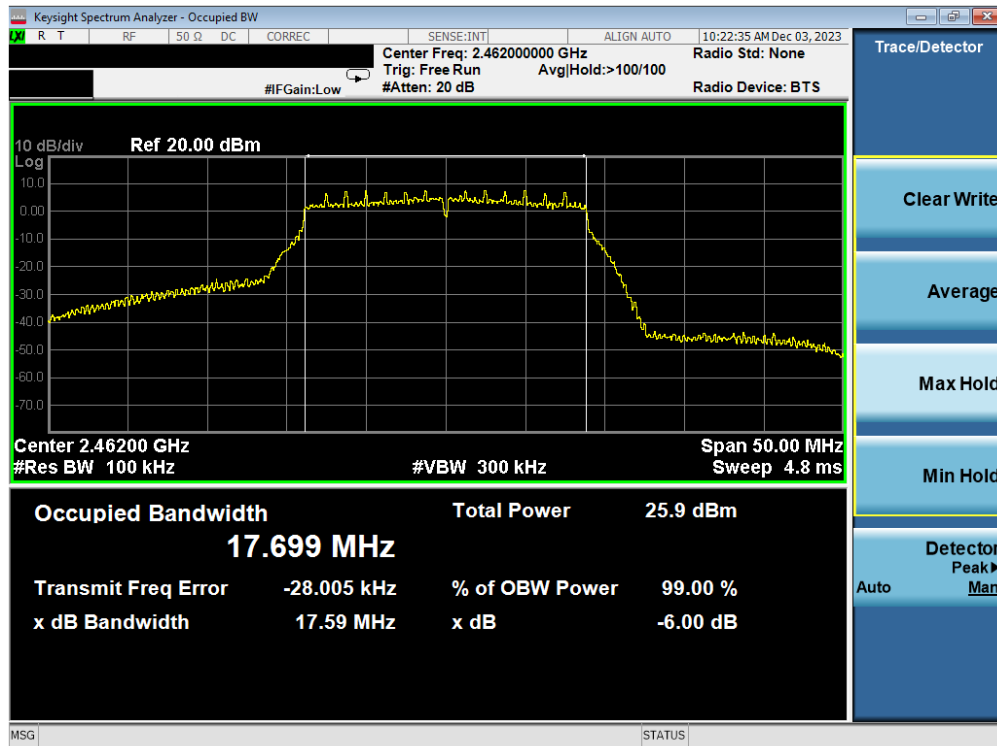
Plot 7-6. 6 dB BW and 99% OBW Plot Antenna WF7b (802.11n (2.4GHz) – Ch. 11) – MCS2
