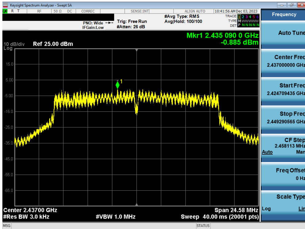
Plot 7-62. Power Spectral Density Plot Antenna WF7b (802.11g – Ch. 6) – 12Mbps
