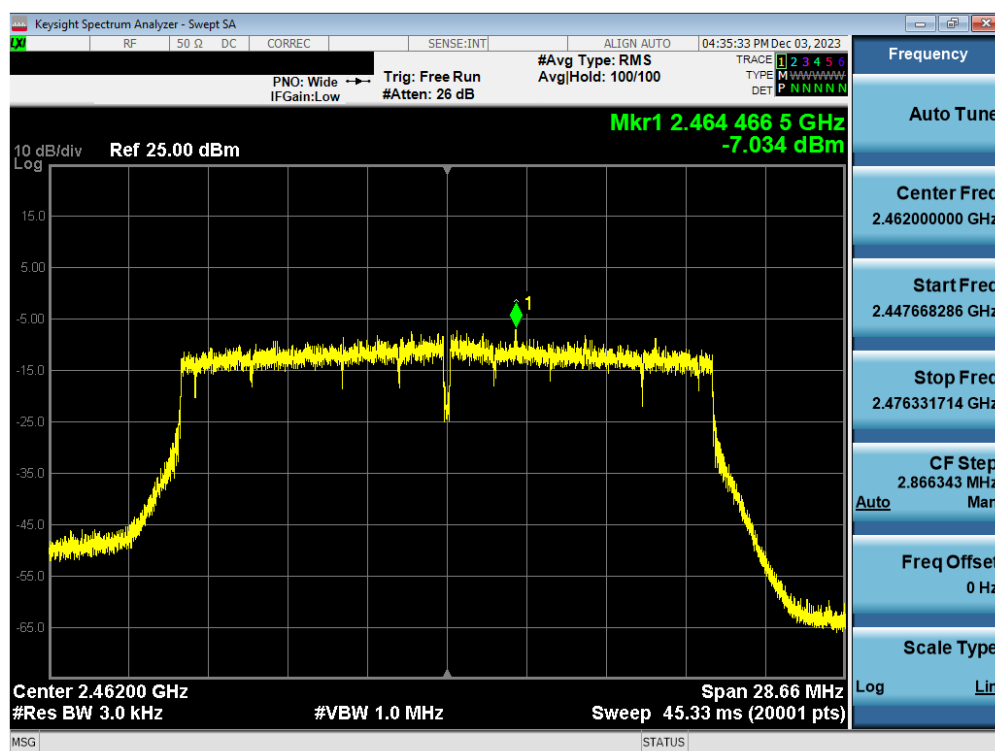
Plot 7-108. Power Spectral Density Plot Antenna WF2b (802.11ax(SU) - (2.4GHz) – Ch. 11) – MCS4
