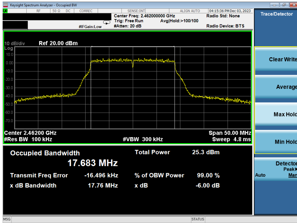
Plot 7-57. 6 dB BW and 99% OBW Plot Antenna WF2b (802.11n (2.4GHz) – Ch. 11) – MCS7
