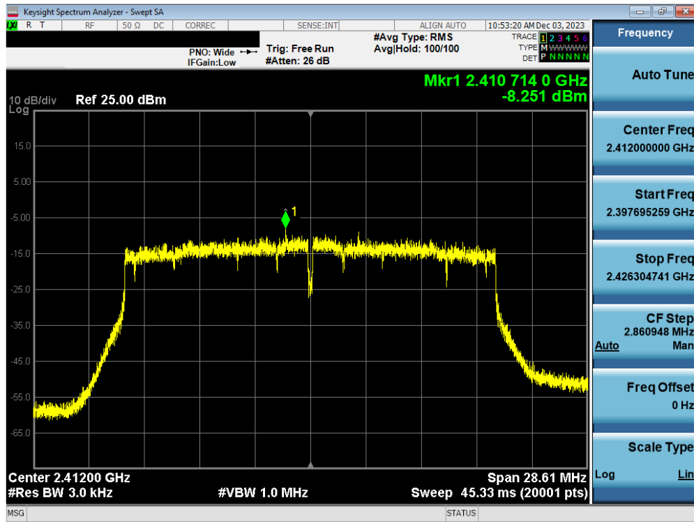
Plot 7-76. Power Spectral Density Plot Antenna WF7b (802.11ax(SU) - (2.4GHz) – Ch. 1) – MCS4
