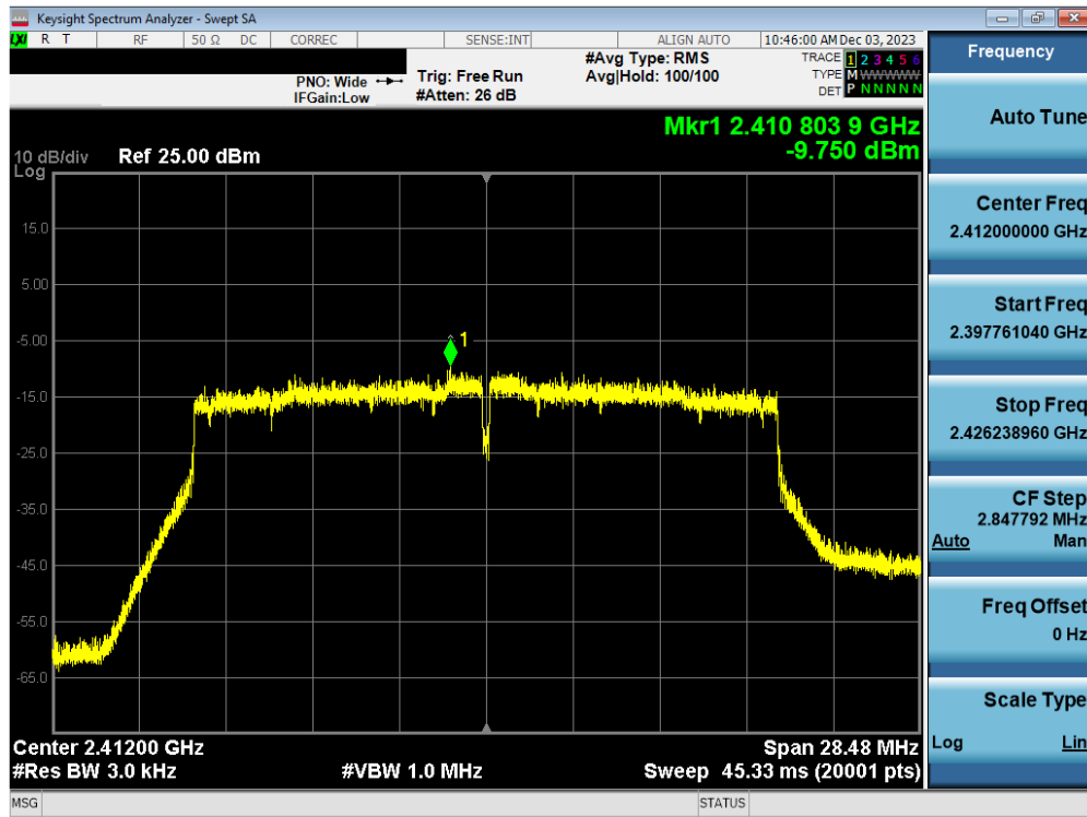
Plot 7-67. Power Spectral Density Plot Antenna WF7b (802.11ax(SU) - (2.4GHz) – Ch. 1) – MCS2
