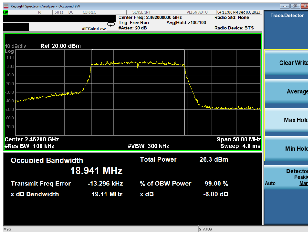
Plot 7-48. 6 dB BW and 99% OBW Plot Antenna WF2b (802.11ax(SU) - (2.4GHz) – Ch. 11) – MCS4
