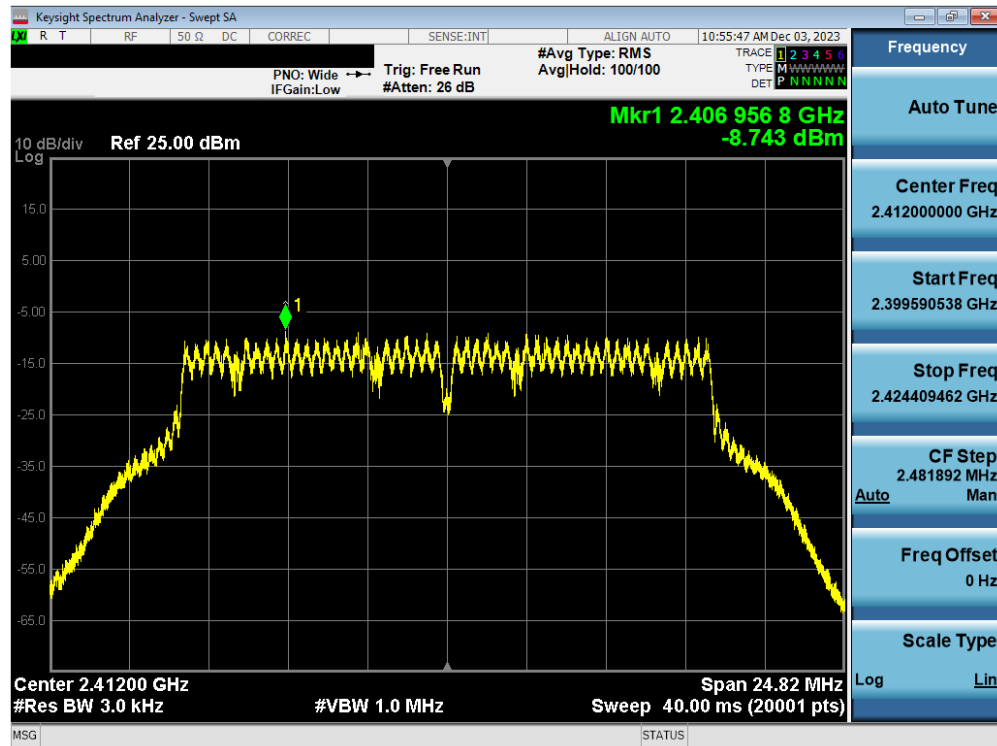
Plot 7-82. Power Spectral Density Plot Antenna WF7b (802.11g – Ch. 1) – 54Mbps
