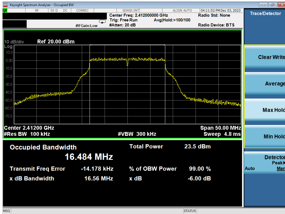
Plot 7-52. 6 dB BW and 99% OBW Plot Antenna WF2b (802.11g – Ch. 1) – 54Mbps
