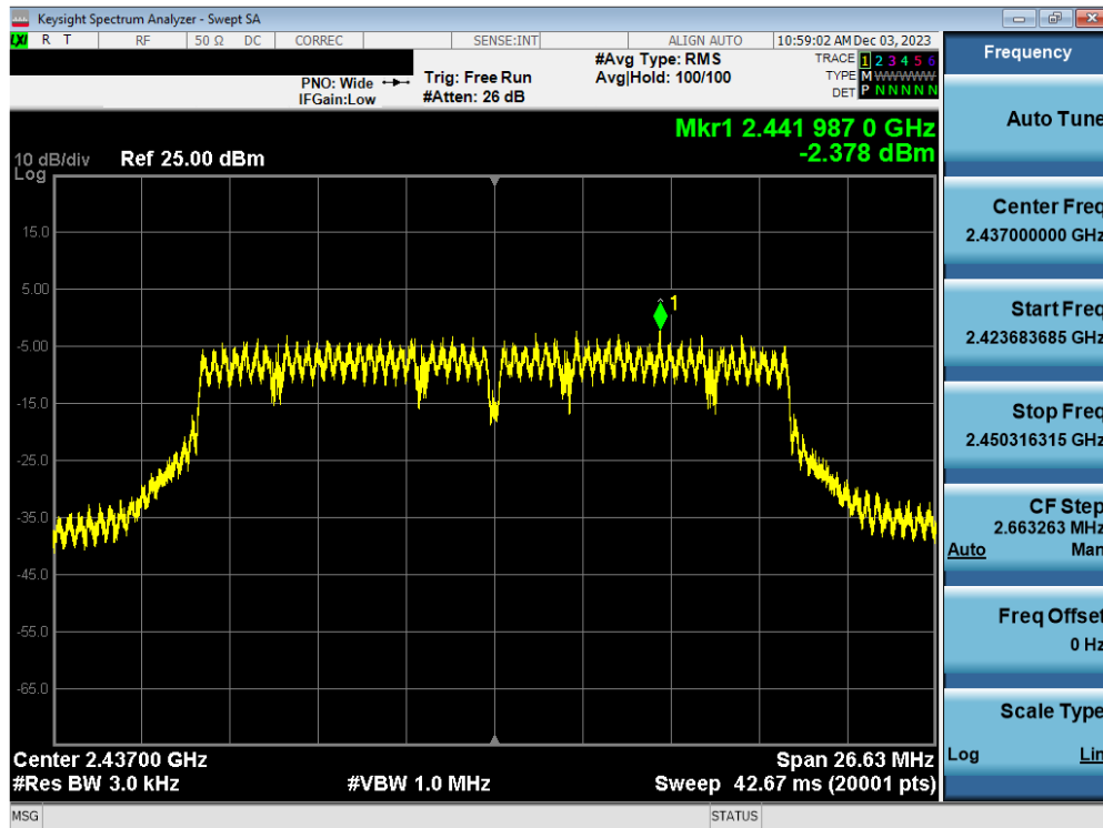
Plot 7-86. Power Spectral Density Plot Antenna WF7b (802.11n (2.4GHz) – Ch. 6) – MCS7
