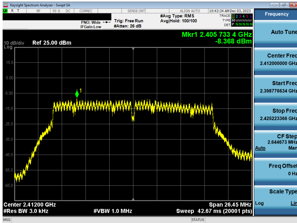
Plot 7-64. Power Spectral Density Plot Antenna WF7b (802.11n (2.4GHz) – Ch. 1) – MCS2
