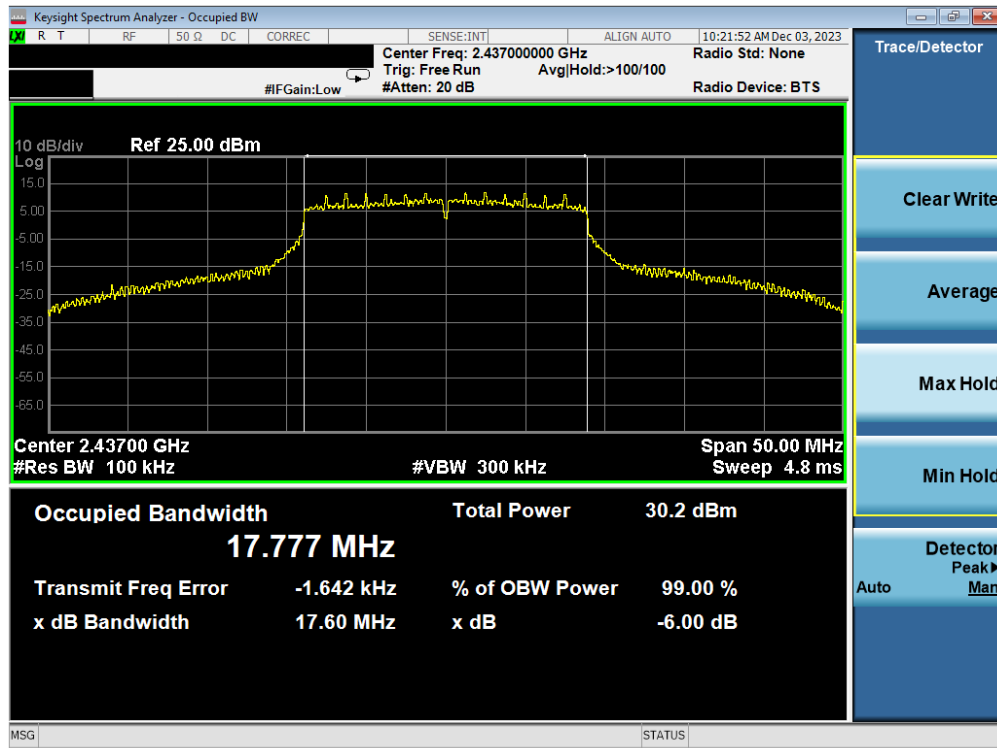
Plot 7-5. 6 dB BW and 99% OBW Plot Antenna WF7b (802.11n (2.4GHz) – Ch. 6) – MCS2
