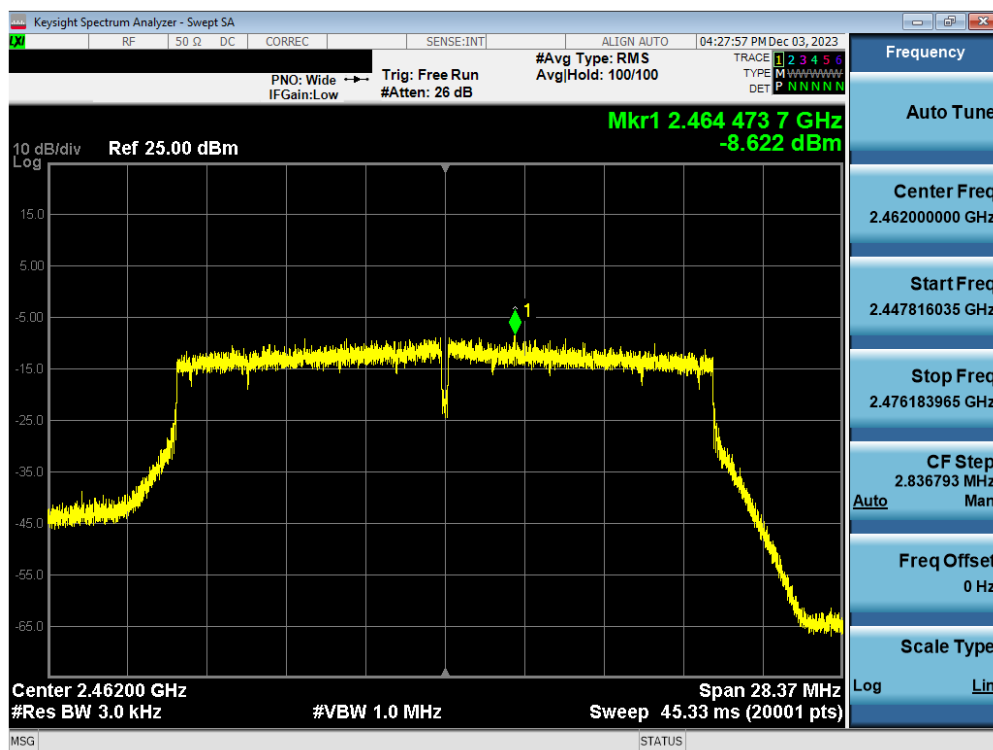
Plot 7-99. Power Spectral Density Plot Antenna WF2b (802.11ax(SU) - (2.4GHz) – Ch. 11) – MCS2
