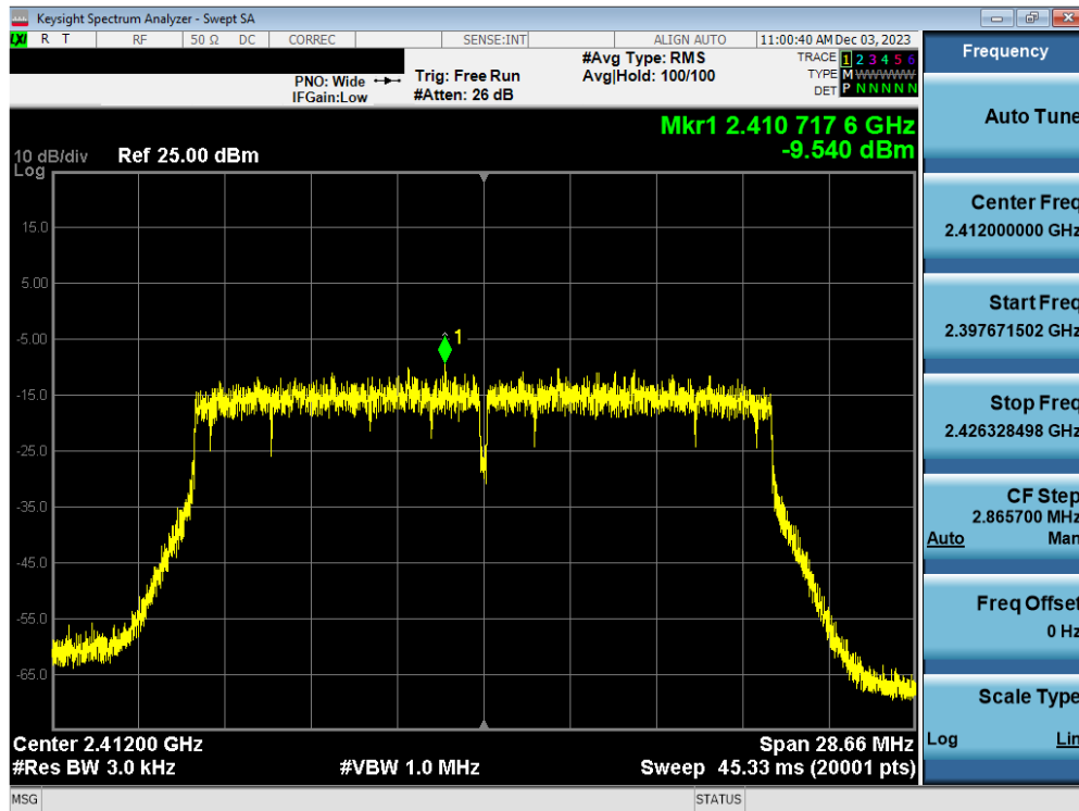
Plot 7-88. Power Spectral Density Plot Antenna WF7b (802.11ax(SU) - (2.4GHz) – Ch. 1) – MCS9
