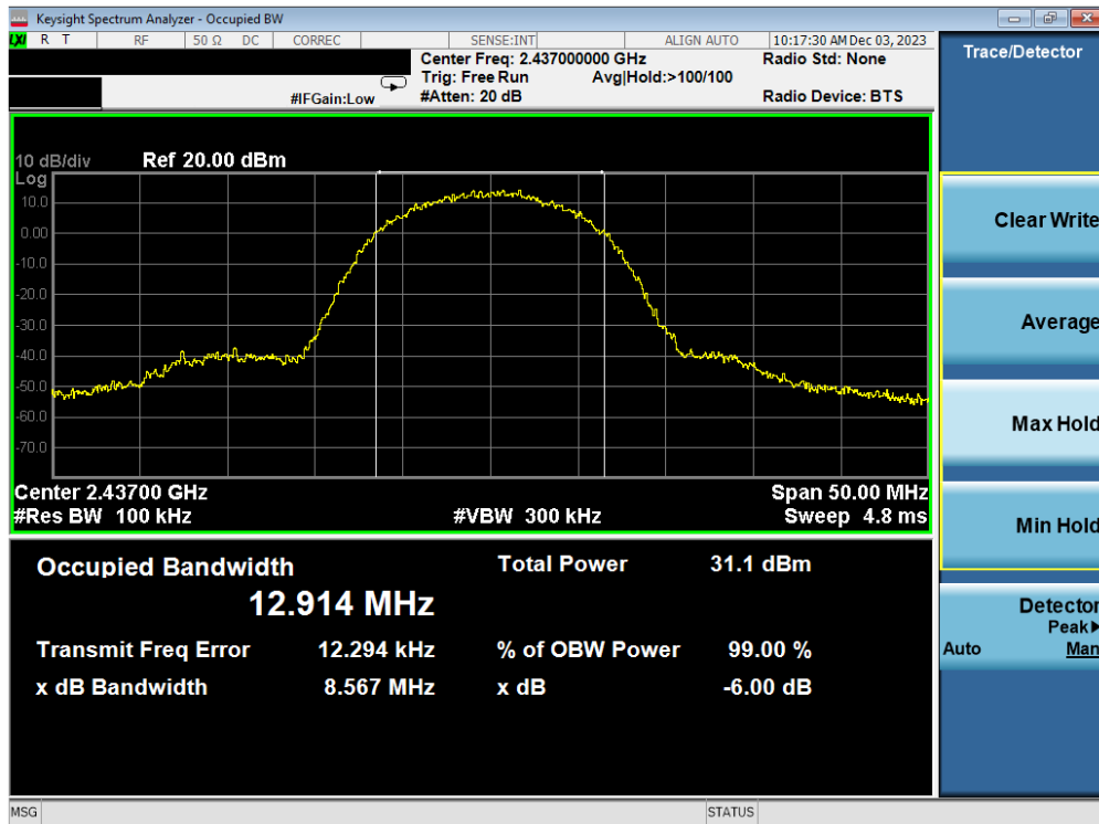
Plot 7-20. 6 dB BW and 99% OBW Plot Antenna WF7b (802.11b – Ch. 6) – 11Mbps
