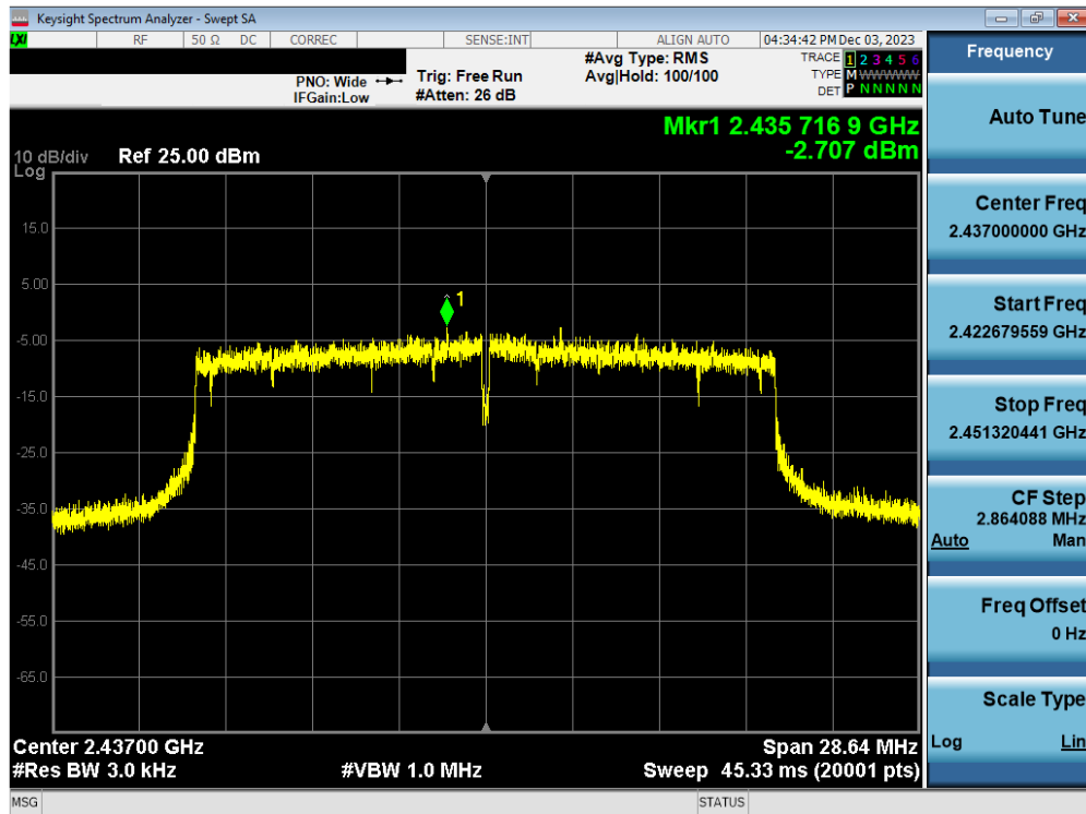
Plot 7-107. Power Spectral Density Plot Antenna WF2b (802.11ax(SU)) - (2.4GHz) – Ch. 6) – MCS4
