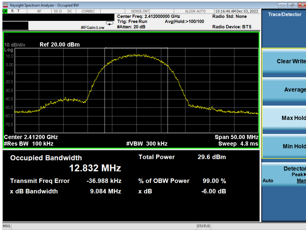
Plot 7-19. 6 dB BW and 99% OBW Plot Antenna WF7b (802.11b – Ch. 1) – 11Mbps
