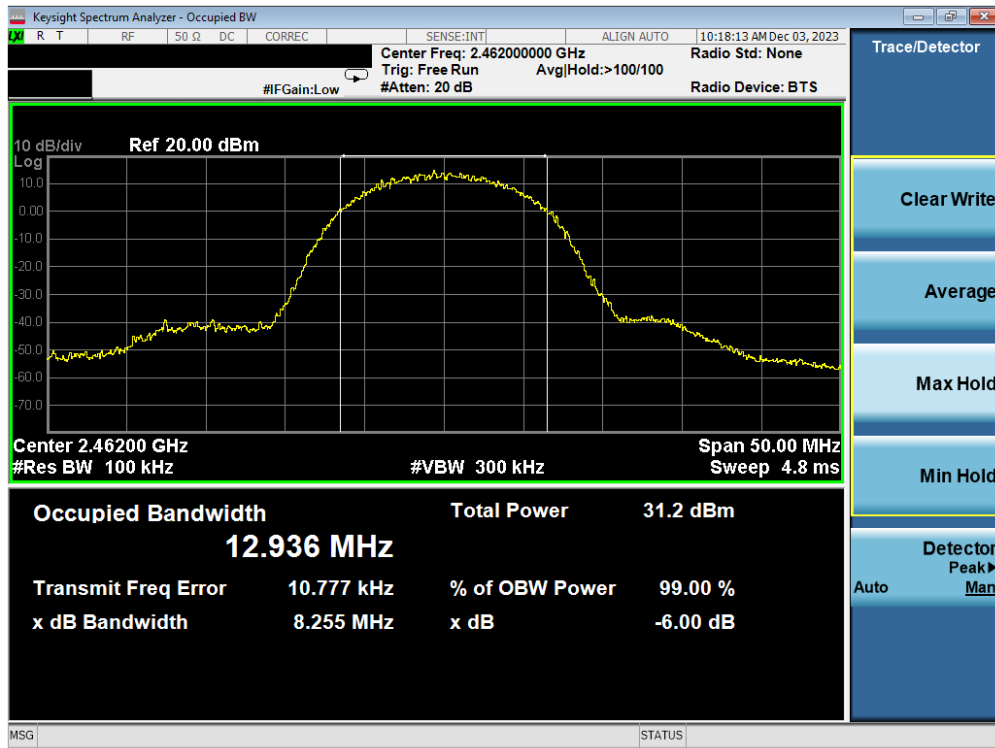
Plot 7-21. 6 dB BW and 99% OBW Plot Antenna WF7b (802.11b – Ch. 11) – 11Mbps
