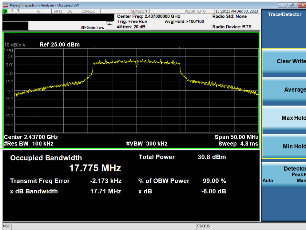
Plot 7-14. 6 dB BW and 99% OBW Plot Antenna WF7b (802.11n (2.4GHz) – Ch. 6) – MCS4
