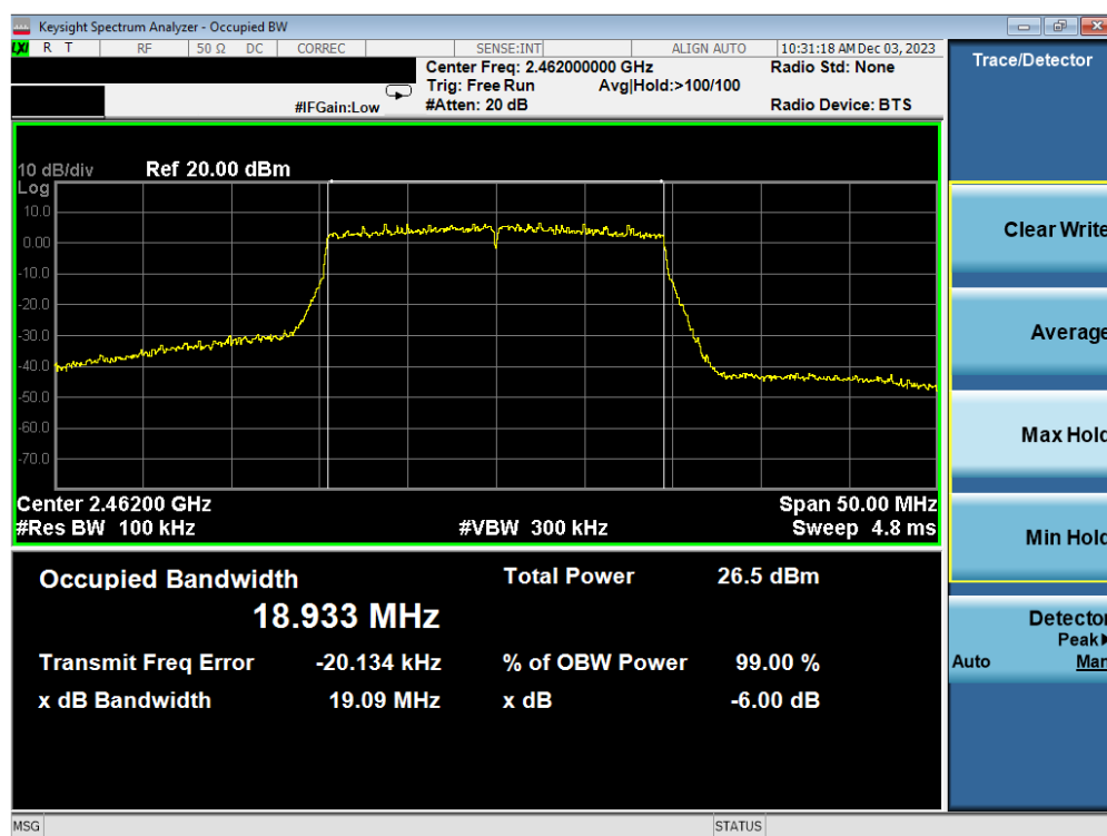
Plot 7-18. 6 dB BW and 99% OBW Plot Antenna WF7b (802.11ax(SU) - (2.4GHz) – Ch. 11) – MCS4
