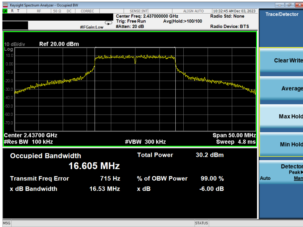
Plot 7-23. 6 dB BW and 99% OBW Plot Antenna WF7b (802.11g – Ch. 6) – 54Mbps
