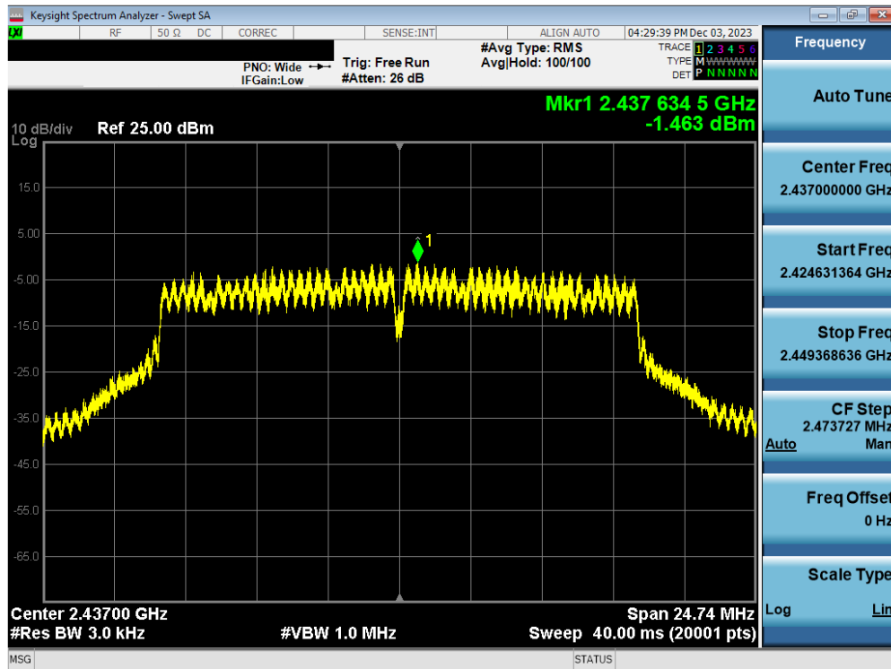
Plot 7-101. Power Spectral Density Plot Antenna WF2b (802.11g – Ch. 6) – 24Mbps
