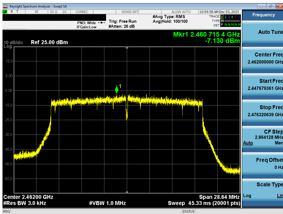
Plot 7-78. Power Spectral Density Plot Antenna WF7b (802.11ax(SU) - (2.4GHz) – Ch. 11) – MCS4
