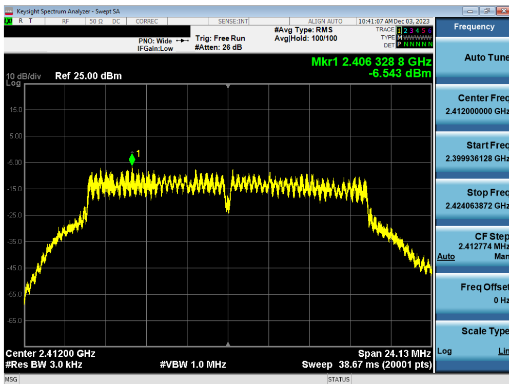
Plot 7-61. Power Spectral Density Plot Antenna WF7b (802.11g – Ch. 1) – 12Mbps
