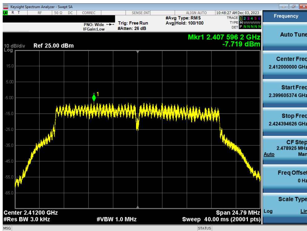
Plot 7-70. Power Spectral Density Plot Antenna WF7b (802.11g – Ch. 1) – 24Mbps
