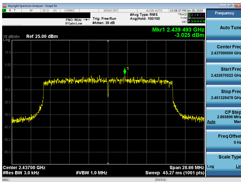
Plot 7-89. Power Spectral Density Plot Antenna WF7b (802.11ax(SU) - (2.4GHz) – Ch. 6) – MCS9
