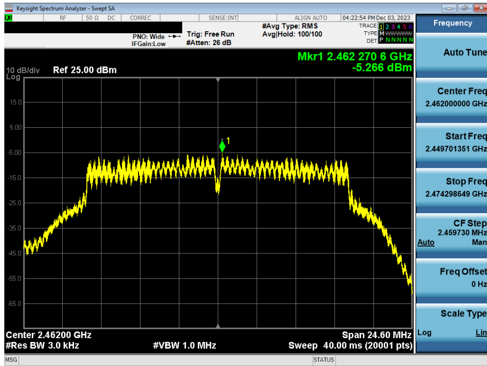
Plot 7-93. Power Spectral Density Plot Antenna WF2b (802.11g – Ch. 11) – 12Mbps
