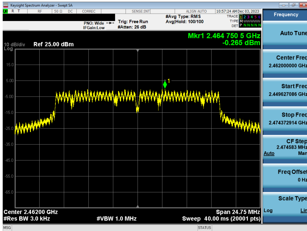
Plot 7-84. Power Spectral Density Plot Antenna WF7b (802.11g – Ch. 11) – 54Mbps
