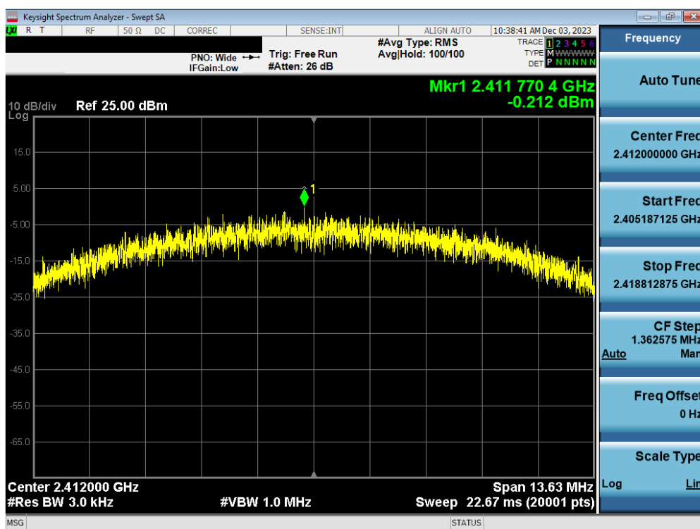
Plot 7-79. Power Spectral Density Plot Antenna WF7b (802.11b – Ch. 1) – 11Mbps
