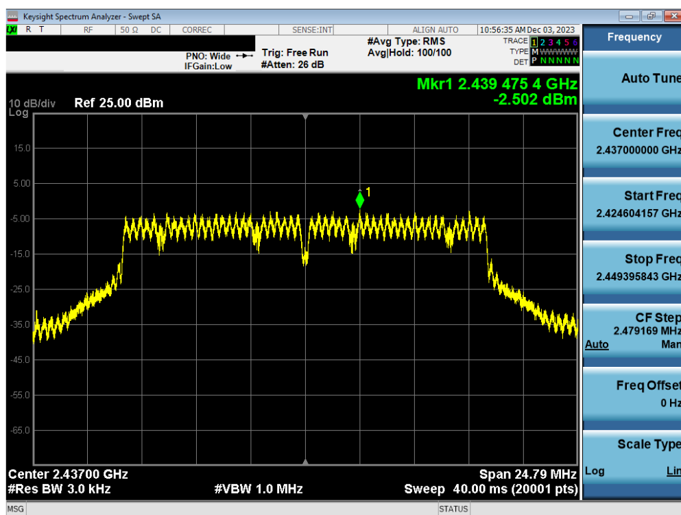
Plot 7-83. Power Spectral Density Plot Antenna WF7b (802.11g – Ch. 6) – 54Mbps
