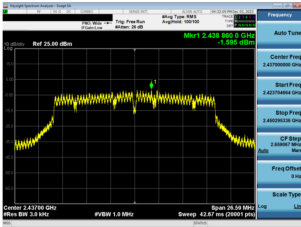
Plot 7-104. Power Spectral Density Plot Antenna WF2b (802.11n (2.4GHz) – Ch. 6) – MCS4
