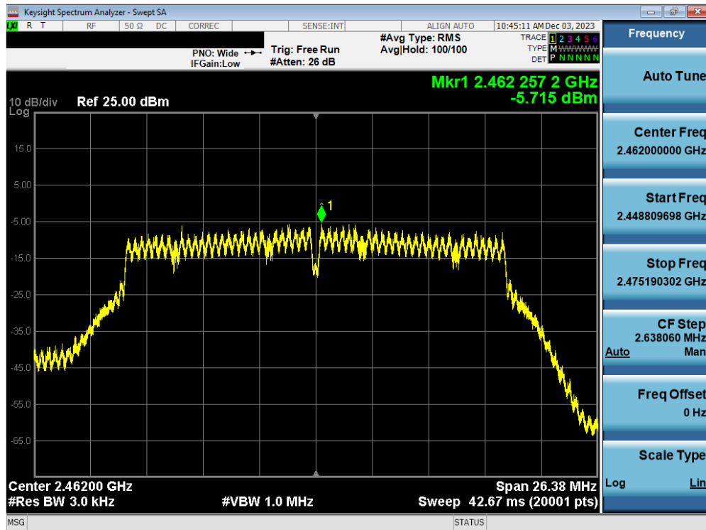
Plot 7-66. Power Spectral Density Plot Antenna WF7b (802.11n (2.4GHz) – Ch. 11) – MCS2
