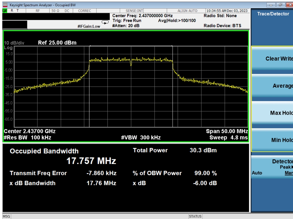
Plot 7-26. 6 dB BW and 99% OBW Plot Antenna WF7b (802.11n (2.4GHz) – Ch. 6) – MCS7
