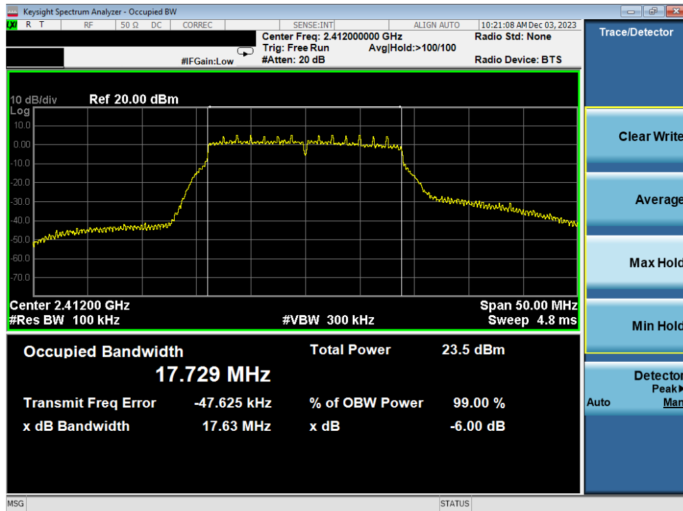
Plot 7-4. 6 dB BW and 99% OBW Plot Antenna WF7b (802.11n (2.4GHz) – Ch. 1) – MCS2
