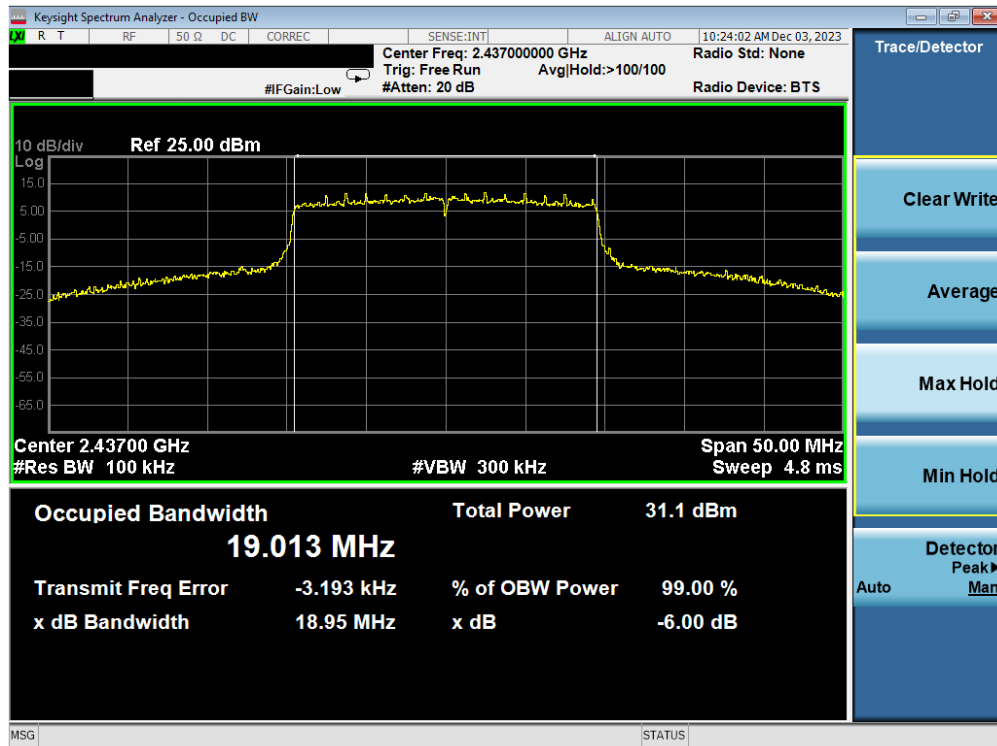
Plot 7-8. 6 dB BW and 99% OBW Plot Antenna WF7b (802.11ax(SU) - (2.4GHz) – Ch. 6) – MCS2
