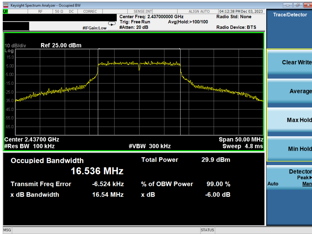
Plot 7-53. 6 dB BW and 99% OBW Plot Antenna WF2b (802.11g – Ch. 6) – 54Mbps
