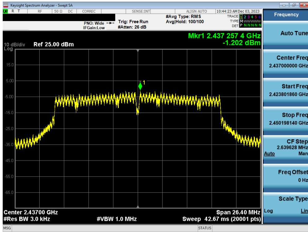
Plot 7-65. Power Spectral Density Plot Antenna WF7b (802.11n (2.4GHz) – Ch. 6) – MCS2
