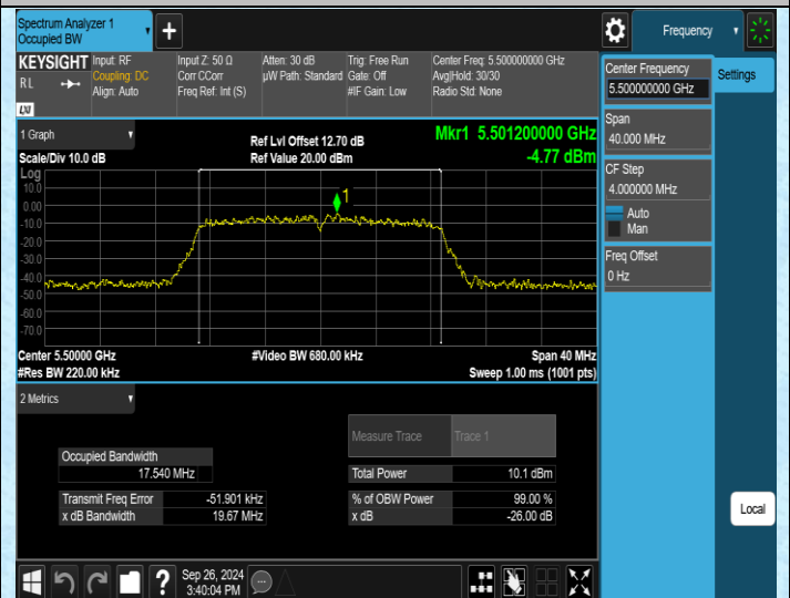
11AC20MIMO-Ant2-5500
