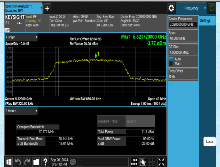
11AC20MIMO-Ant2-5320
