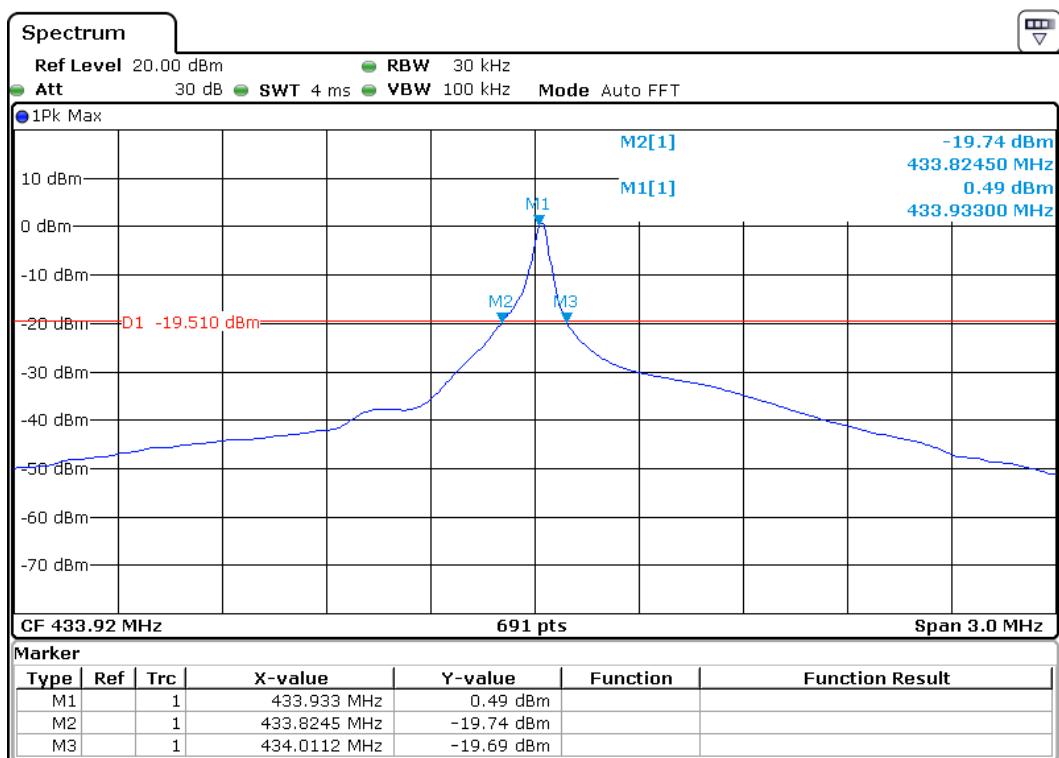
Channel 01: 433.92MHz
