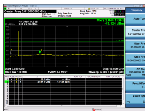
B13-5M-Mid CH-CSE-1-QPSK-1 RB 0
