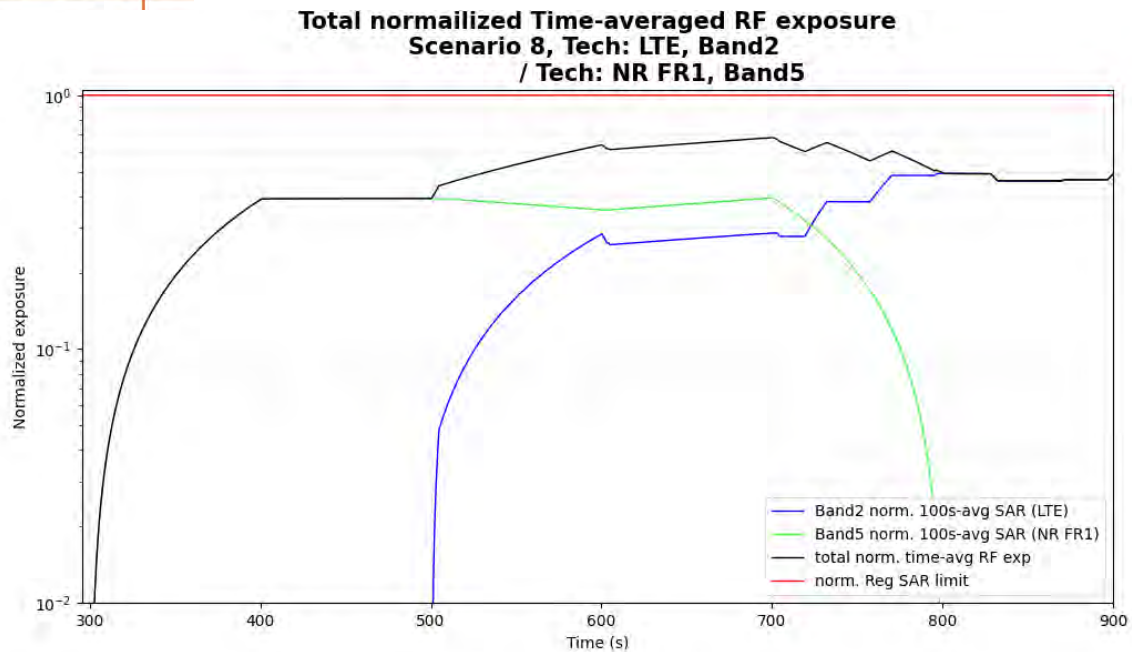
Figure 5- 57 Normalized time-averaged SAR for case 23 (LTE B2, sub6 NR n5)
