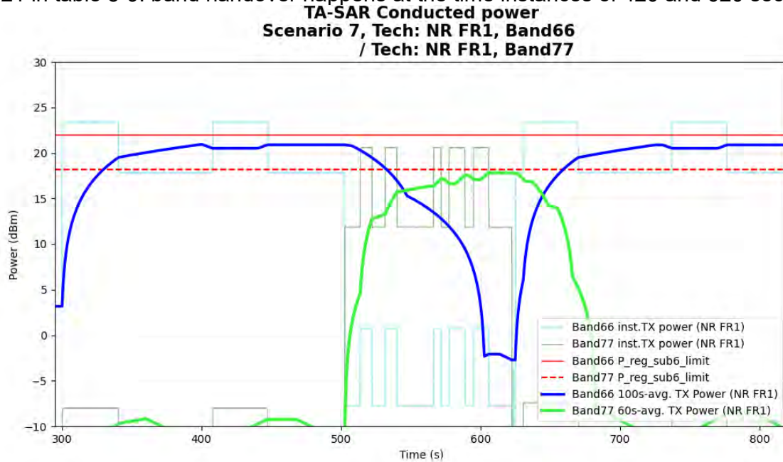
Figure 5- 52 Time-averaged conducted TX power over time for case 21 (sub6 NR n66 and n77)
