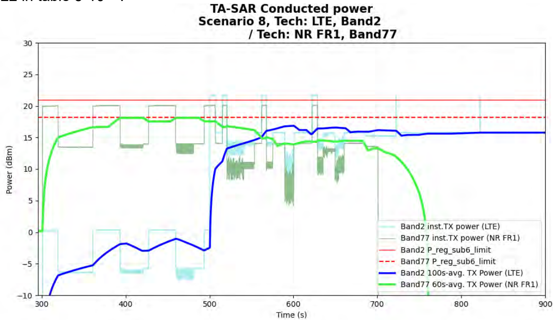
Figure 5- 54 Time-averaged conducted TX power over time for case 22 (LTE B2, sub6 NR n77)
