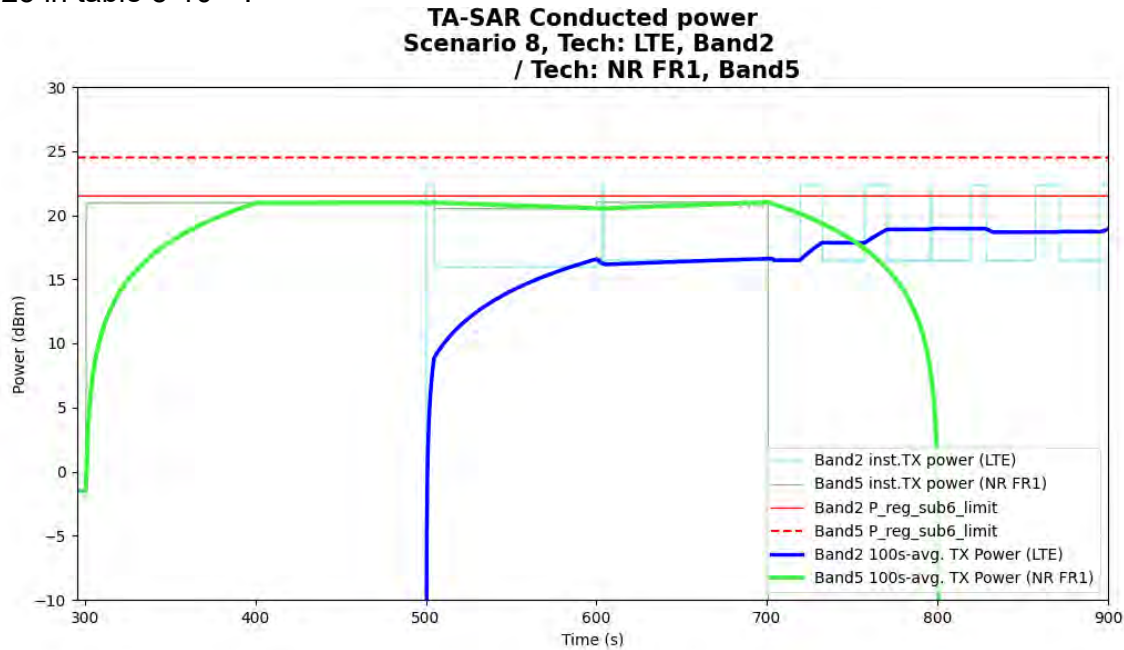
Figure 5- 56 Time-averaged conducted TX power over time for case 23 (LTE B2, sub6 NR n5)
