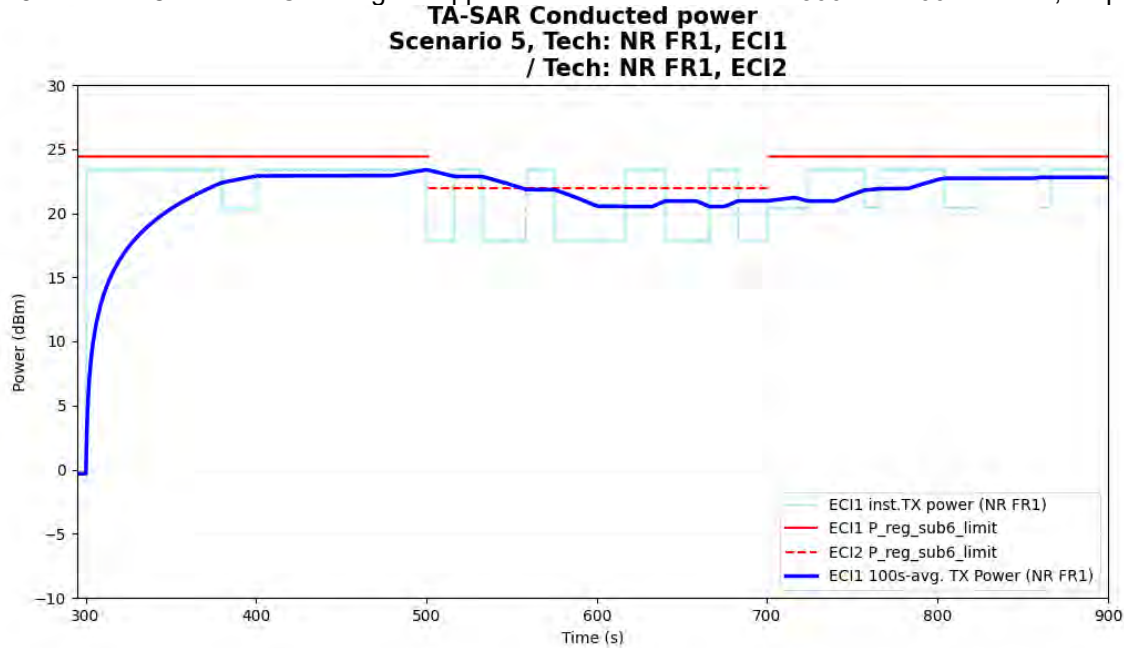
Figure 5- 46 Time-averaged conducted TX power over time for case 19 (sub NR n66)
