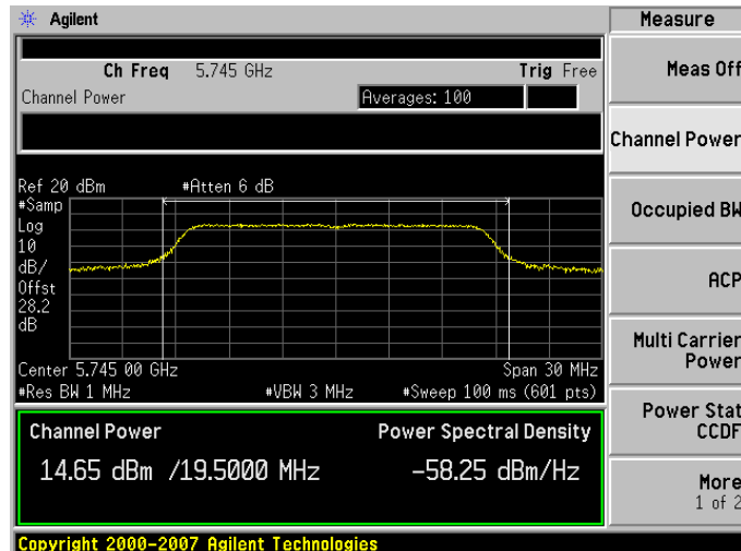
Antenna D
