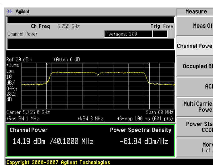
Antenna D
