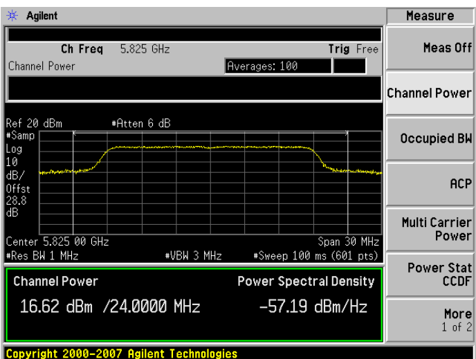
Antenna D
