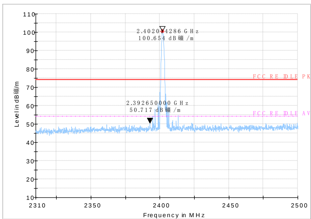
Fig.53 Radiated emission (Power): 8DPSK, low channel
