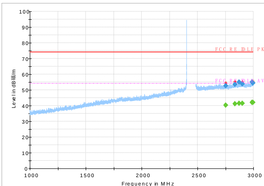
Fig.46 Radiated emission: \pi/4 DQPSK, Ch0, 1GHz~3GHz
