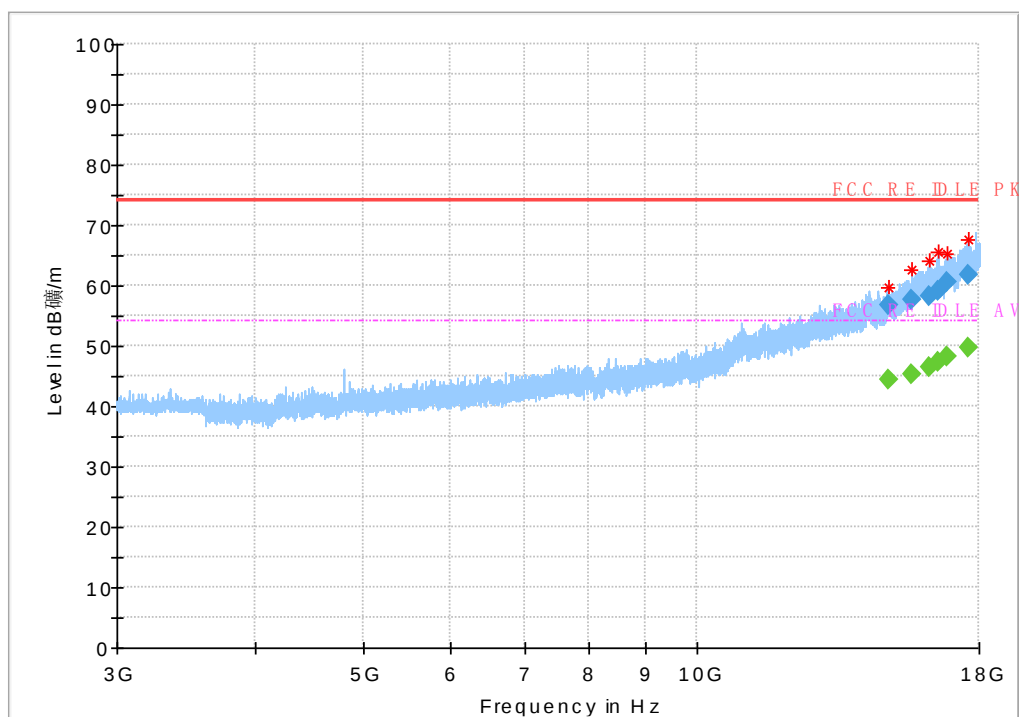
Fig.52 Radiated emission: 8DPSK, Ch0, 3GHz~18GHz
