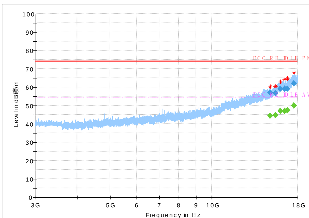
Fig.47 Radiated emission: \pi/4 DQPSK, Ch0, 3GHz~18GHz
