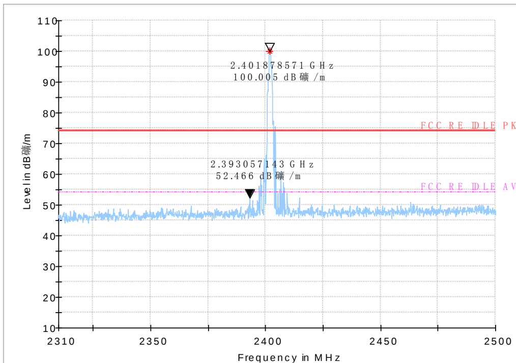
Fig.48 Radiated emission (Power): \pi/4 DQPSK, low channel
