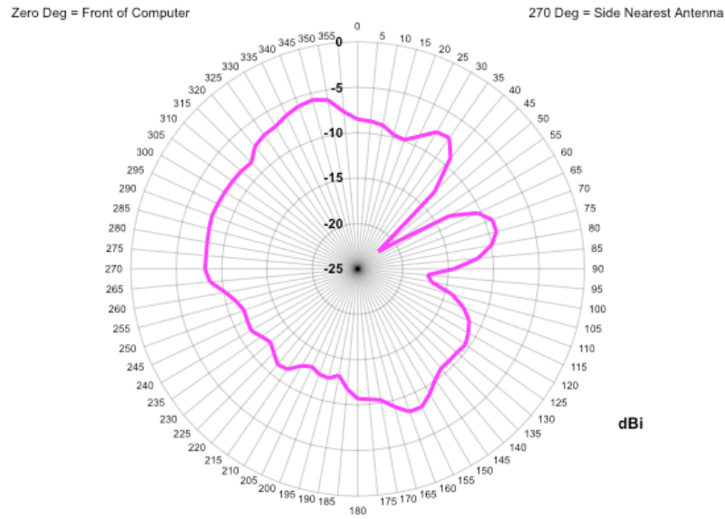
603-1203 Radiation Pattern; Azimuth; 2.45 GHz
