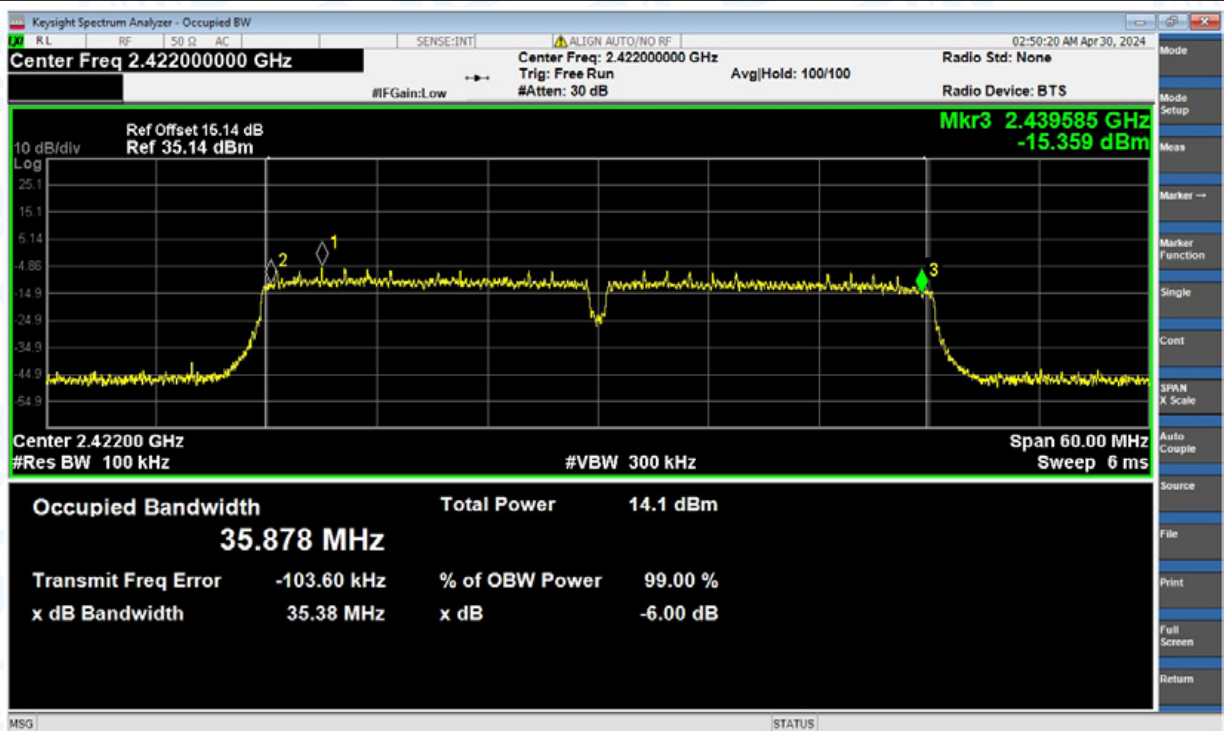
-6dB Bandwidth NVNT n(HT40) 2422MHz Ant2
