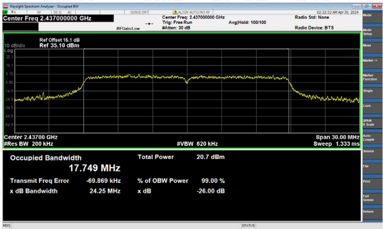
OBW NVNT n(HT20) 2437MHz Ant2
