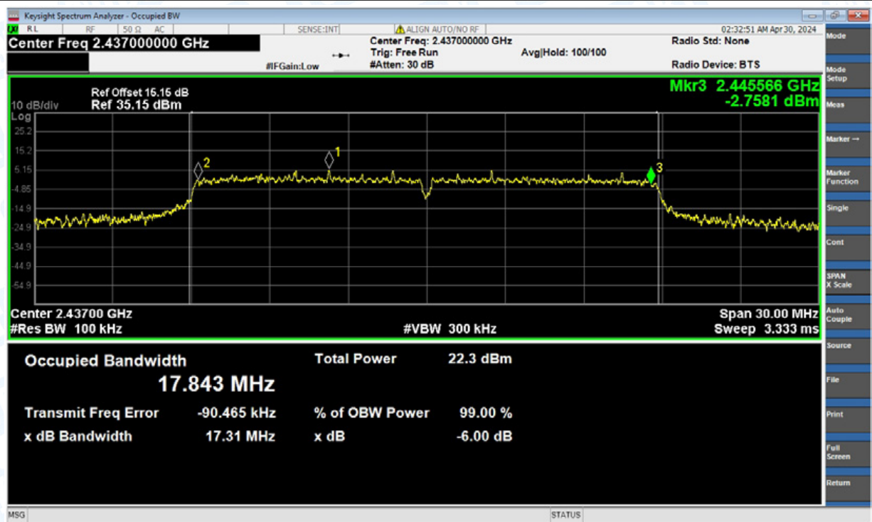
-6dB Bandwidth NVNT n(HT20) 2437MHz Ant2
