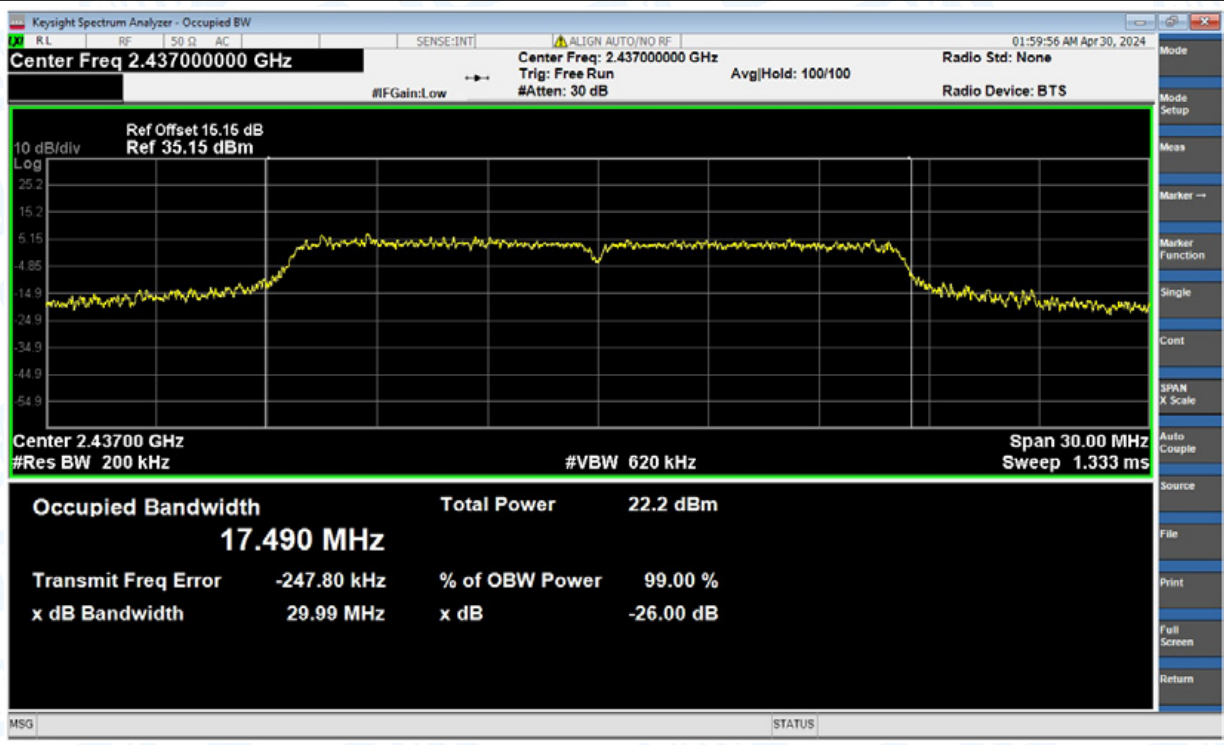
OBW NVNT g 2437MHz Ant2
