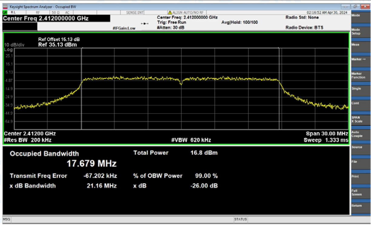
OBW NVNT n(HT20) 2412MHz Ant2
