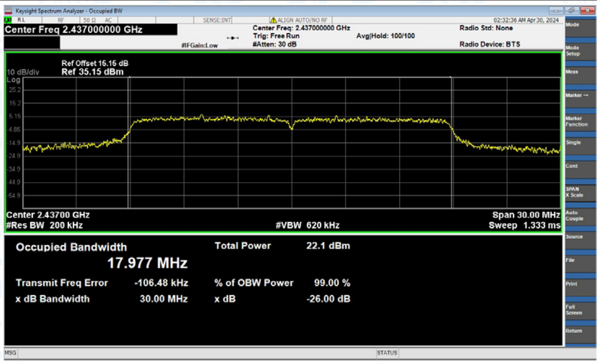
OBW NVNT n(HT20) 2437MHz Ant2
