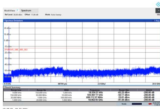
NB-IoT Band 12 CH-Middle 9kHz~20GHz
