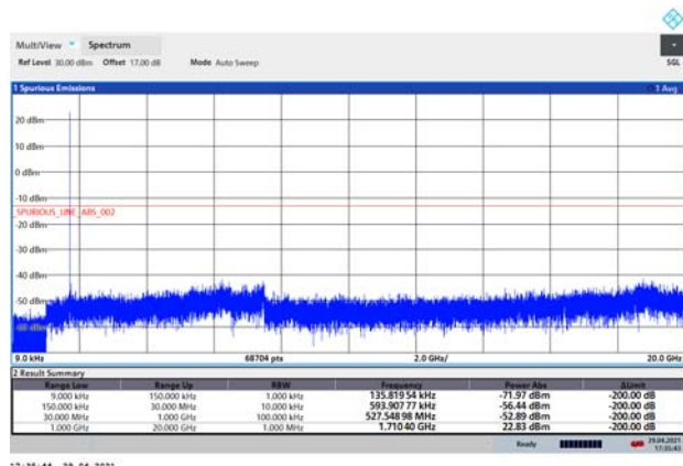
NB-IoT Band 4 CH-Middle 9kHz~20GHz
