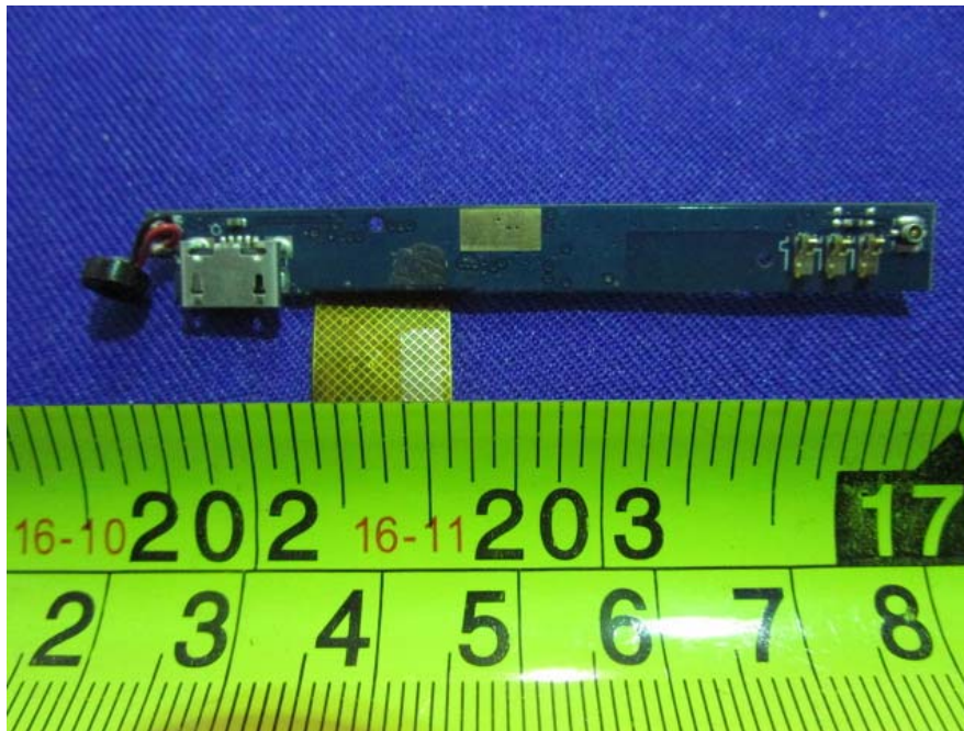
EUT – PC Board Top View
