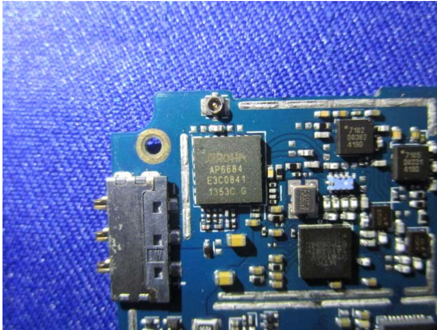
EUT – GSM Chipset 1 View
