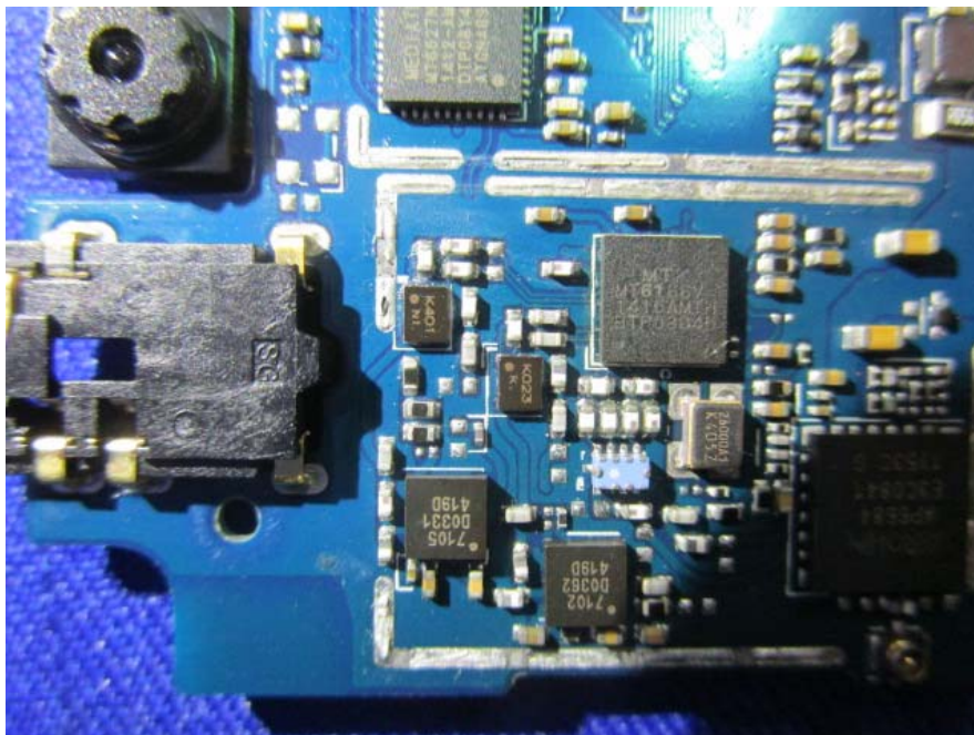
EUT –GSM Chipset 2 View
