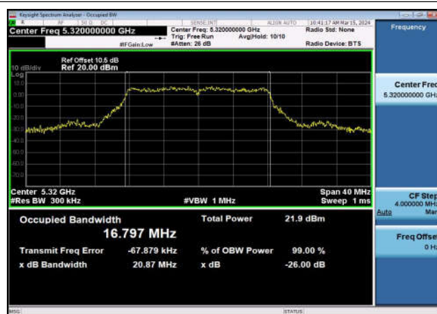
U-NII-2a 99%&26dB Bandwidth-802.11a(20MHz) ,5320MHz,Ant1
