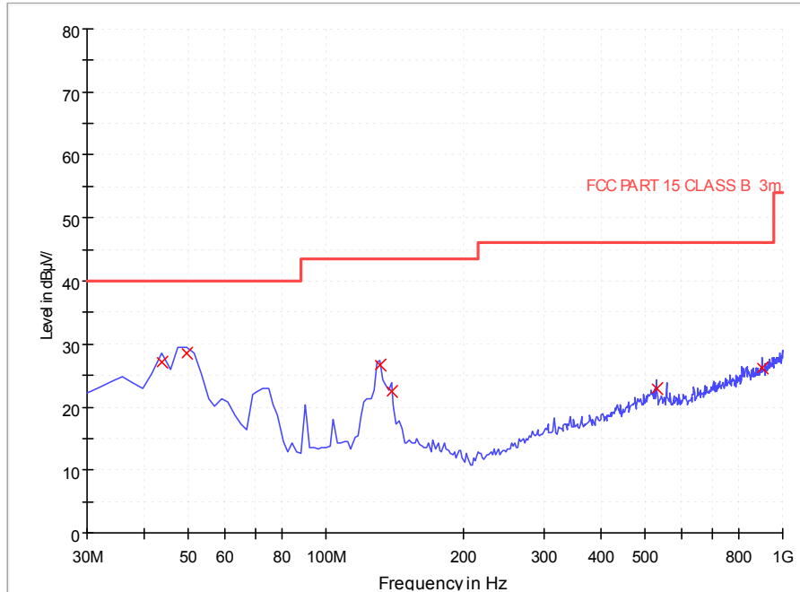
EMI Sweep-3M(30-1G)
