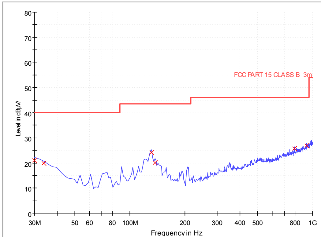
EMI Sweep-3M(30-1G)
