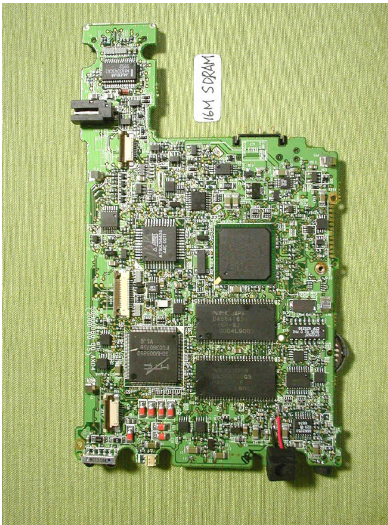
Front view of SDRAM (16MB)
