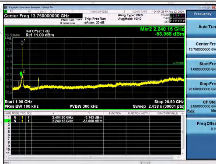
11AX40SISO-Ant1-2422-1000~26500-PASS
