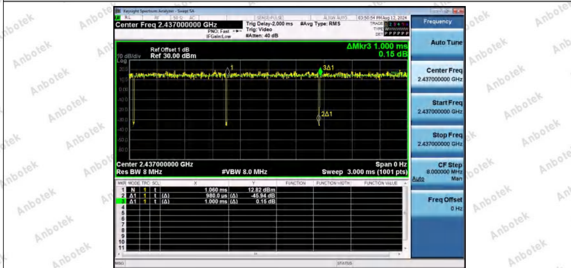
NTNV-11AX20SISO-Ant1-2437
