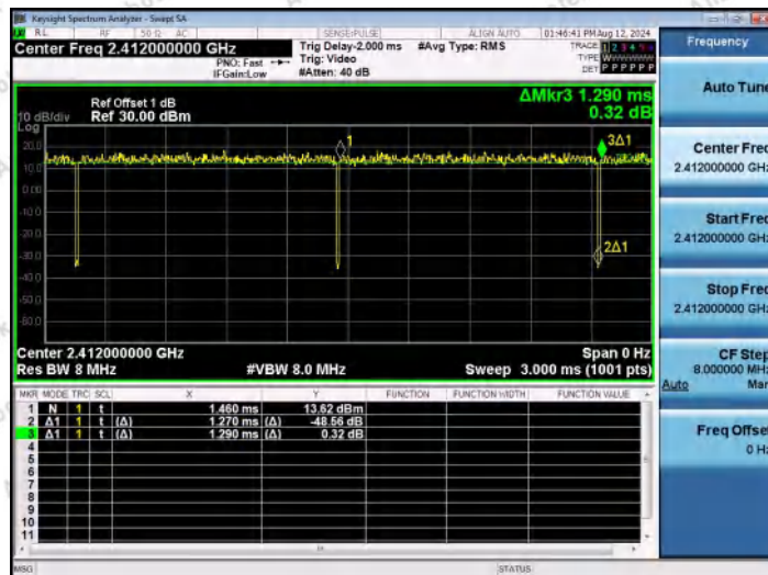
NTNV-11N20SISO-Ant1-2412
