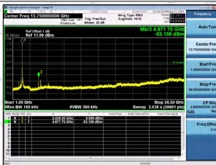
11G-Ant1-2437-1000~26500-PASS
