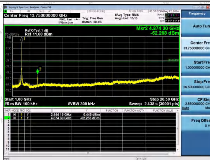
11AX20SISO-Ant1-2437-1000~26500-PASS
