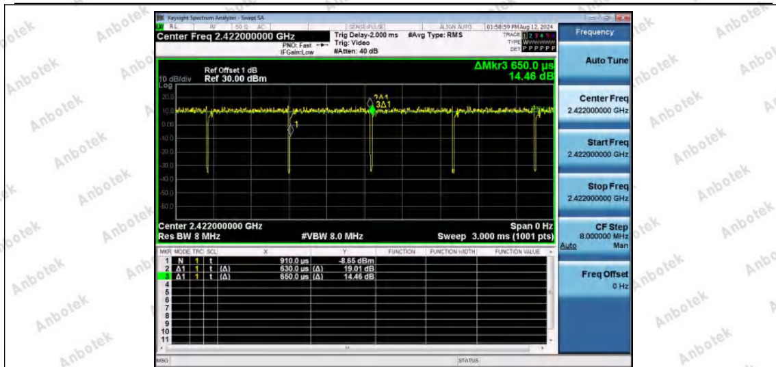
NTNV-11N40SISO-Ant1-2422
