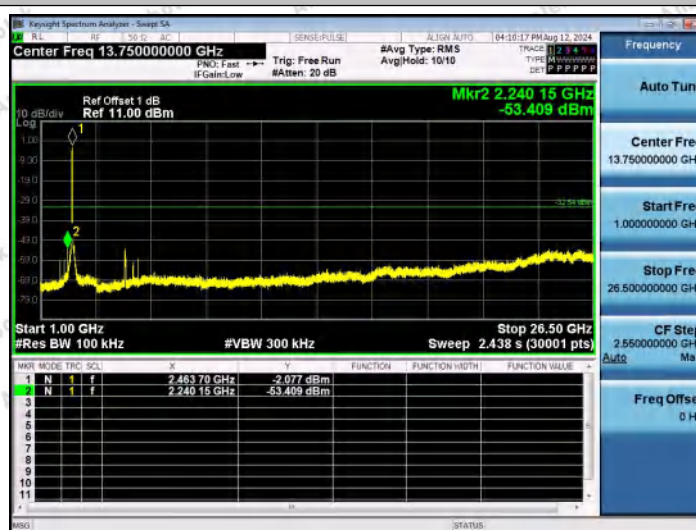
11AX40SISO-Ant1-2452-1000~26500-PASS
