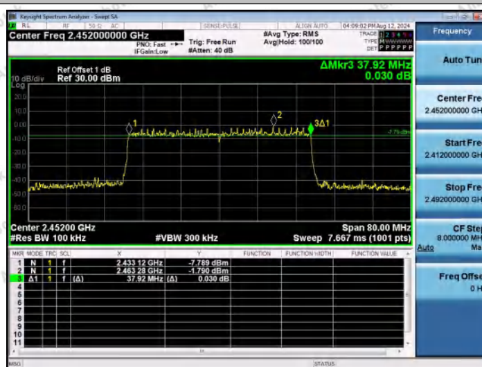
11AX40SISO-Ant1-2452-PASS
