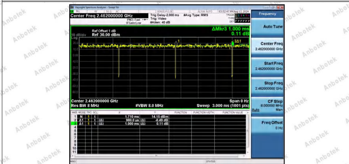
NTNV-11AX20SISO-Ant1-2462
