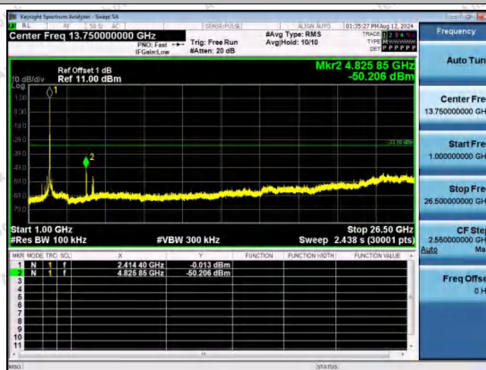
11G-Ant1-2412-1000~26500-PASS
