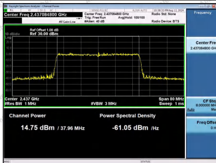
11AX40SISO-Ant1-2437-PASS
