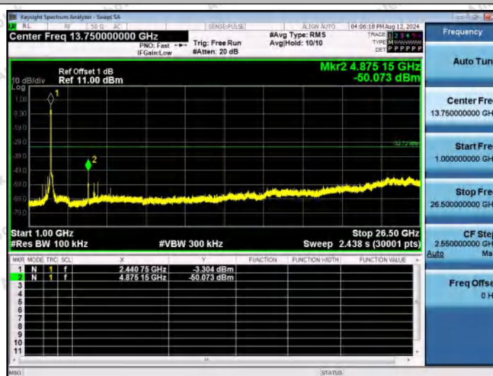
11AX40SISO-Ant1-2437-1000~26500-PASS
