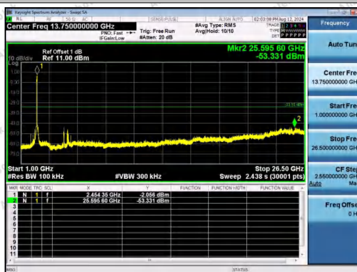
11N40SISO-Ant1-2437-1000~26500-PASS
