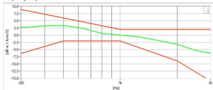
Frequency Response
