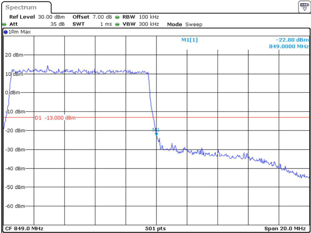
Band 5_10 MHz_High_QPSK_RB50#0
