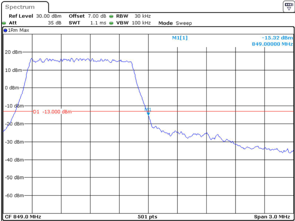
Band 5_1.4 MHz_High_QPSK_RB6#0
