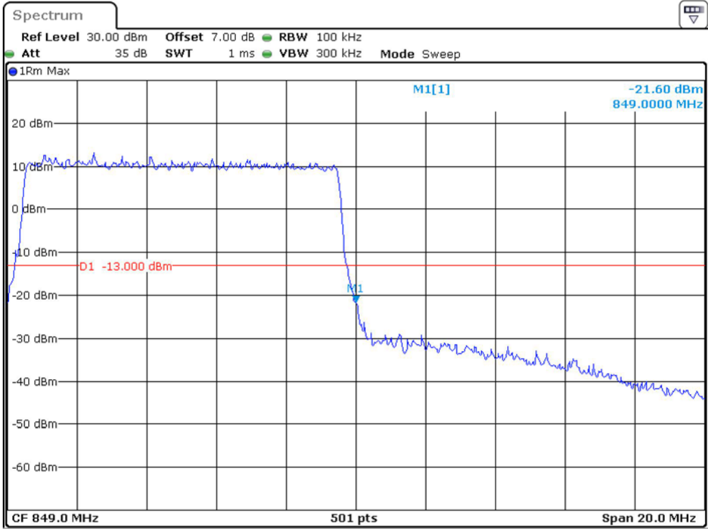
Band 5_10 MHz_High_16QAM_RB50#0
