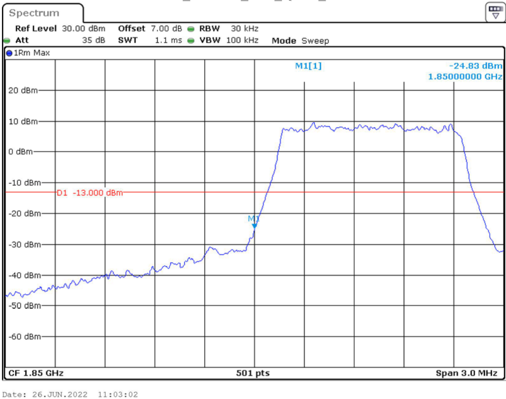
Band 2_1.4 MHz_Low_QPSK_RB6#0
