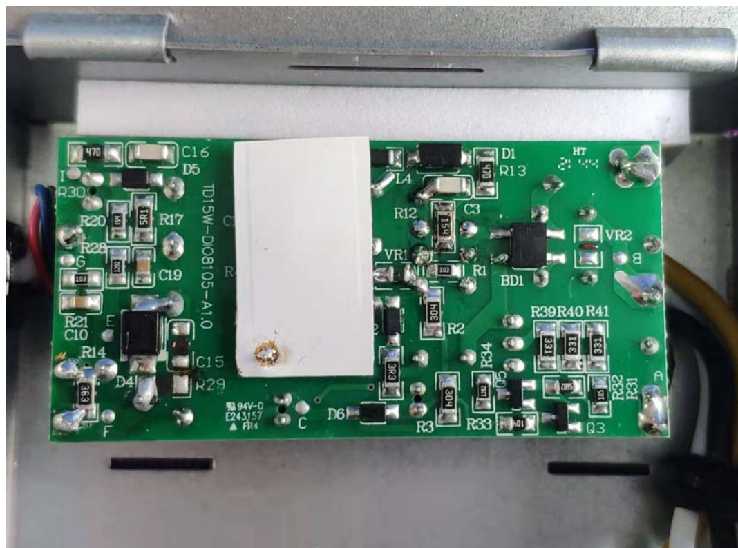
FIGURE 5 CYNCR FIXTURE CANLESS (M/N: CFIxCNLR6S1) POWER BOARD (COMPONENT SIDE)
