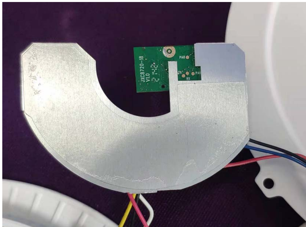
FIGURE 3 CYNC FIXTURE CANLESS (M/N: CFIXCNLR6S1) MAIN BOARD (SOLDERED SIDE)
