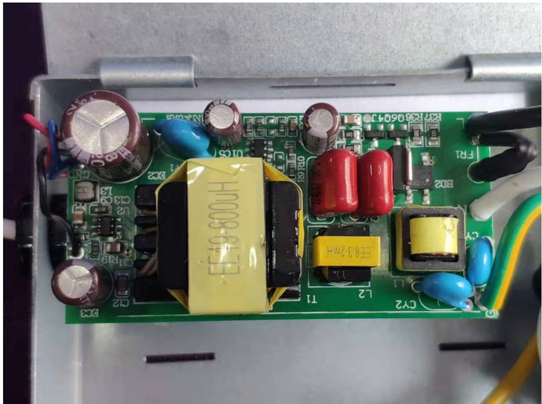
FIGURE 7 CYNC FIXTURE CANLESS (M/N: CFIXCNLR6S1) COVER REMOVED #2
