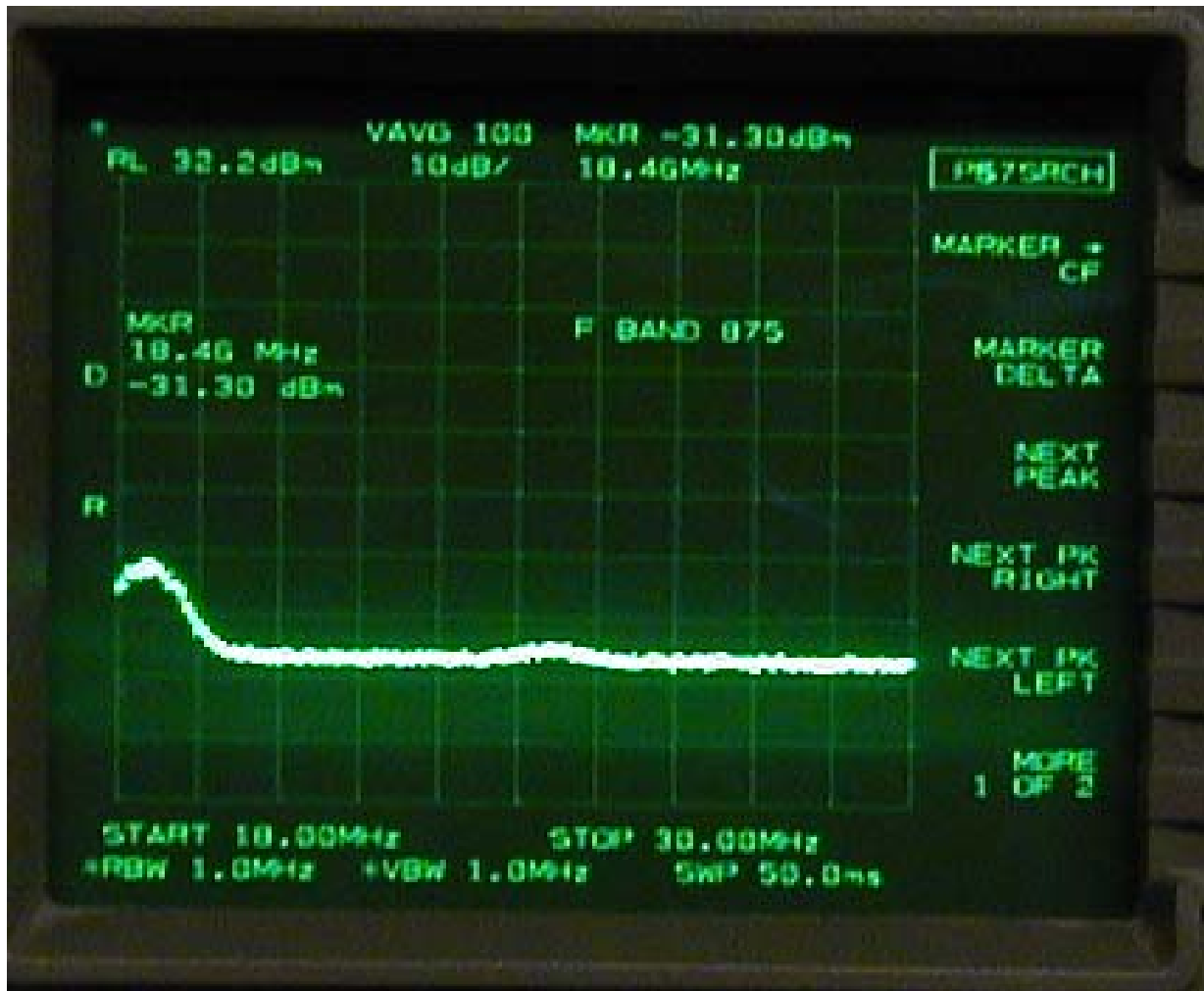
Figure 64: 18 MHz – 30 MHz
