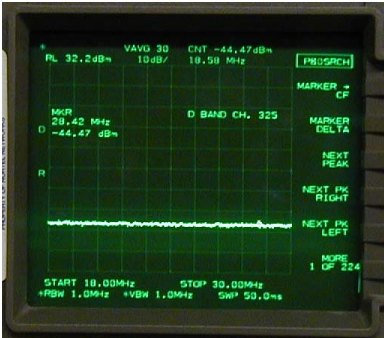
Figure 15 : 18 MHz – 30 MHz
