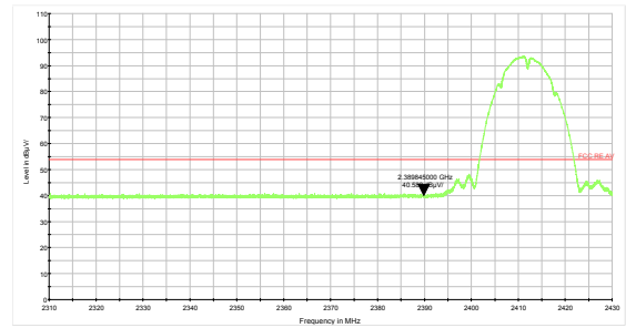
802.11b-Channel 1 Average
