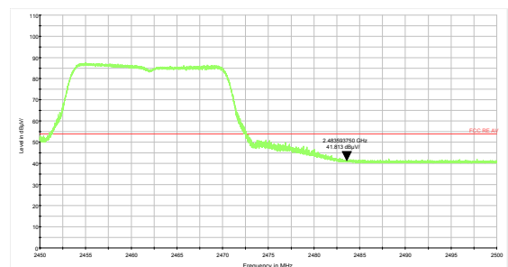
802.11g-Channel 11 Average
