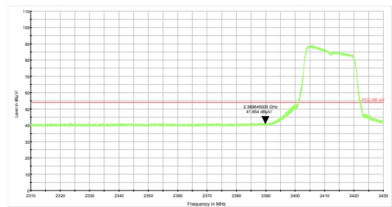
802.11g-Channel 1 Average
