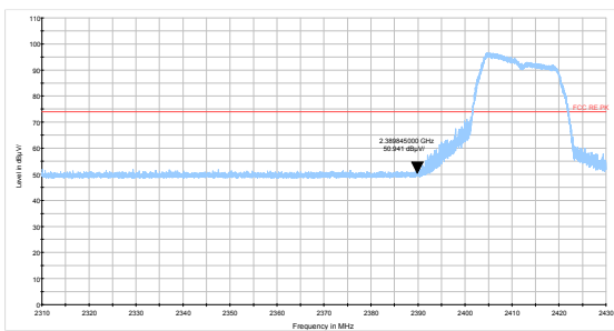
802.11g-Channel 1 Peak
