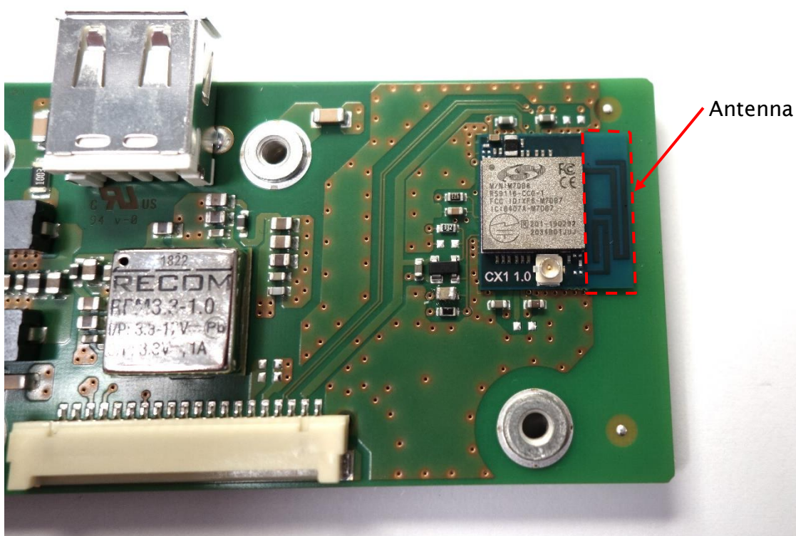
Detail of PCBA Redpine WLAN Module zoomed on RS9116N-DB00-CC1-B00
