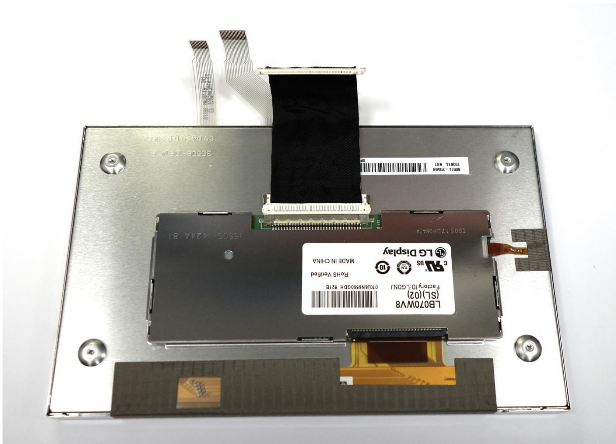
Back of AI Modul UL Display (without head spreader)
